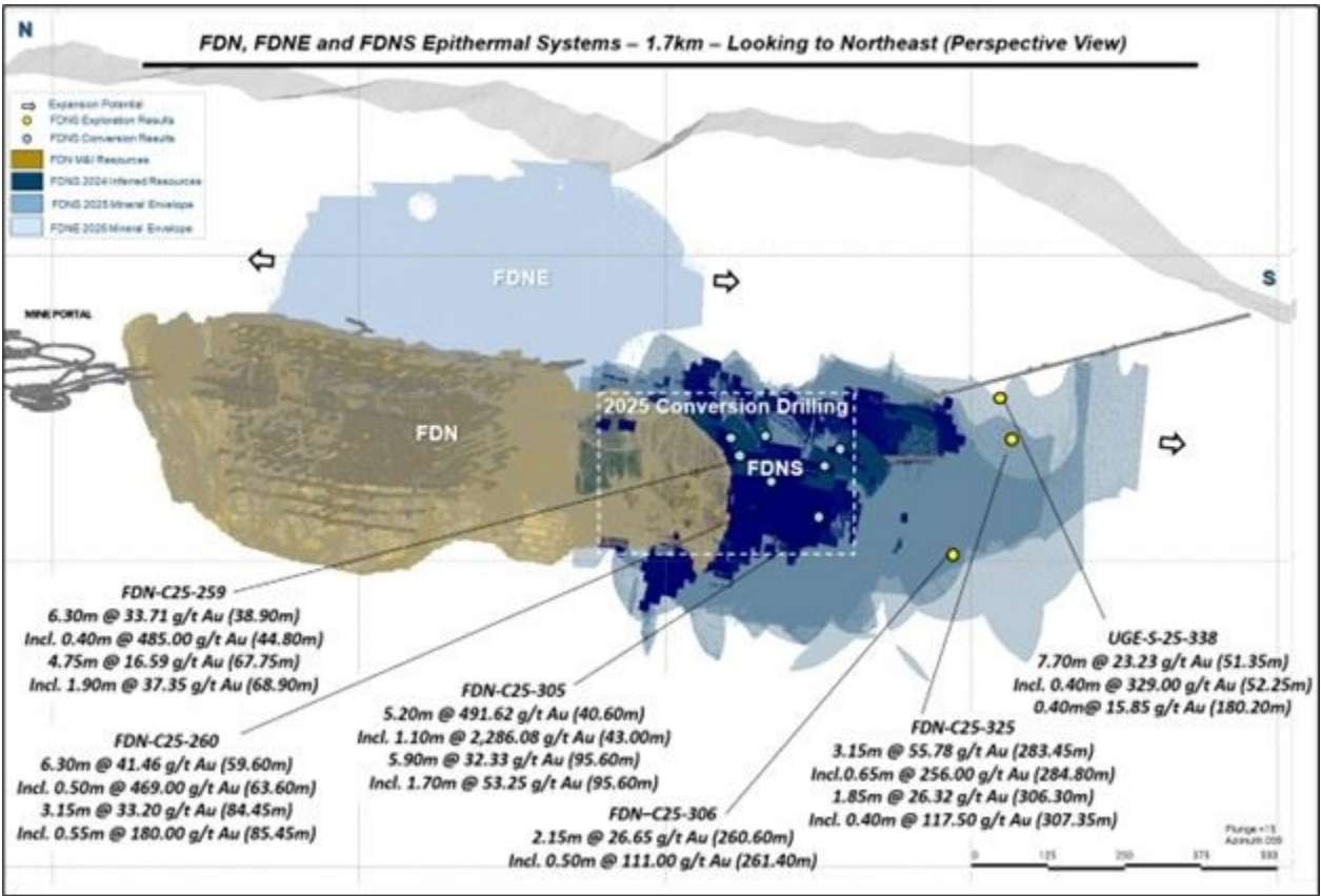
Figure 2: Map showing FDN and FDNS deposit with selected FDNS conversion and exploration drilling results
