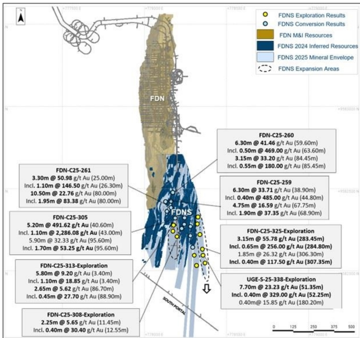
Figure 3: Map showing FDN, FDN deposit and FDN East with selected FDN East drilling results
