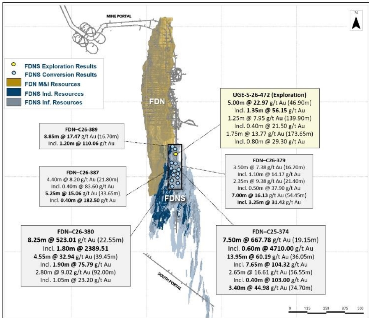
Figure 3: Long section showing FDN and FDNS deposits with selected FDNS conversion and exploration drilling results
