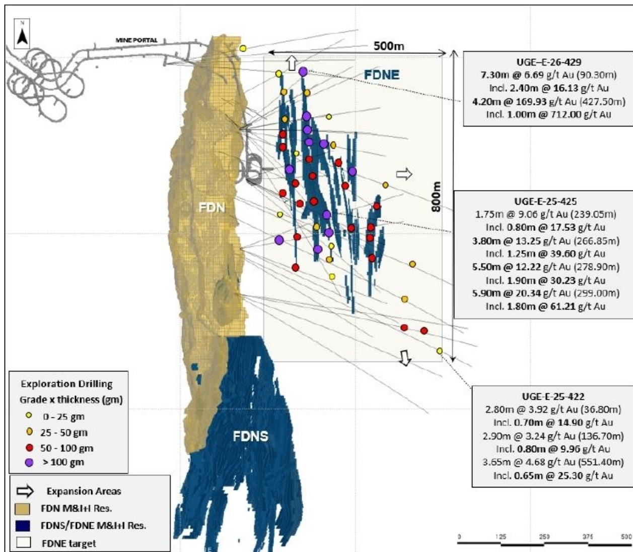
Figure 5: Long Section showing FDN, FDNS, FDN East deposits with selected exploration drilling results along the FDN upper extension
