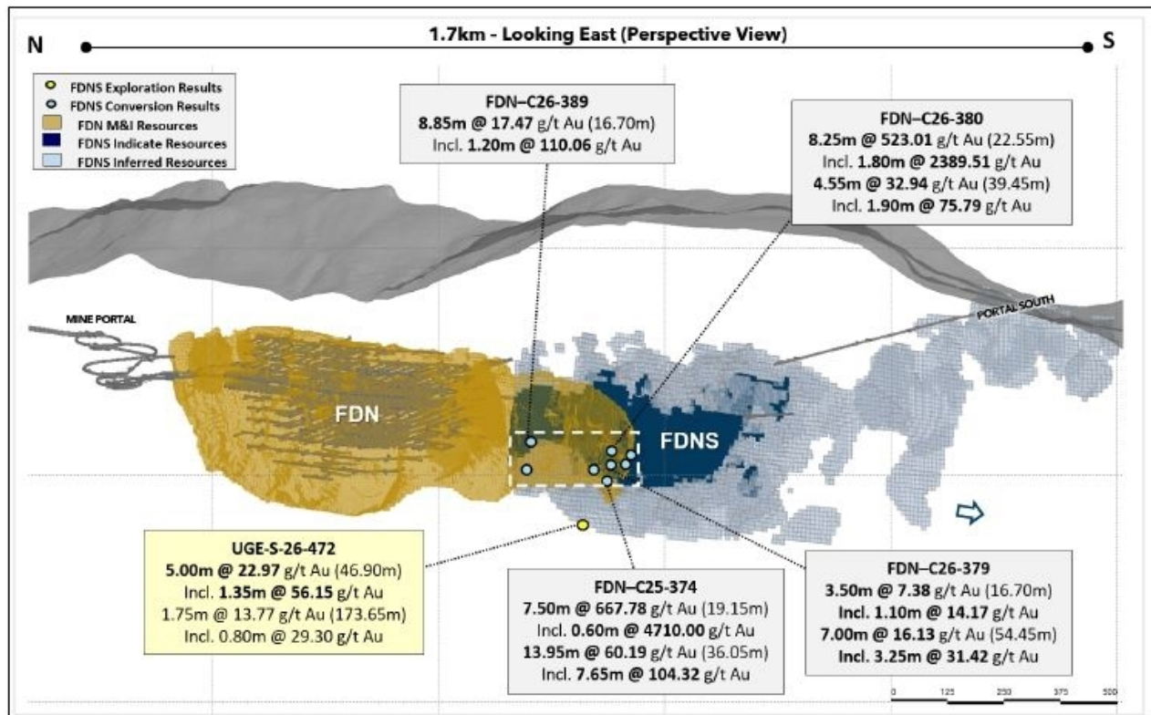
Figure 4: Map showing FDN, FDNS, and FDN East deposits with selected FDN East exploration drilling results
