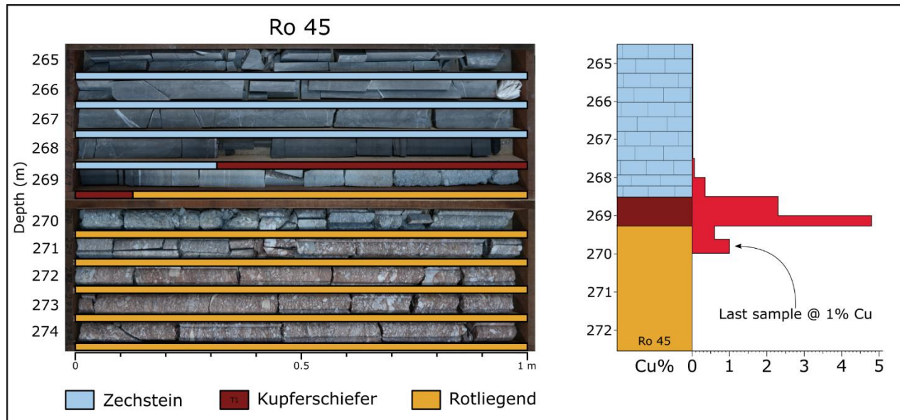
Figure 2: Historical drill core from Ro 45, 1.6% Cu and 19 g/t Ag over 2.7 m from 268 m.
