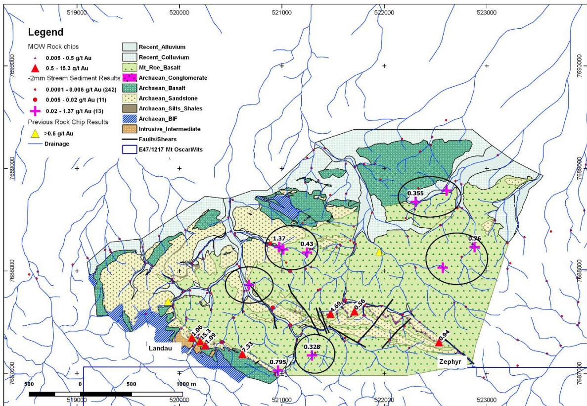
Figure 2: Enlargement of the central area of Figure 1, showing rock chip and anomalous stream sediment results.
