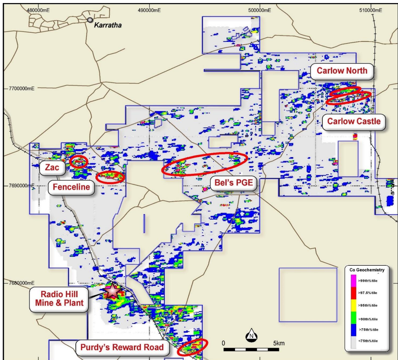
Figure 6: Cobalt Prospectivity identified by Cobalt Geochemical sampling
