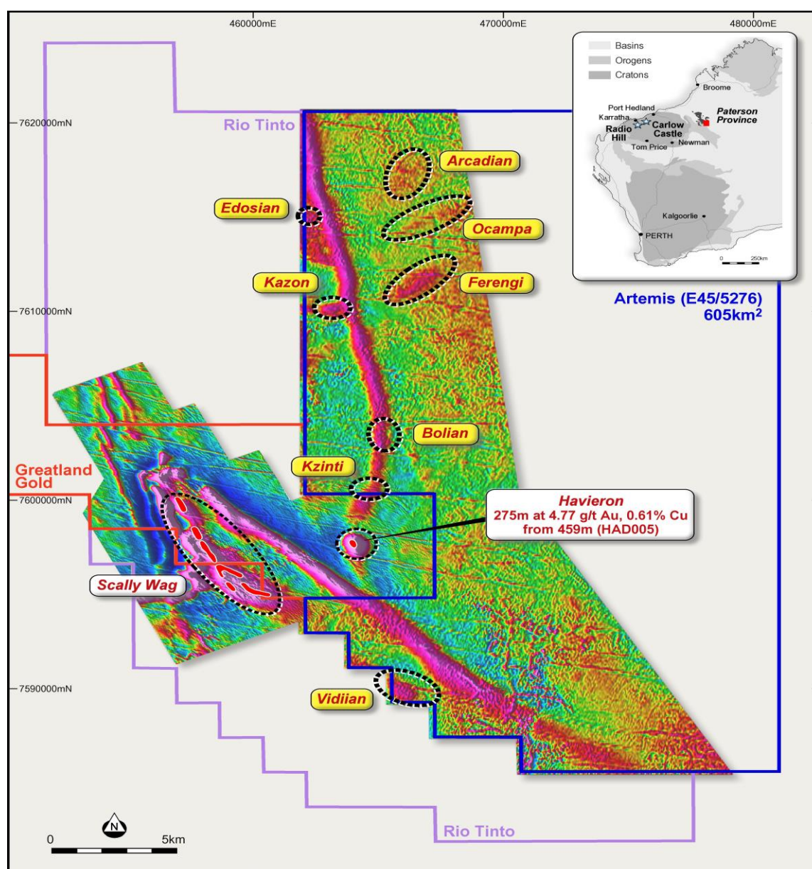
Figure 1: Artemis Armada Prospect in the Paterson Ranges
