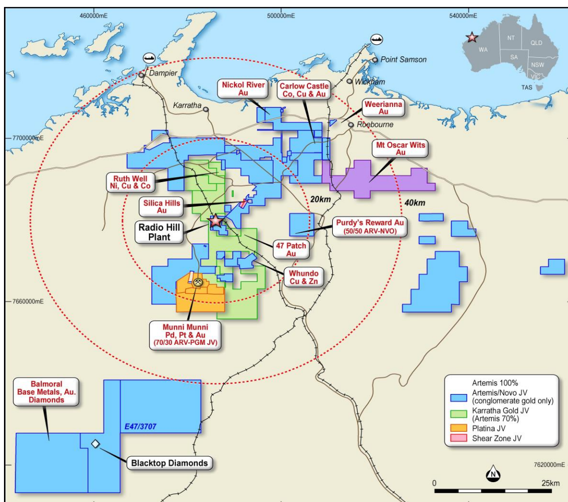
Figure 5: Artemis West Pilbara Asset Map
