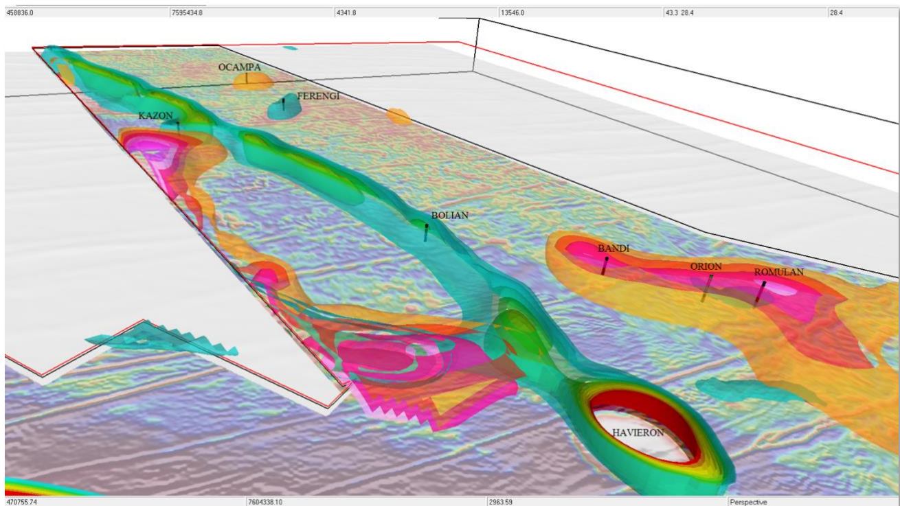
Figure 3 - Armada Project, Paterson Ranges - 3D Inversion Results for Aeromagnetic/Gravity - Primary Target/Potential Deep Drill Holes Highlighted. Warm colours gravity inversion shells and green/cooler colours magnetic inversion shells (with exception of Havieron which is an intense magnetic high).
