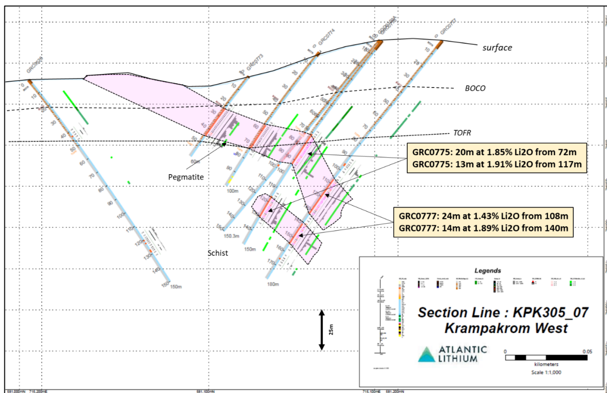
Figure 3: Cross-section B-B' assay results received for GRC0775 and GRC0777 at the Kaapakrom West target.
