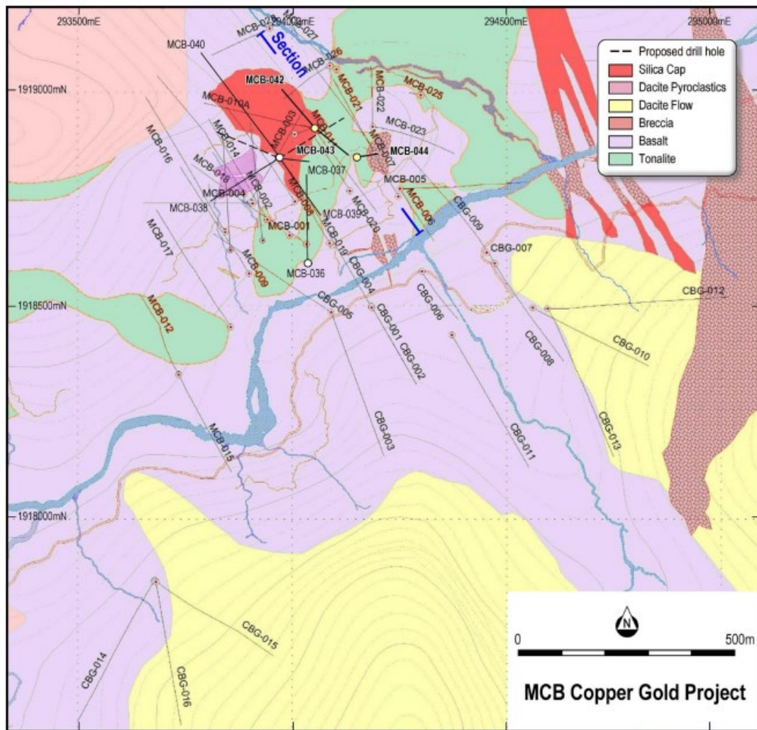
Figure 1. Location of MCB-042 to MCB-044 drill holes relative to recent and historical drilling at MCB
