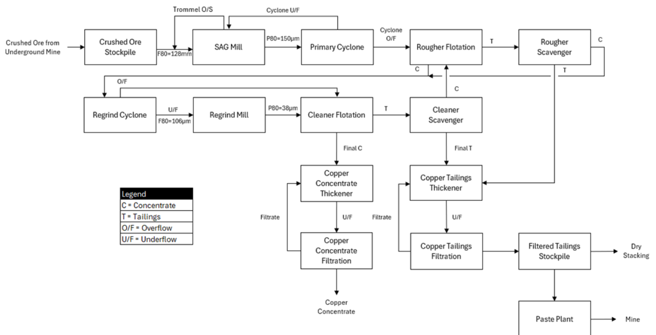
Figure 8. Process Flow Block Model
