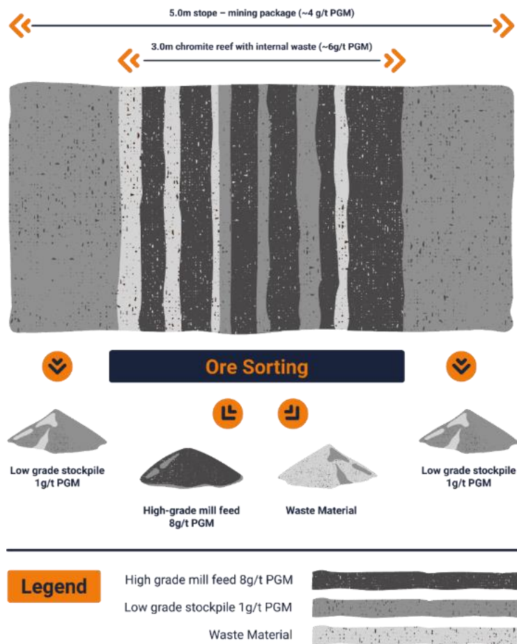
Figure Nine | Ore Sorting Schema
