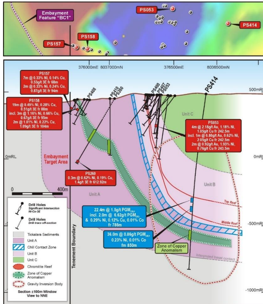
Figure Four | Cross Section for Drill Hole PS414
