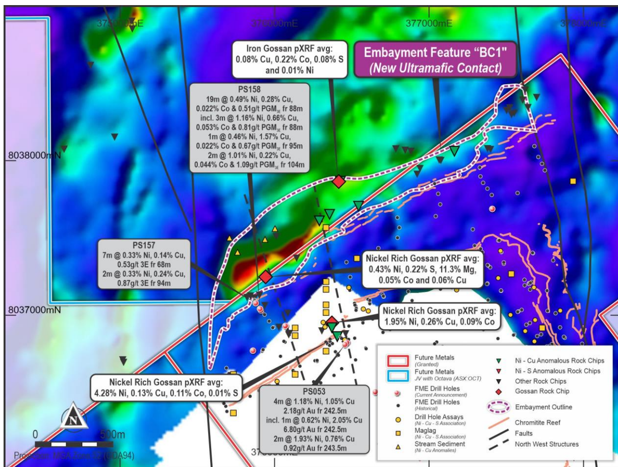
Figure Five | Plan view of BC1 with HoistEM
