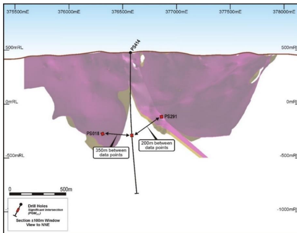
Figure Three | Orthogonal view showing location of PS414 intersection of the high-grade PGM reef relative to the nearest holes in the NNW and NE
