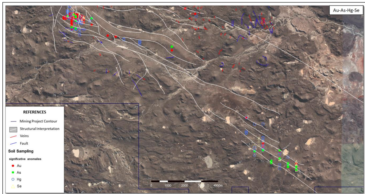
Fig 3. Structural features with Au, Hg and As anomalism, and vein swarms
