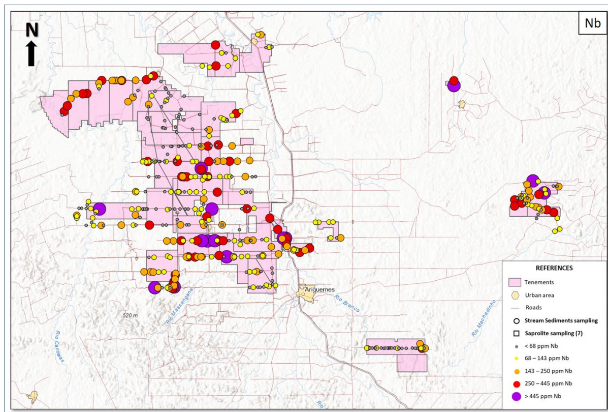
Fig 5. Niobium in streams
