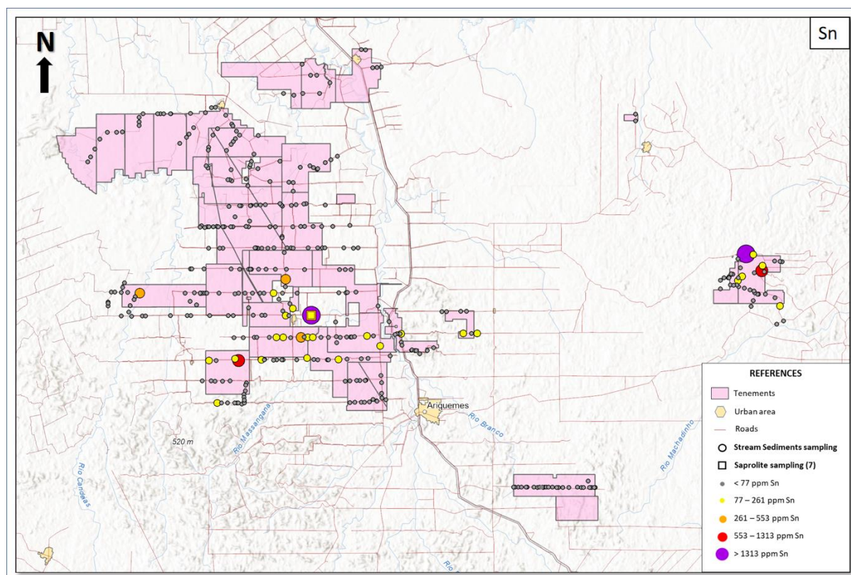
Fig 4. Tin in streams
