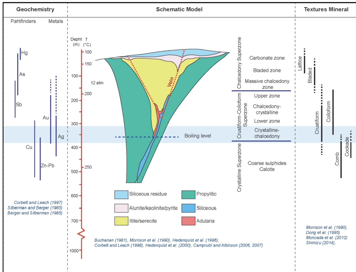
Fig 1. Low Sulphidation Schematic – Poster by Williams Mata Rimac
