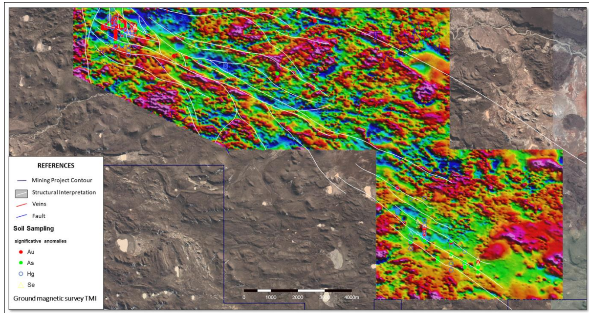
Fig 2. Ground magnetic surveys with Au, Hg and As anomalism
