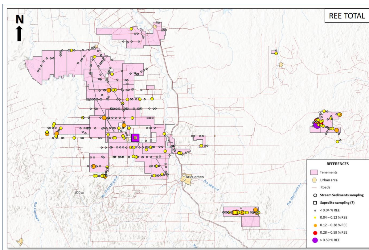
Fig 5, Rare earths in streams
