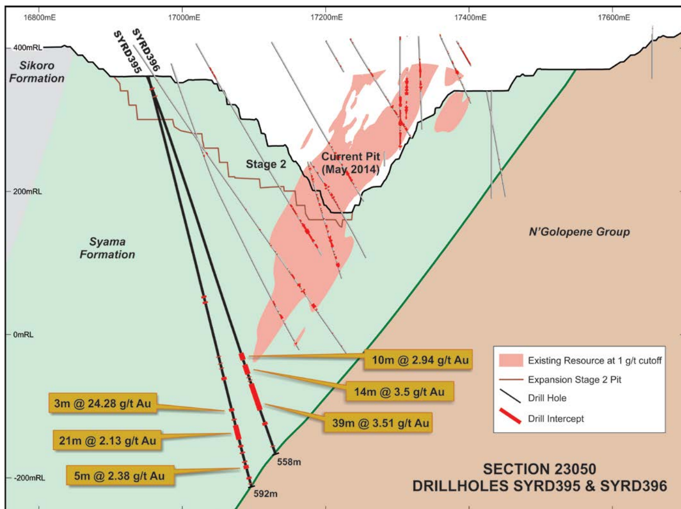
Figure 4 – Section 23050m Nth
