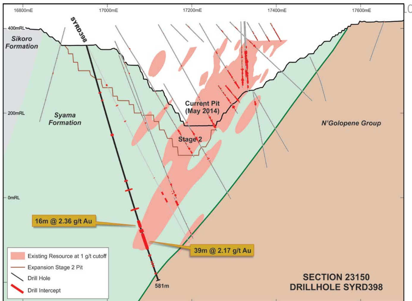
Figure 6 – Section 23150m Nth
