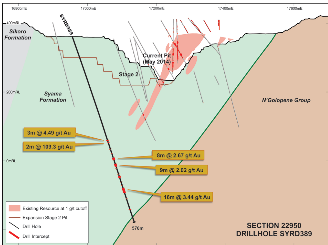
Figure 2 – Section 22950m Nth
