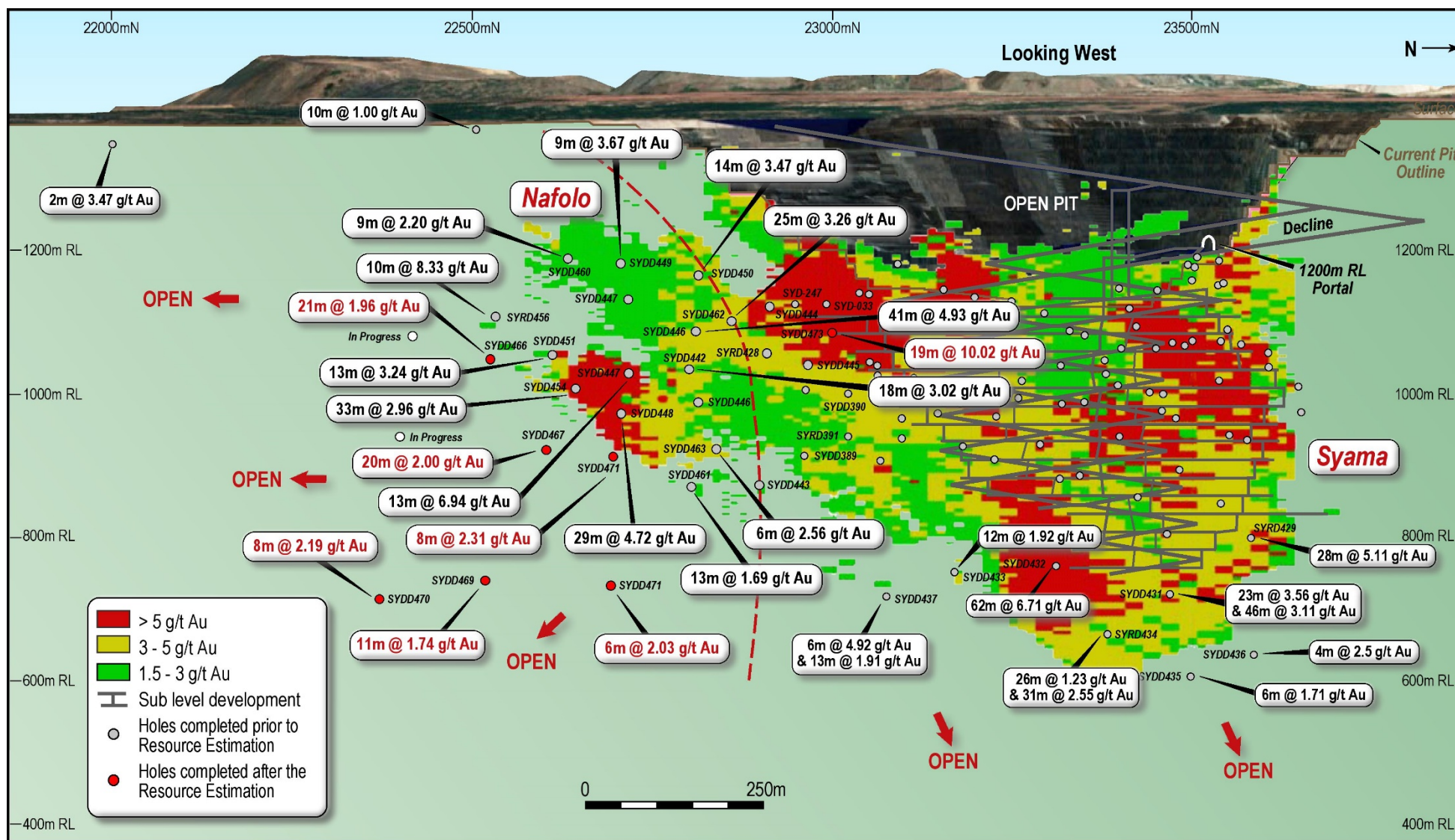
Figure 1: Longitudinal projection of Syama showing updated resource model, drilling results and current underground development design
