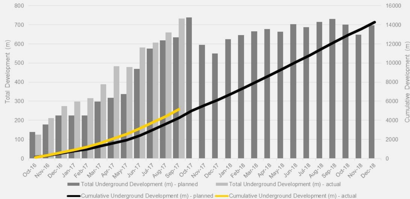
Syama Underground - Total Underground Development
