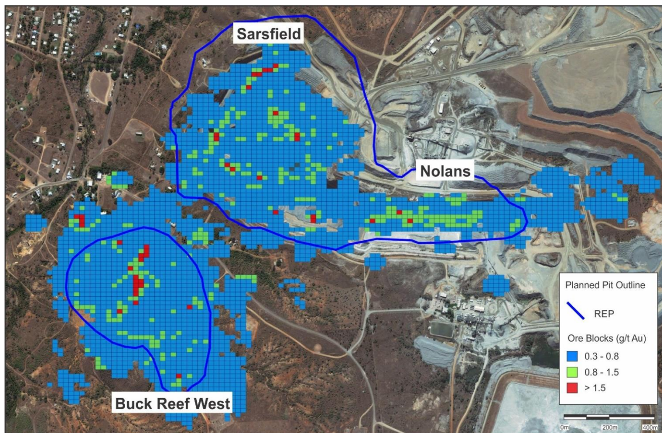
Figure 5: Buck Reef West, Sarsfield and Nolans pits with updated Mineral Resource block model
