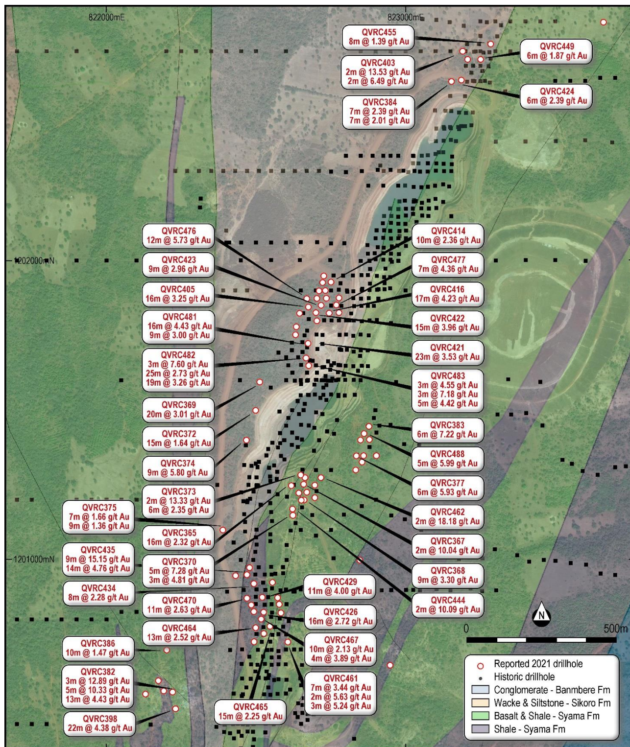
Figure 3. A21 area imagery, geology and drillhole locations
