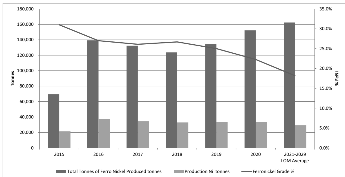
Figure 15-4: Ferronickel production profile
