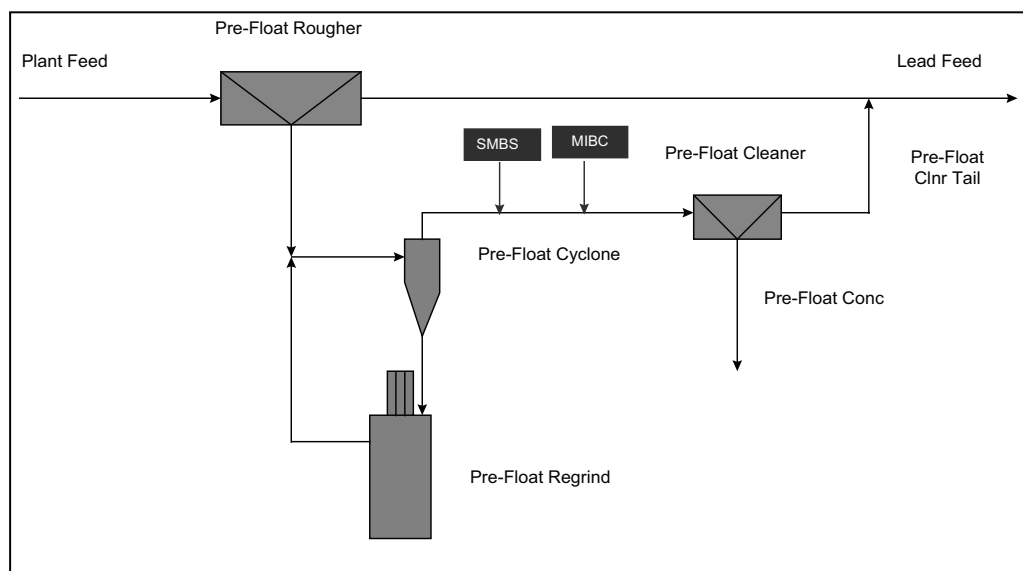
Figure 4.13: Cannington Operations Ore Treatment Talc Pre-Float Flowsheet
