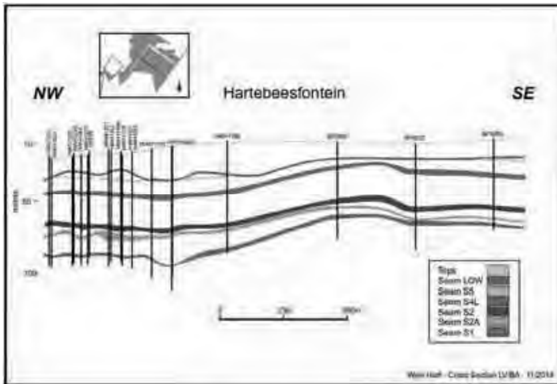
Figure 5.11: Cross-section through Hartbeestfontein pit showing rolling seams
