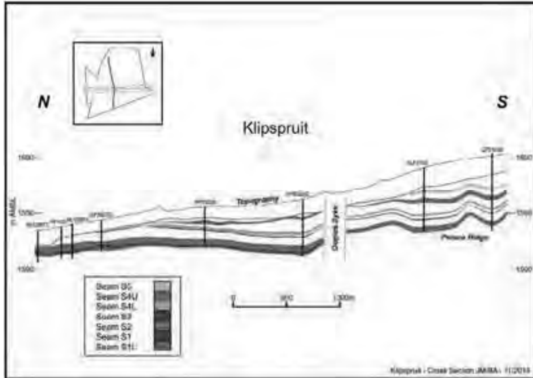
Figure 5.32: North-south cross-section through Klipspruit
