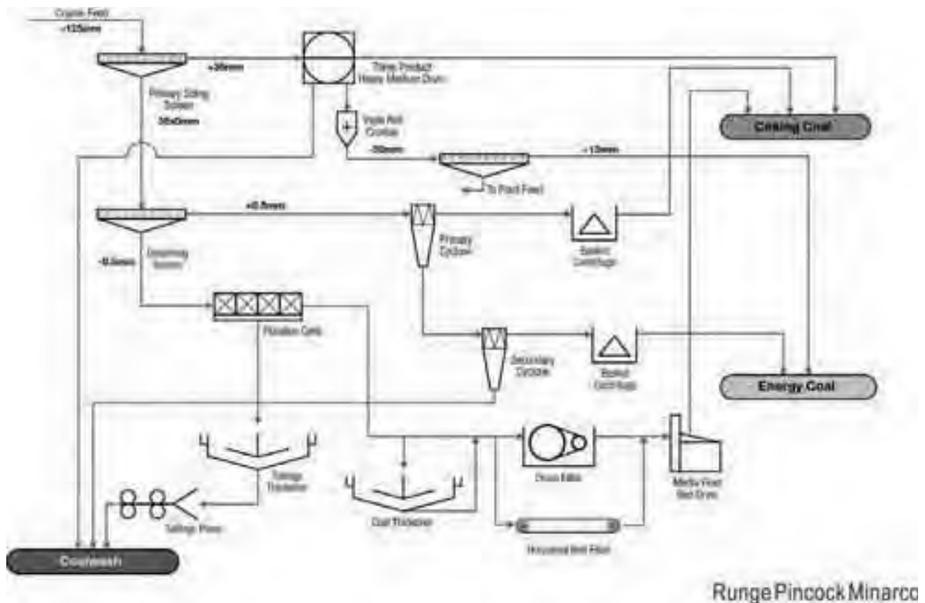
Figure 9-2 - Dendrobium Coal Handling and Processing Plant Flow Sheet
