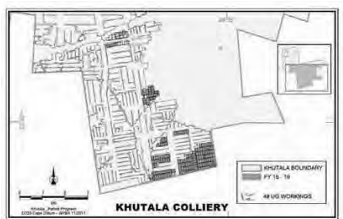
Figure 5.48: Progress plan of No.2 Seam
