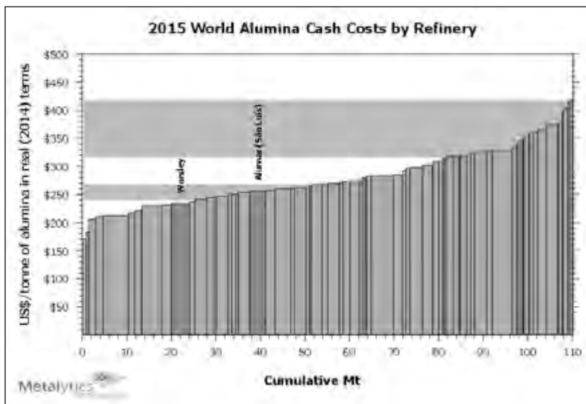
Figure 15-10: C1 Alumina cash costs
