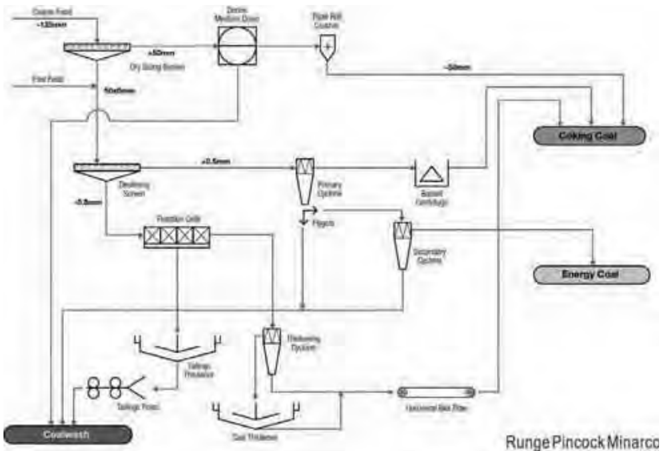
Figure 9-1 – West Cliff Coal Processing Flow Sheet
