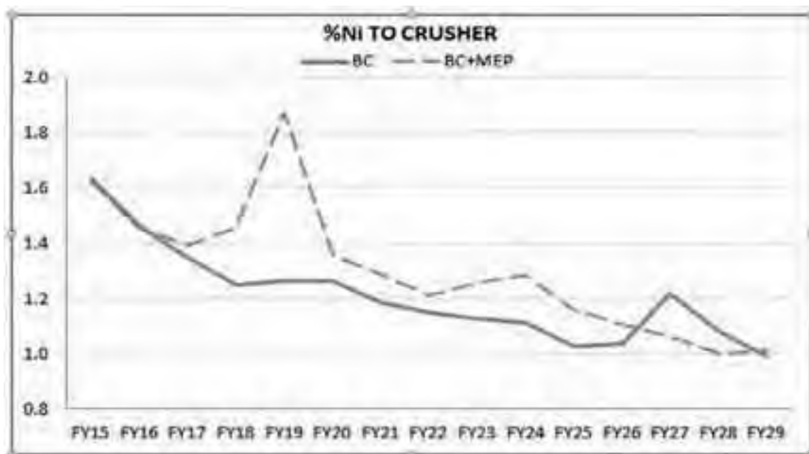
Figure 8-3: Projected crusher feed grades
