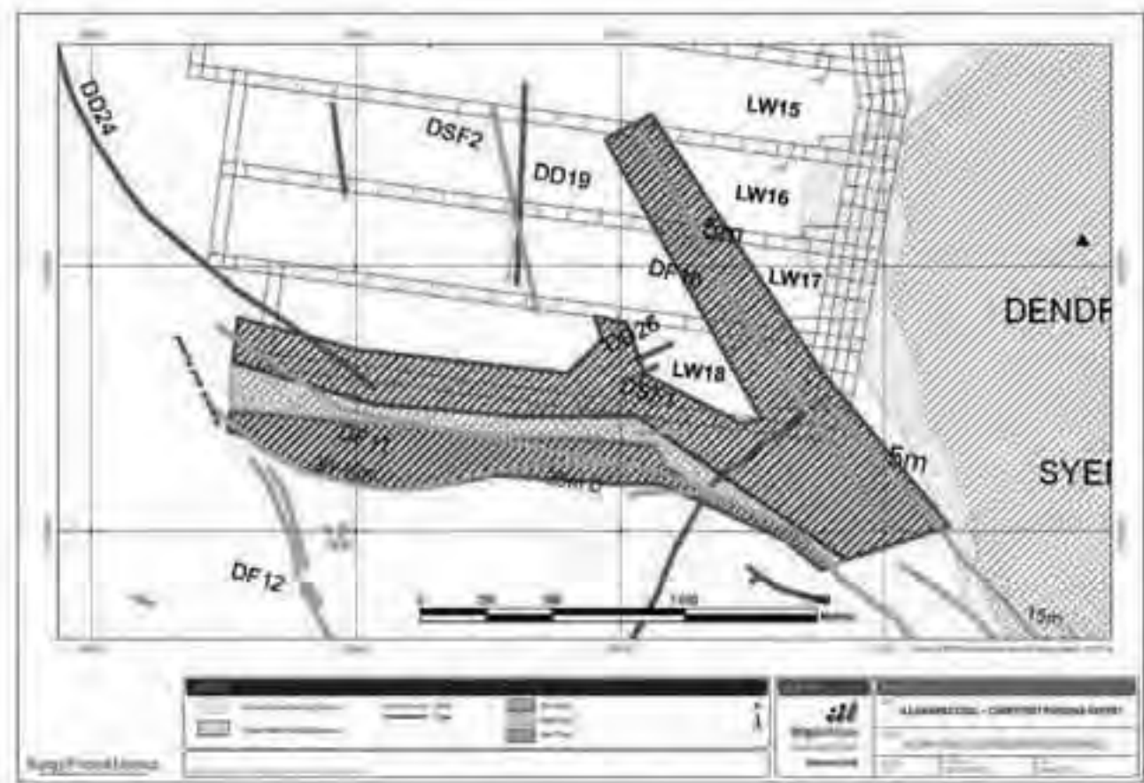
Figure 7-8 - Eloura Fault Disturbed Ground Boundaries
