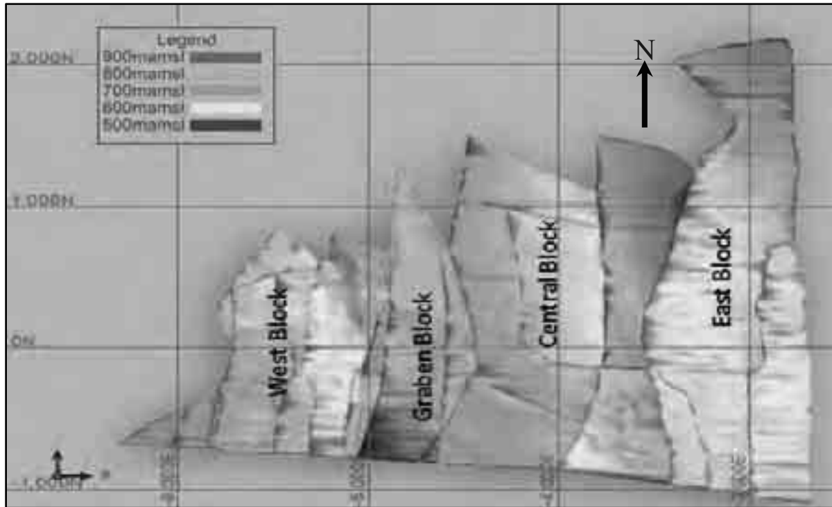
Figure 31 Plan indicating structural zones
