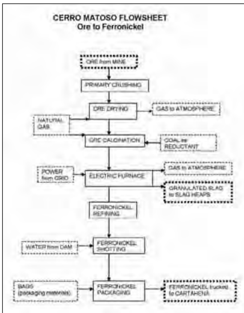
Figure 8-4: Processing flowsheet
