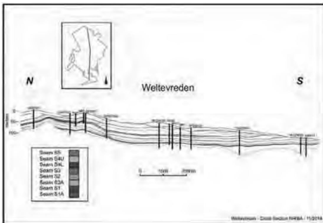
Figure 6.3: Weltevreden cross-section
