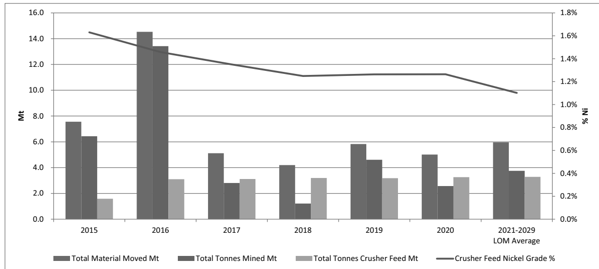
Figure 15-3: Mine production profile
