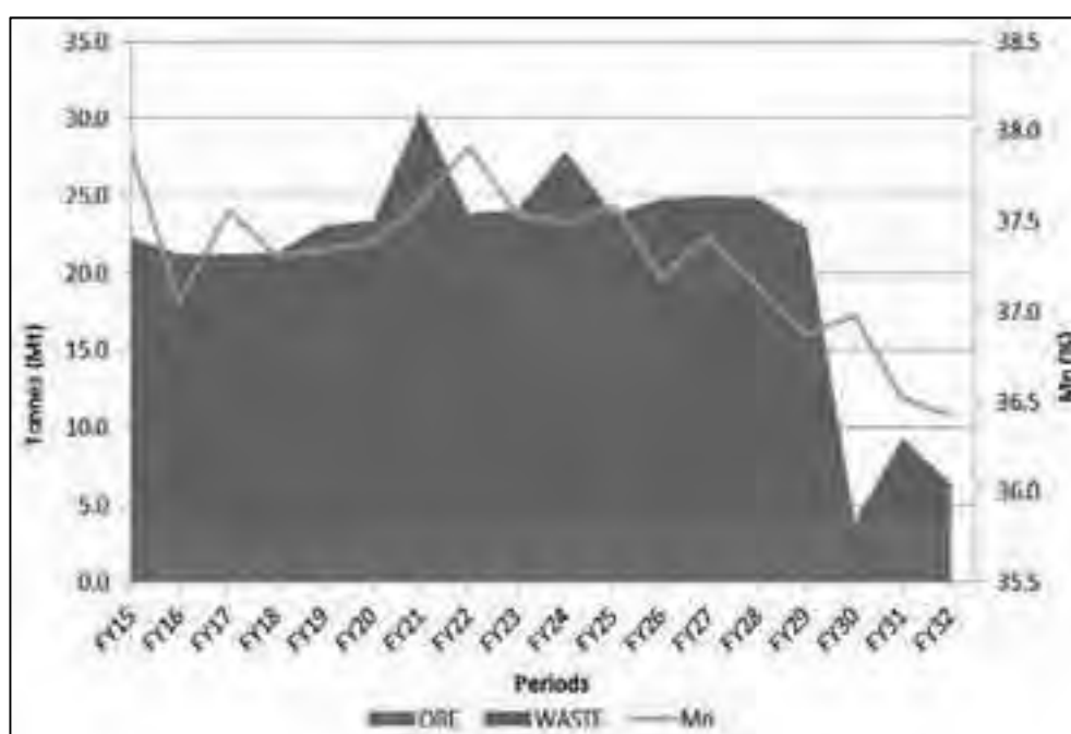
Figure 24 Mamatwan Mine production profile
