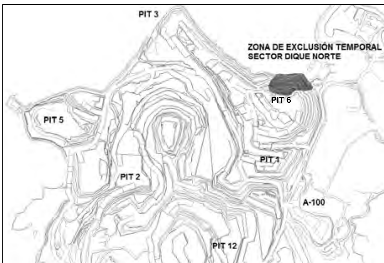
Figure 7-1: Pit numbering of Cerro Matoso pit
