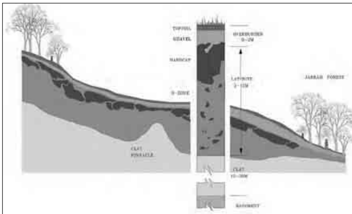
Figure 3-2: Typical profile of Darling Range bauxite
