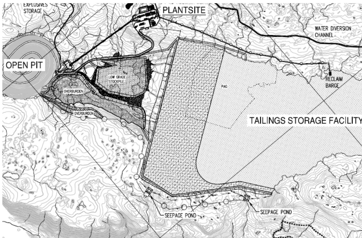
Figure 18-3 Tailings Containment
