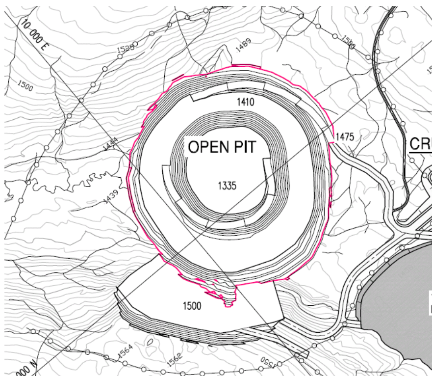
Figure 18-8 Prosperity Mine Development – End of Year 2
