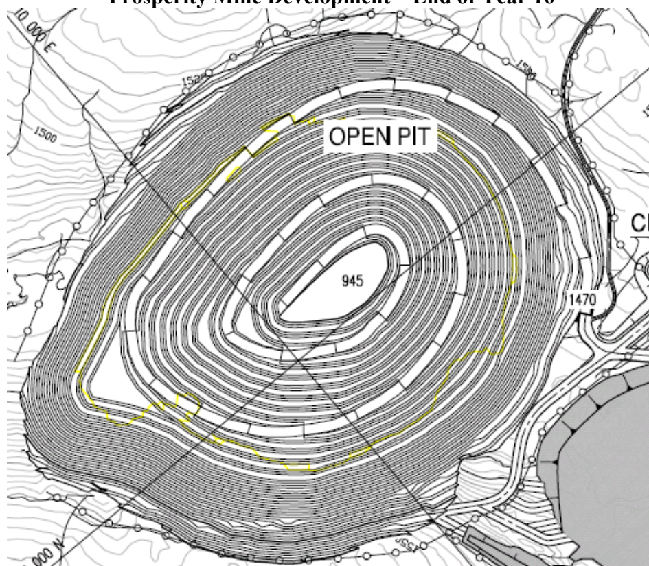
Figure 18-11 Prosperity Mine Development – End of Year 16
