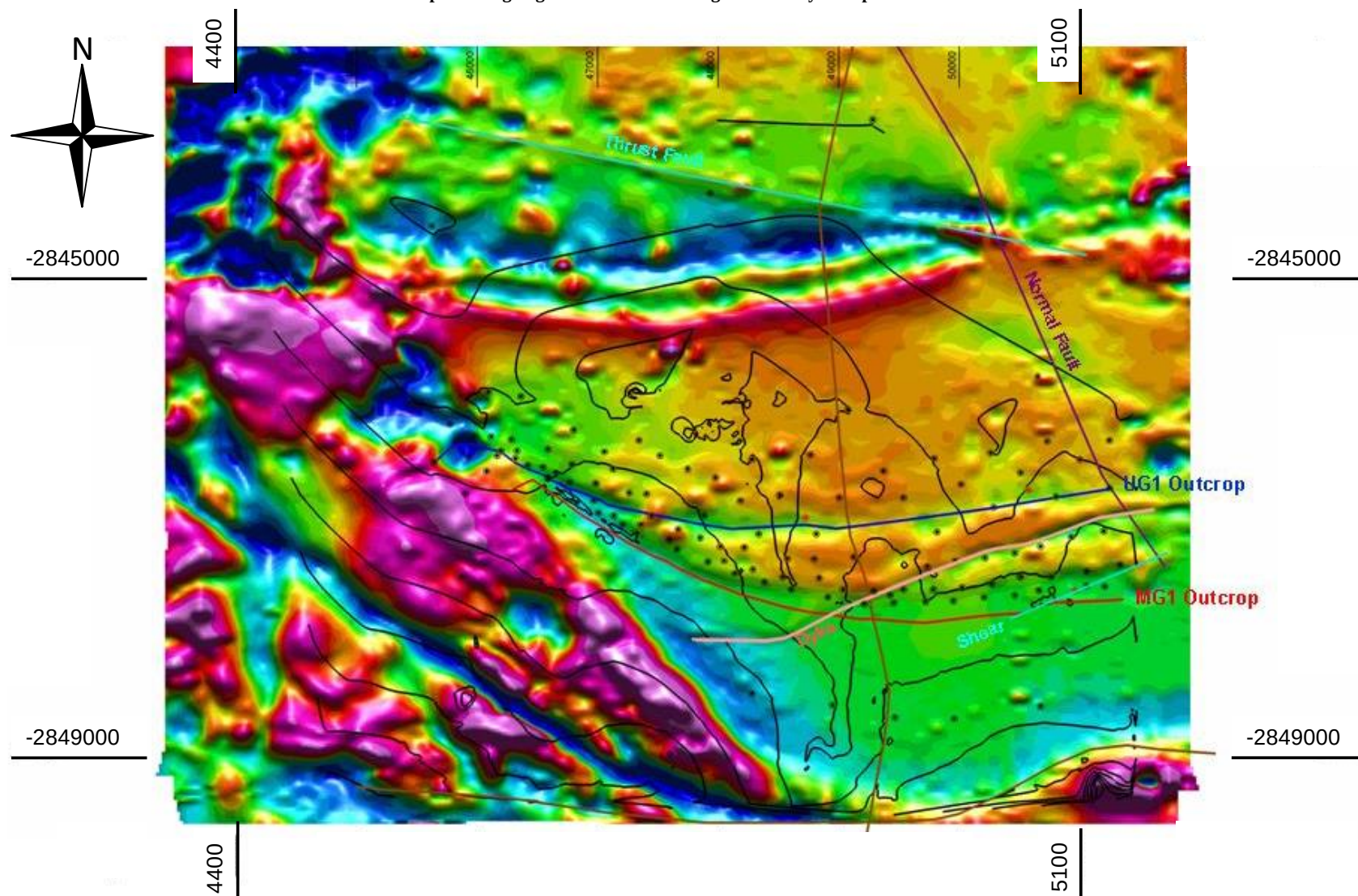
Figure 6.4_1 Map Showing High Resolution Aeromagnetic Survey Interpretation
