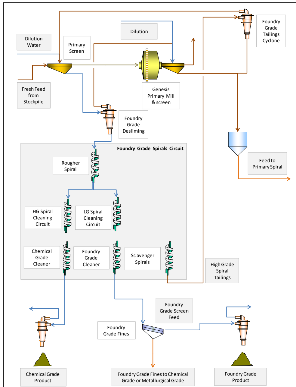
Figure 11.2_1 Phase 1 Foundry Grade Project Simplified Flow Diagram
