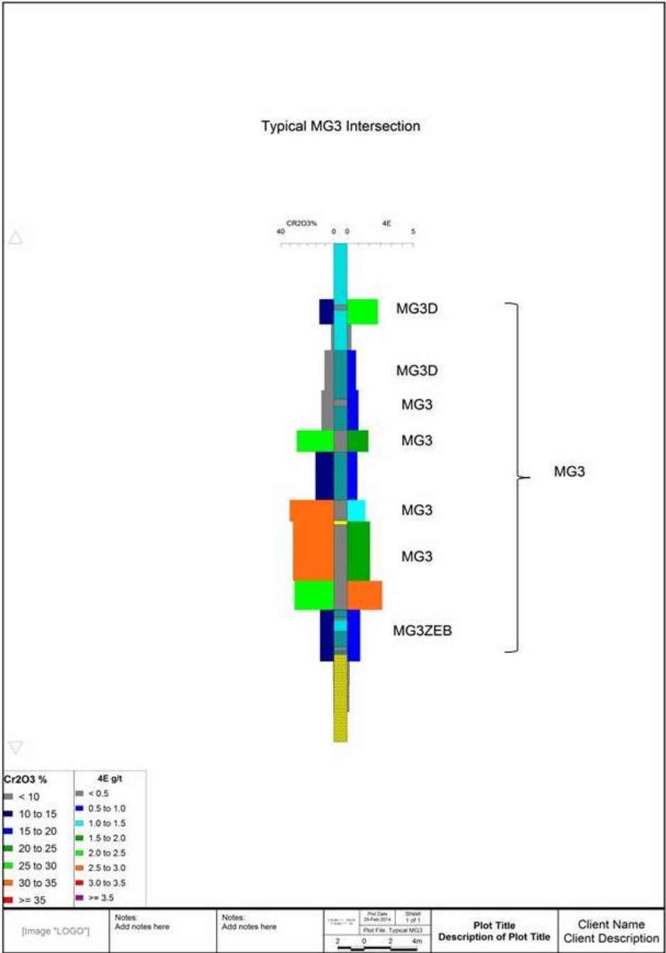
Typical MG3 Chromitite Layer Cr 2 O 3 and 3PGE+Au geochemical signature
