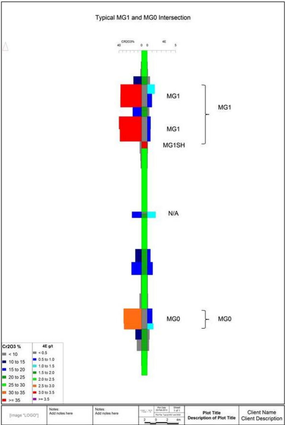
Typical MG1 Chromitite Layer Cr 2 O 3 and 3PGE+Au geochemical signature
