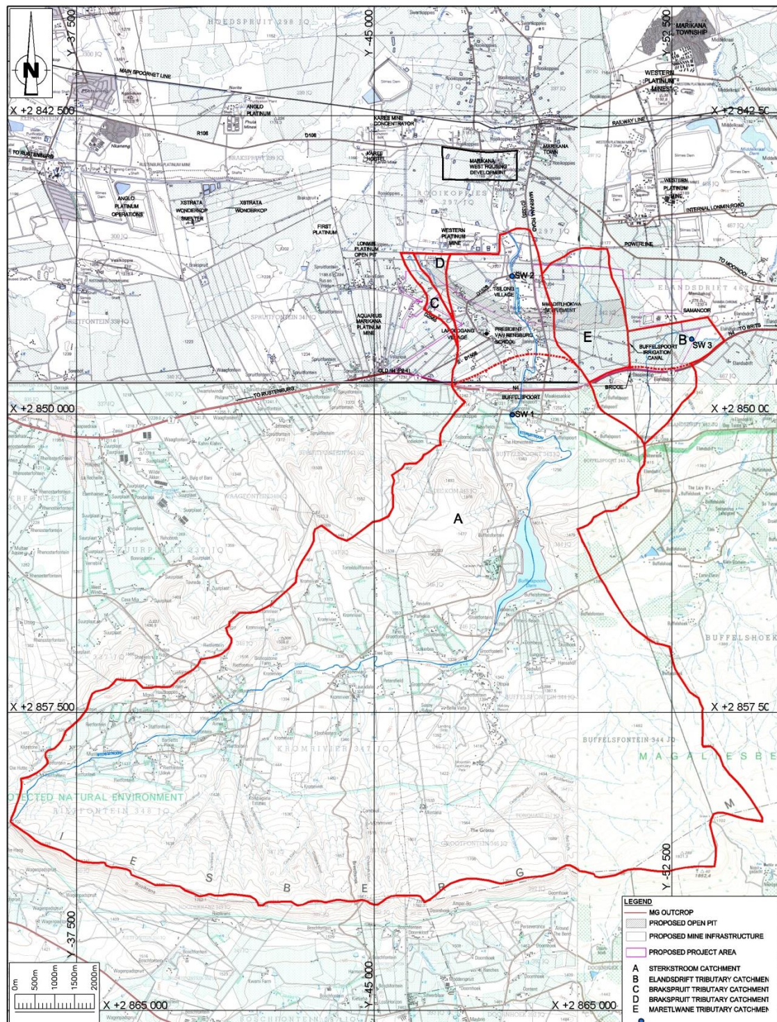
Figure 4.8_1 River Systems and Catchment Boundaries in the Mine Area
