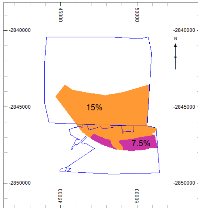
Figure 8.10_1 Map showing the Applied Geological Loss
