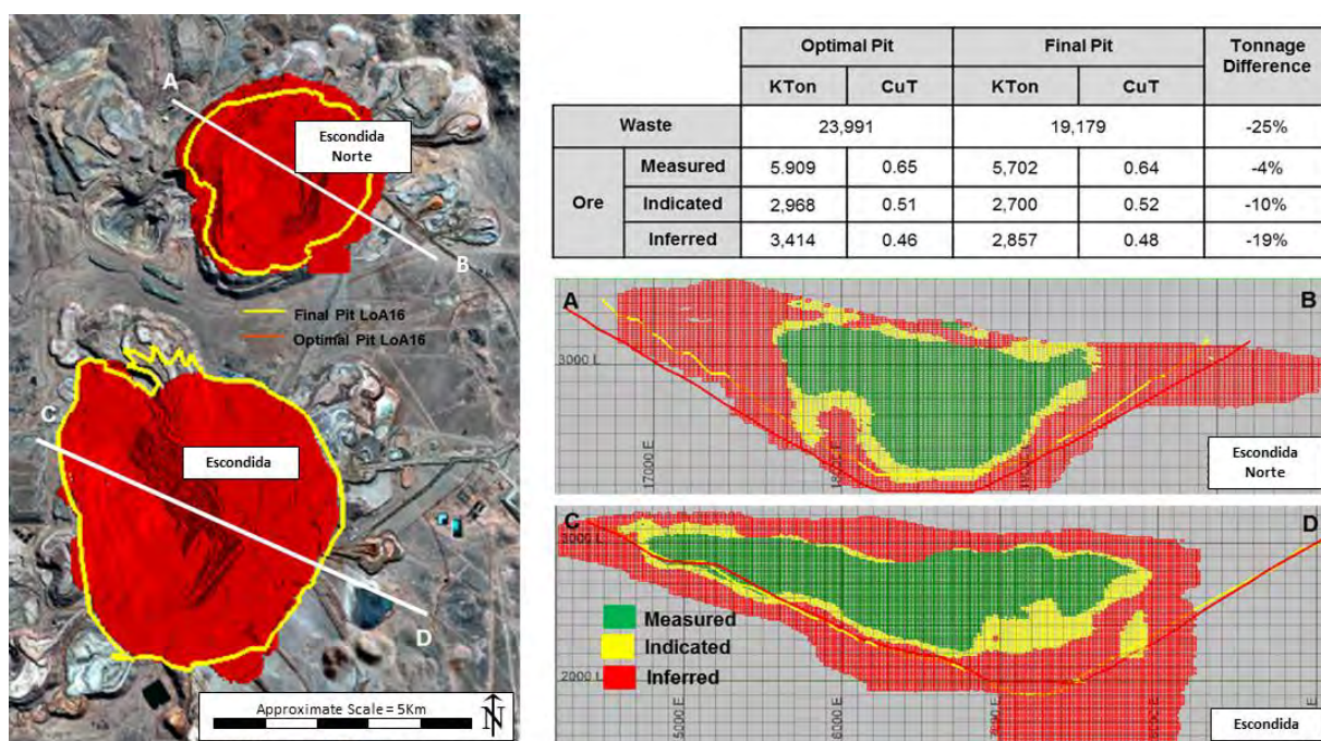
Figure 12: Optimal Pit Vs Final Pit Comparison
