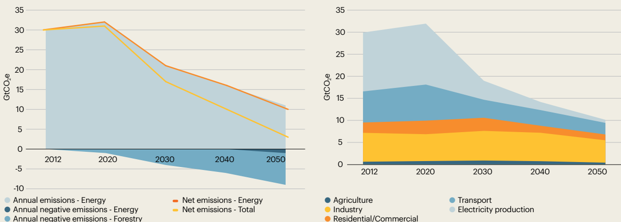
Figure 5: CCUS + BECCS in 1.5°C Scenario
