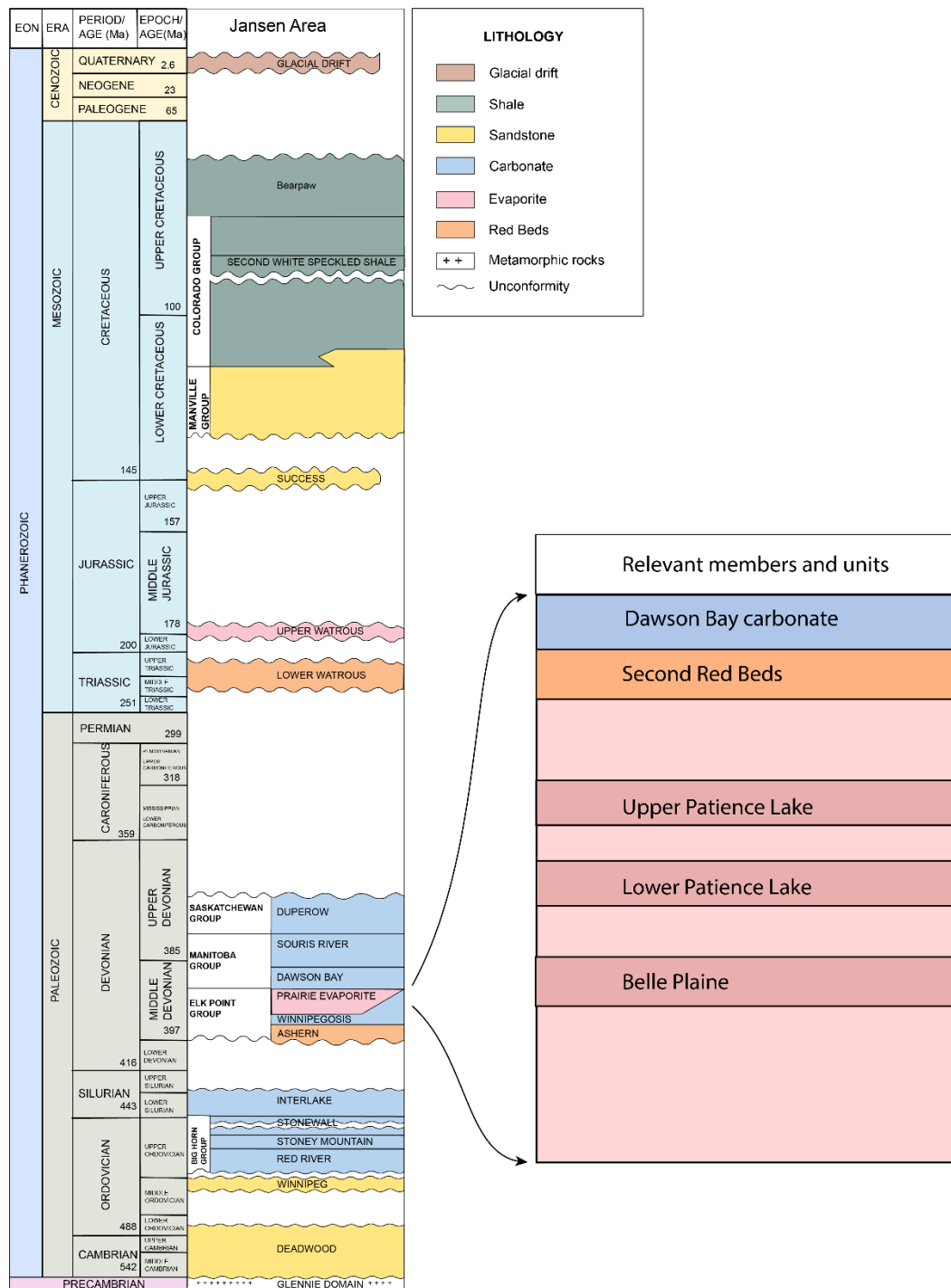
Figure 5. Stratigraphic column for Jansen area
