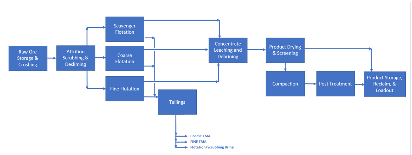
Figure 12 Jansen Process block flow diagram
