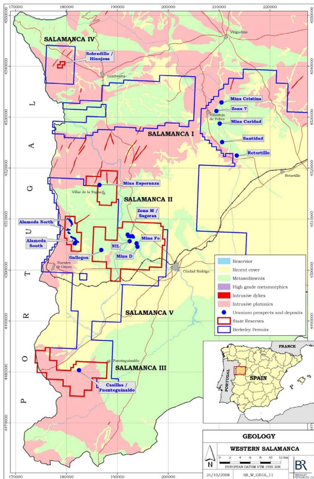
Figure 3 – Salamanca area uranium deposits
