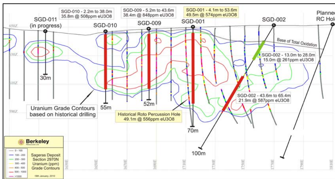
Figure 6 – Sageras Cross Section 2970N
