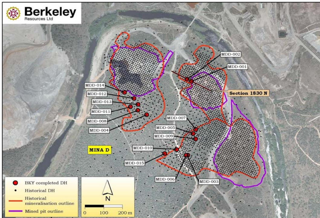
Figure 3 – Location of drill holes at Mina D Deposit
