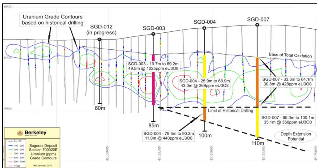
Figure 7 – Sageras Cross Section 700020E
