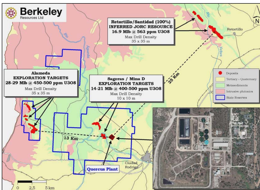
Figure 1 – Salamanca Uranium Project
