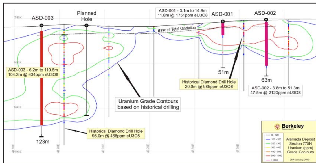
Figure 9 – Alameda South Cross Section 775N
