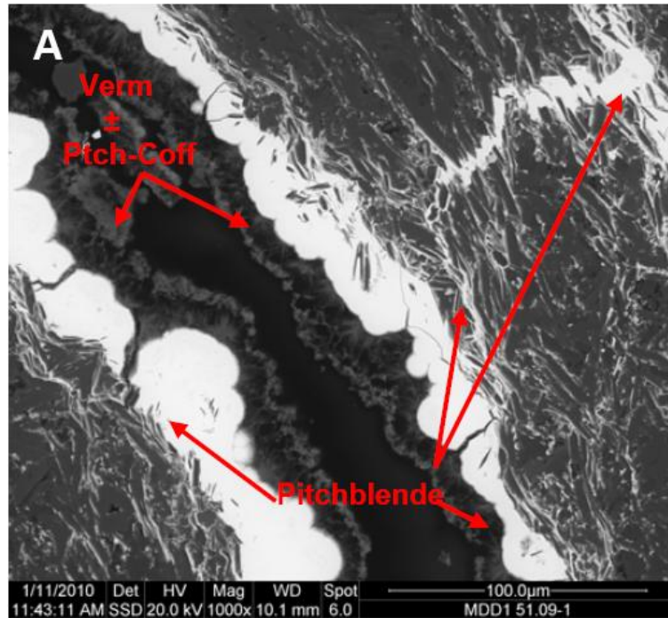
Figure 2 – Photomicrograph of Colloform pitchblende aggregates along the walls of a vein.
