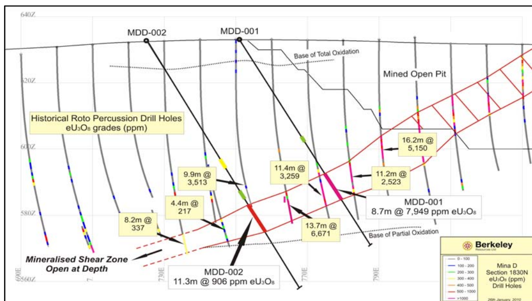
Figure 4 – Mina D 1830N section
