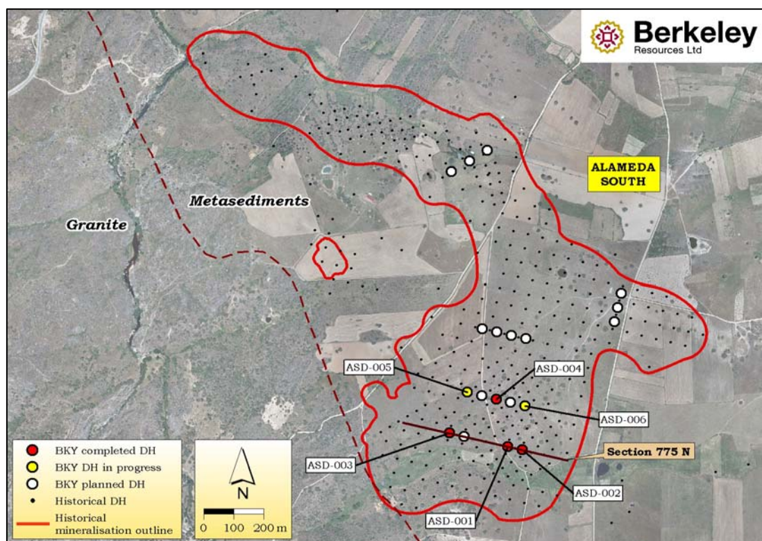
Figure 8 – Location of drill holes at Alameda Deposit
