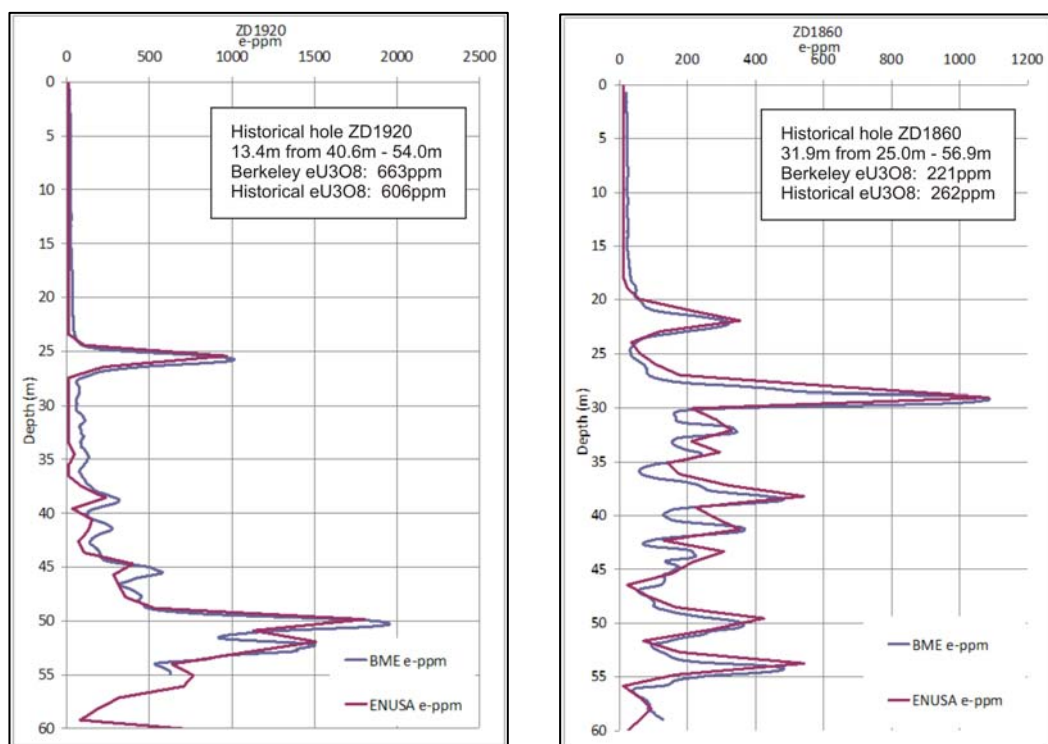
Figure 11 – Zona D Holes 1920 and 1860 Berkeley and historic e-grades.
