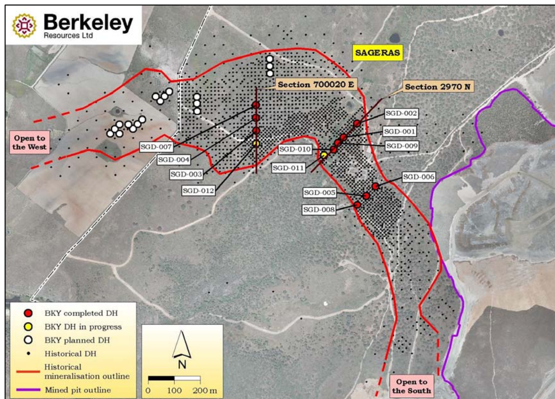
Figure 5 – Location of drill holes at Sageras Deposit
