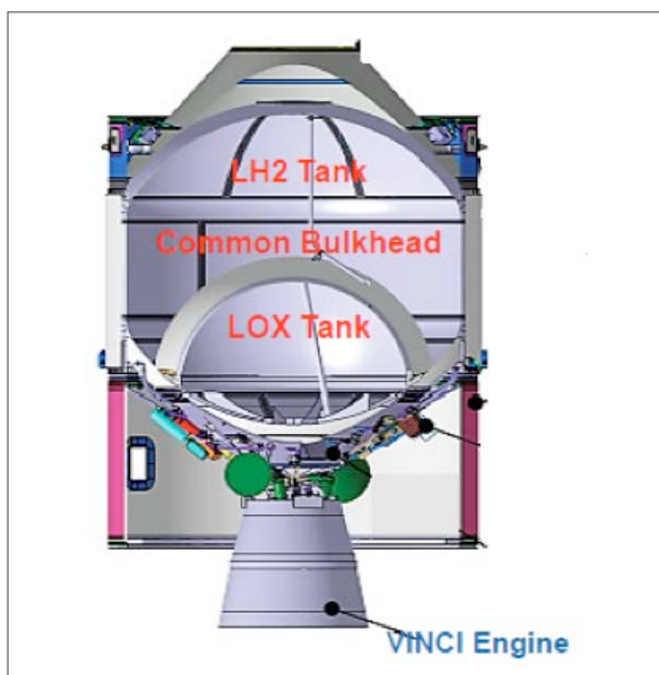
Enlarged upper stage tanks of the ARIANE 5 ME
