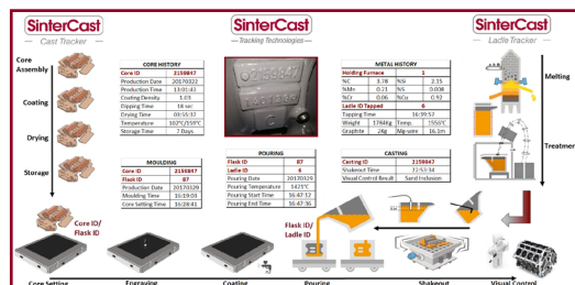
Real-time position monitoring and tracking with Cast Tracker.
