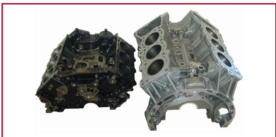
The Audi 3.0 litre V6 with a CGI cylinder block is 15 kg lighter than the Mercedes 3.0 litre V6 based on an aluminium cylinder block.
