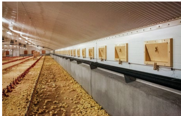
TPI's air inlet valves in a chicken barn
