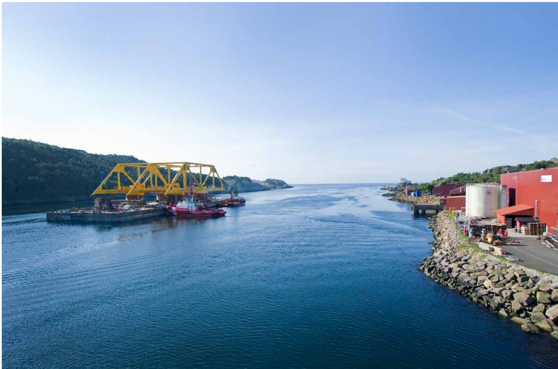
In June 2013, Aker Solutions delivered the steel frame for the world's first subsea gas compression facility to be installed at the Statoil-operated Åsgard field.
