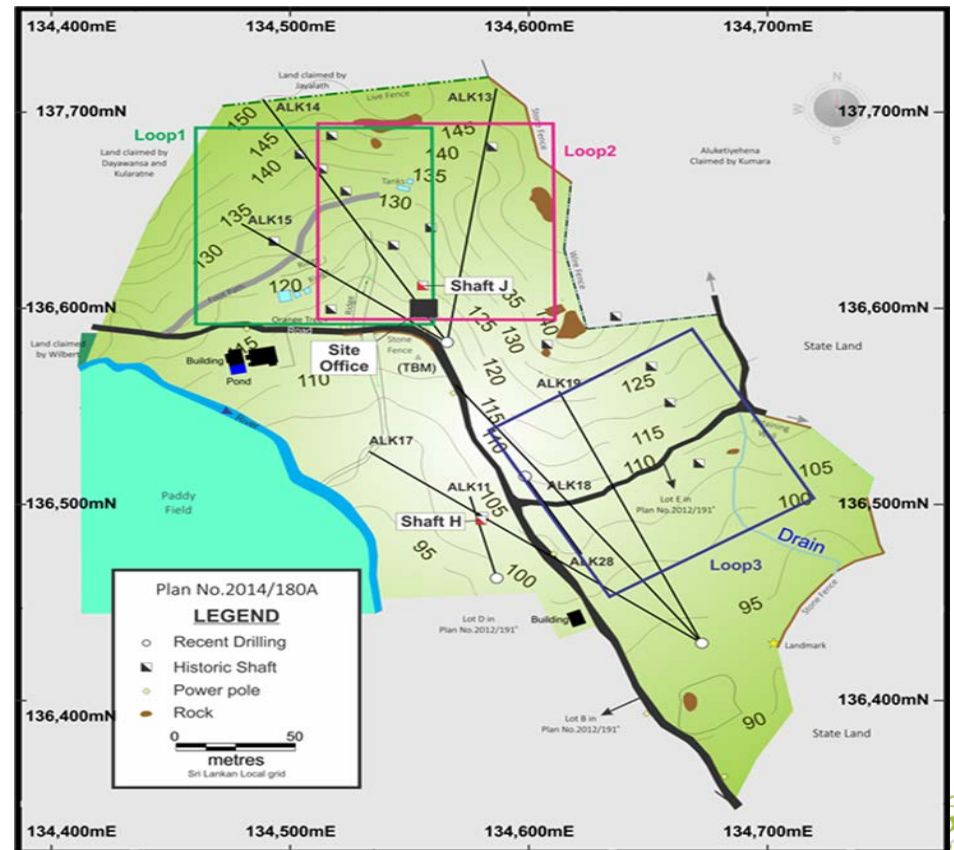
Aluketiya project site plan with Shafts H and J and exploration drill hole traces and transmitter loop locations
