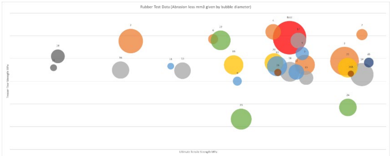
Figure 2: Bubble chart demonstrating mechanical performance of various graphene enhanced rubber formulations. Y axis represents tear strength, X axis represents tensile strength and the bubble diameter shows abrasion loss.
