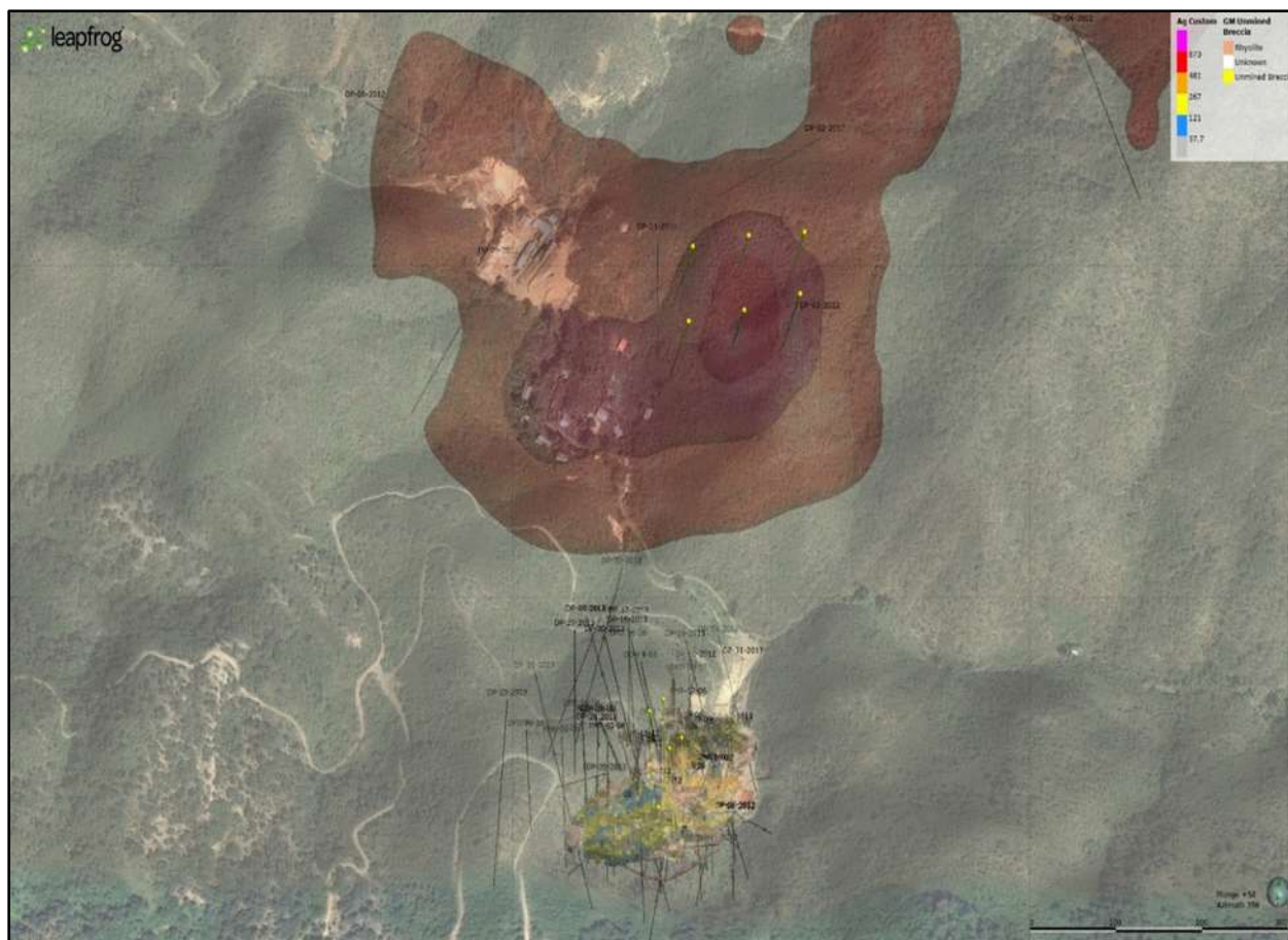
Figure 6.7. Chargeability at 200m below topography. Higher amplitude anomalies are purple shades.
