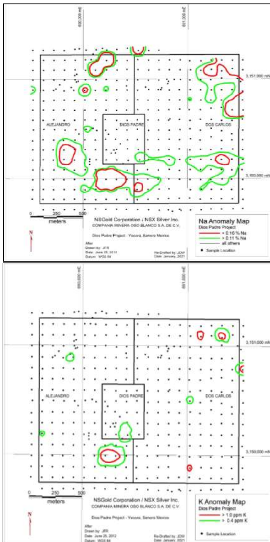
Figure 6-3. Na (top) and K (bottom) anomalies (after Duncan, 2012).
