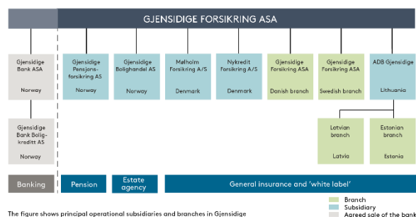
Figure 1 – Business structure
