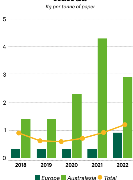
DISCHARGES OF SUSPENDED SOLIDS (SS) Kg per tonne of paper
