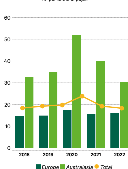
DISCHARGES OF WASTEWATER m³ per tonne of paper
