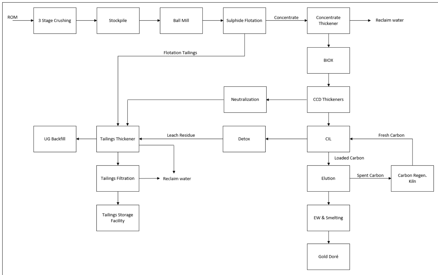
Figure 13-7 New Polaris Process Flowsheet
