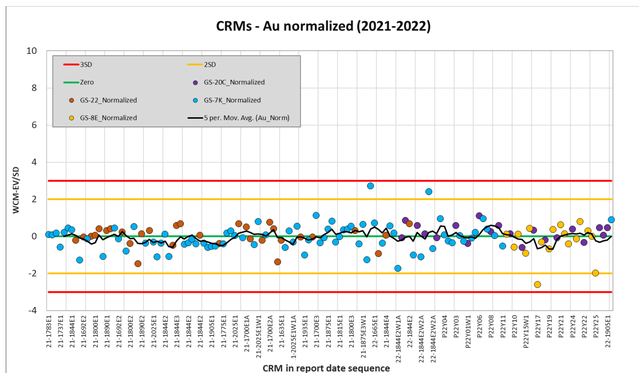
Figure 11-11 PCC Standards Performance 2021-2022 - Au
