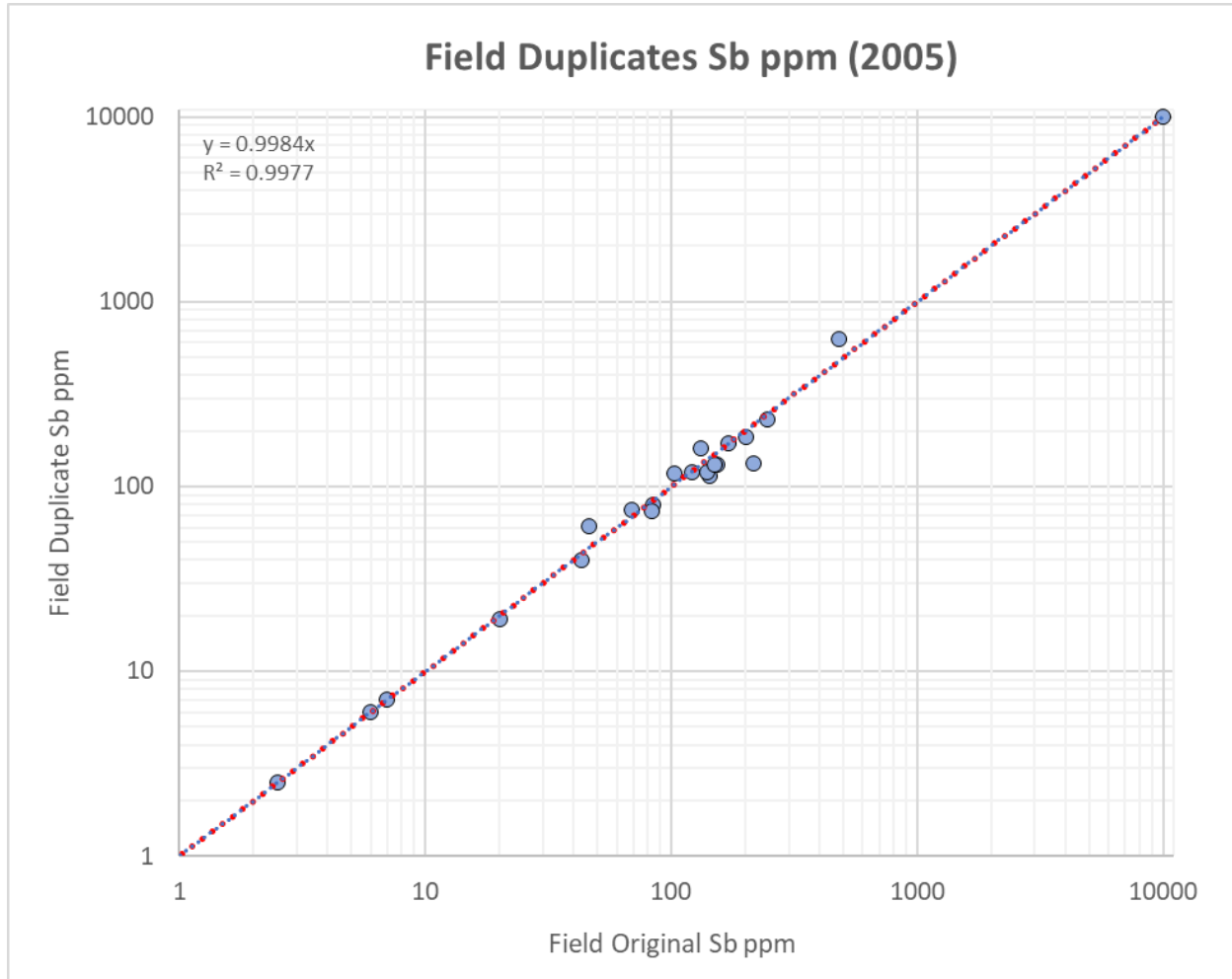
Figure 11-4 Field Duplicate Performance - Sb
