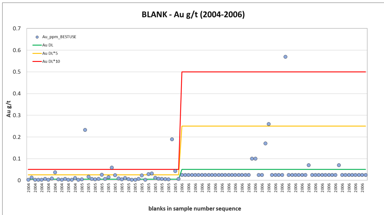
Figure 11-1 Blank Performance 2004-2006 - Au
