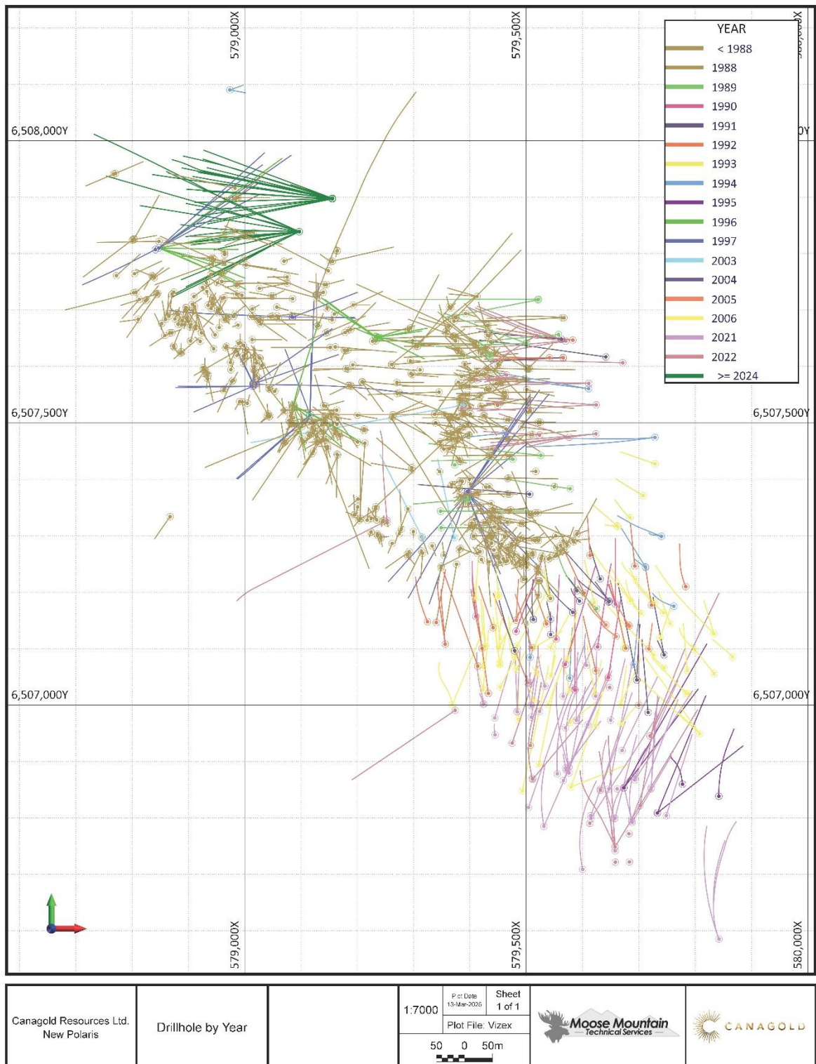
Figure 10-1 Plan view of Drillhole Locations by Year
