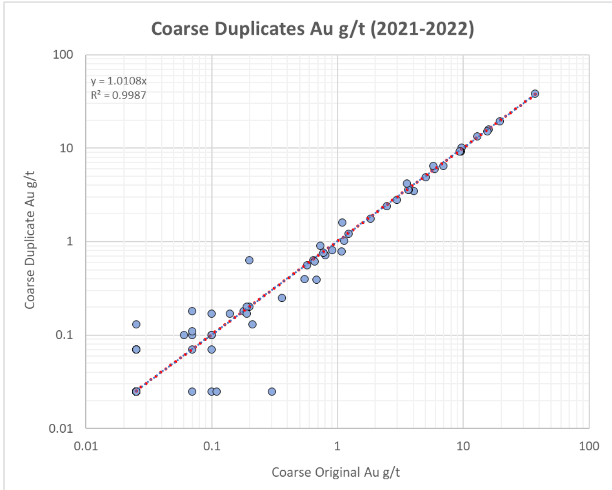
Figure 11-9 Coarse Duplicate Performance 2021-2022 – Au
