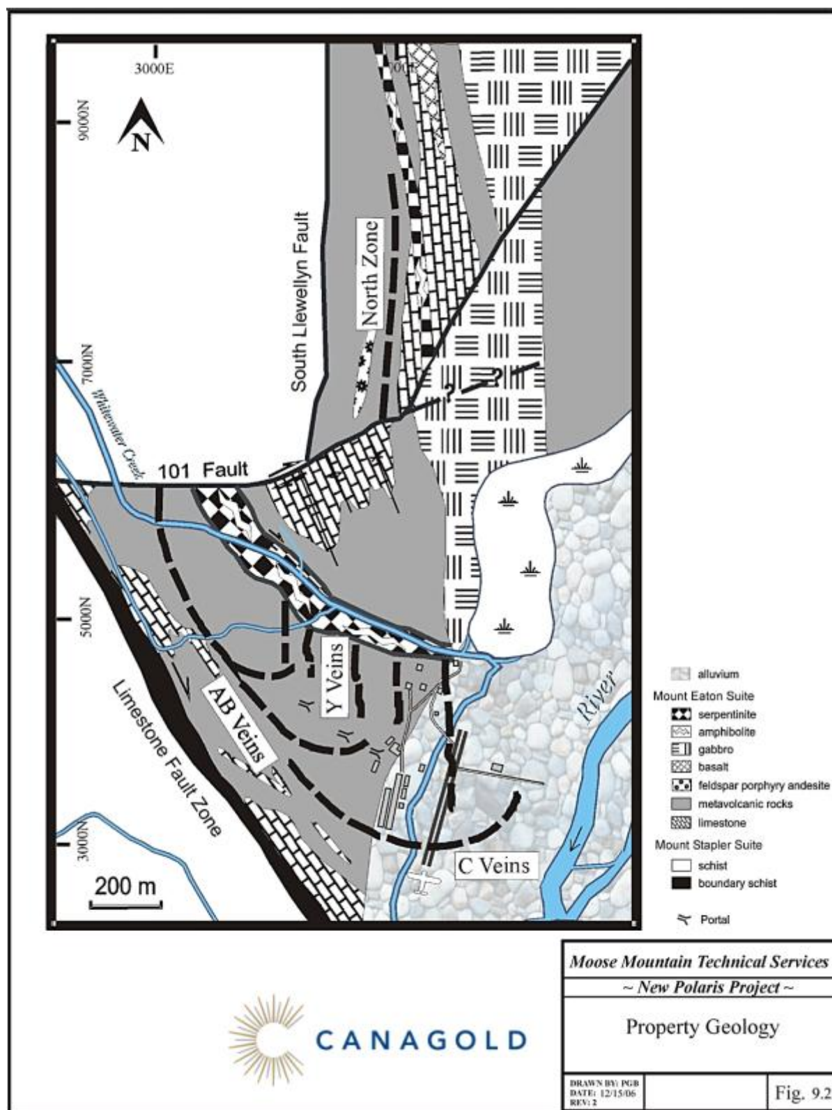
Figure 7-2 Property Geology
