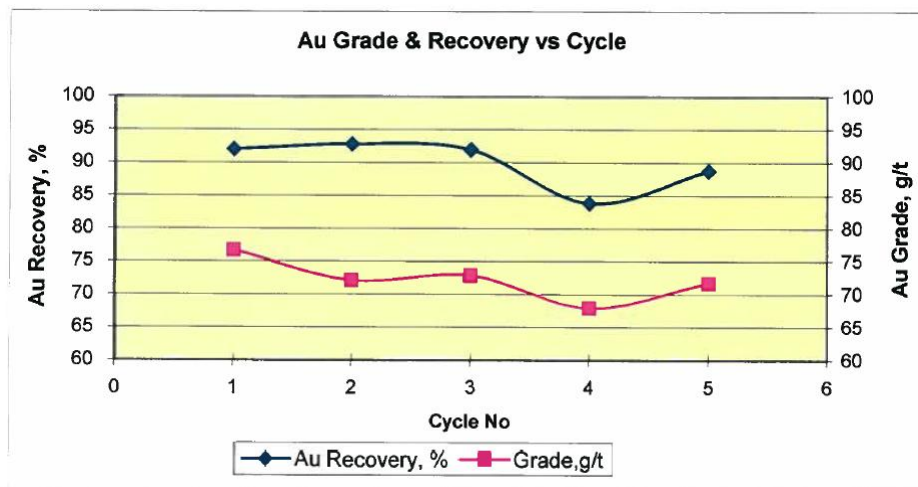
Figure 13-3 Locked Cycle Test Results
