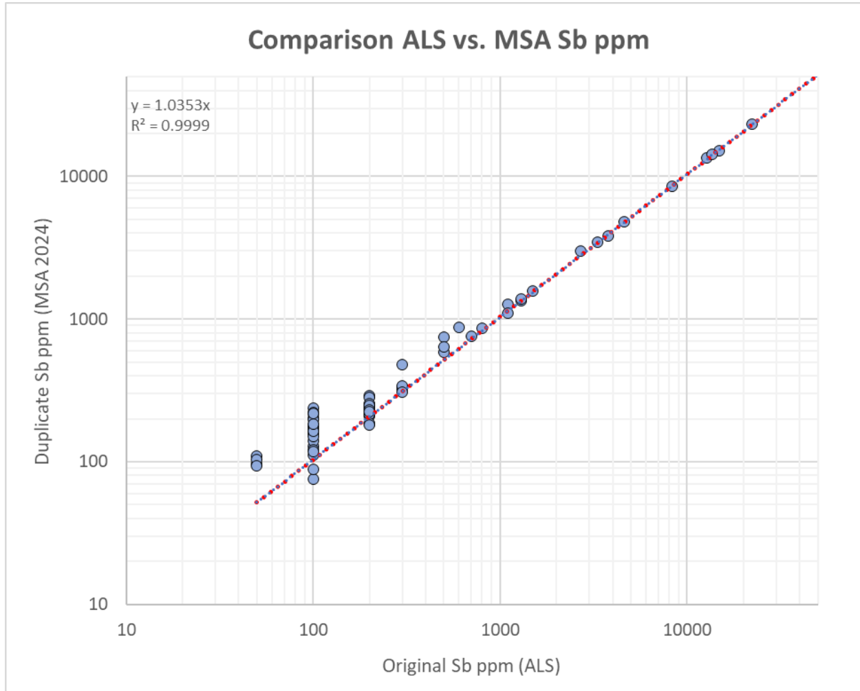
Figure 11-6 Historical Pulp Re-analysis – Sb (MSA 2024)
