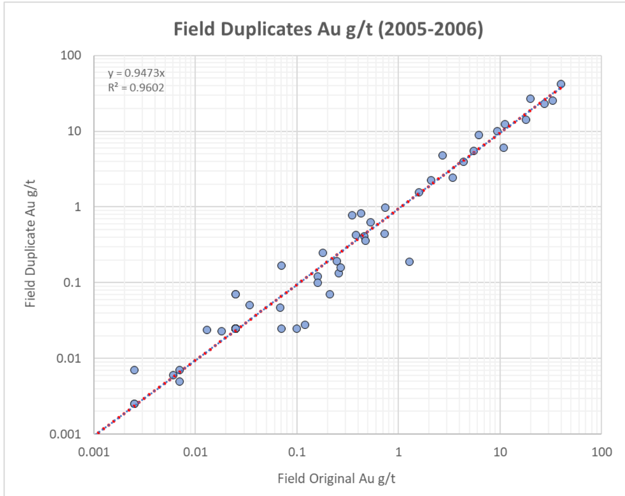
Figure 11-3 Field Duplicate Performance – Au
