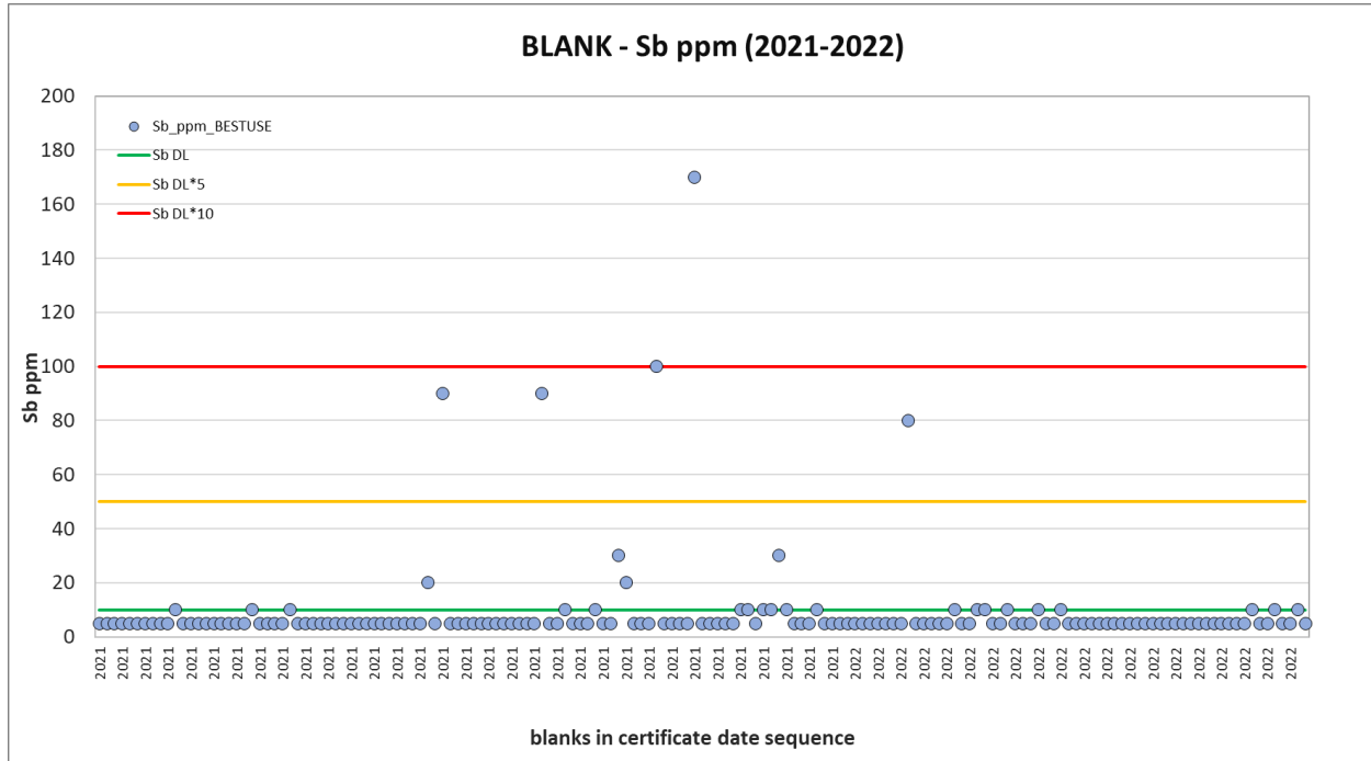
Figure 11-8 Blank Performance 2021-2022 - Sb
