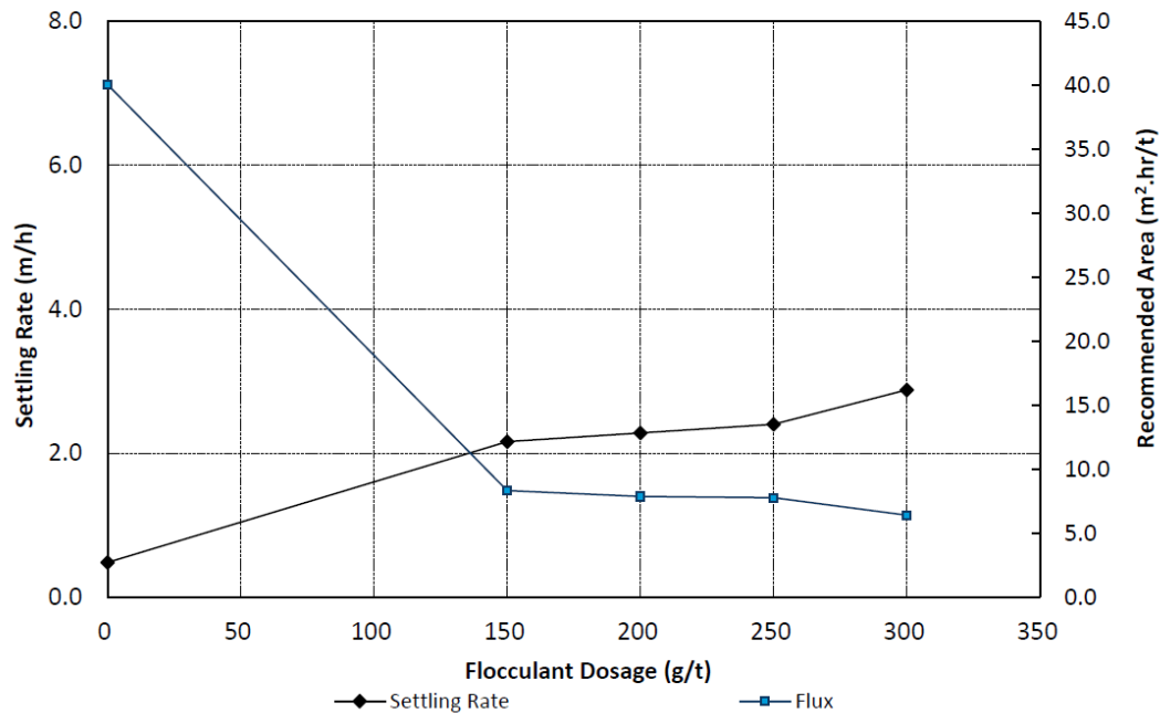
Figure 13-5 Slurry Settling Tests on BIOX™ Products (Outotec RS (PTY) LTD, 2018)
