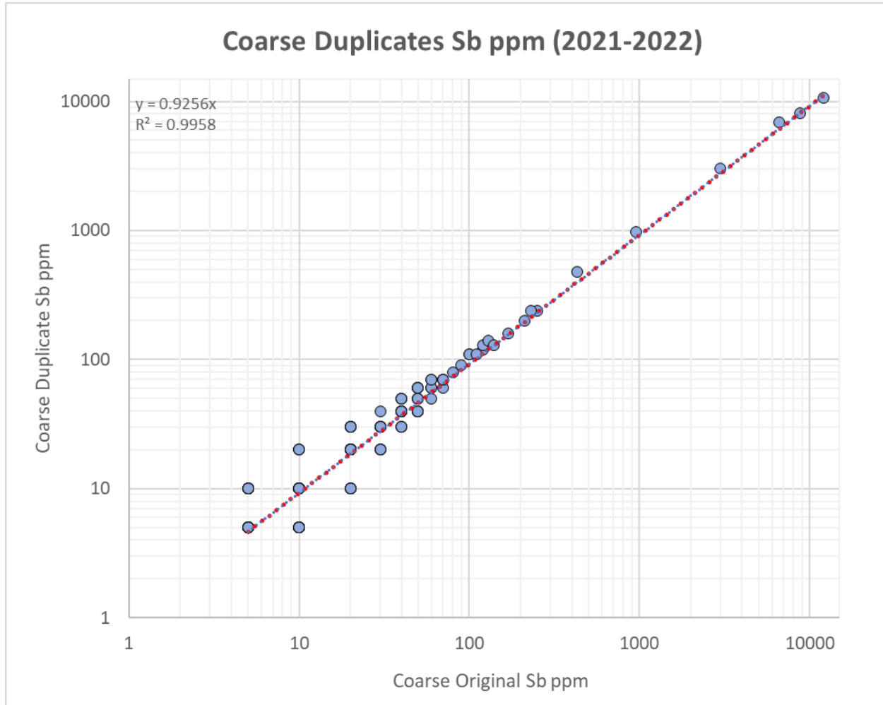
Figure 11-10 Coarse Duplicate Performance 2021-2022 - Sb
