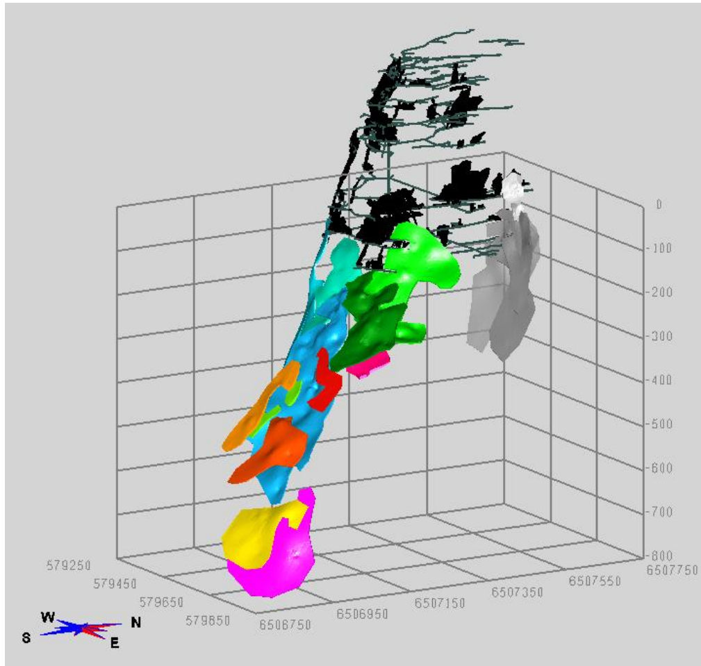
Figure 14-1 Three-dimensional View – Veins and Existing Underground
