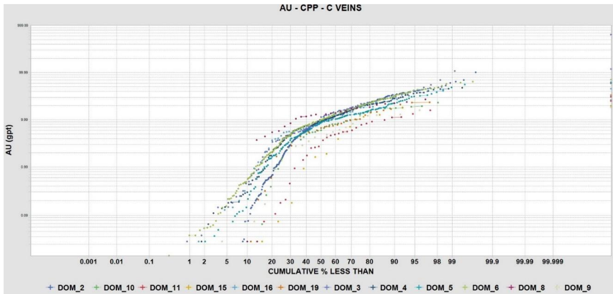
Figure 14-2 Gold Grade (g/t) by Domain – “C” Veins
