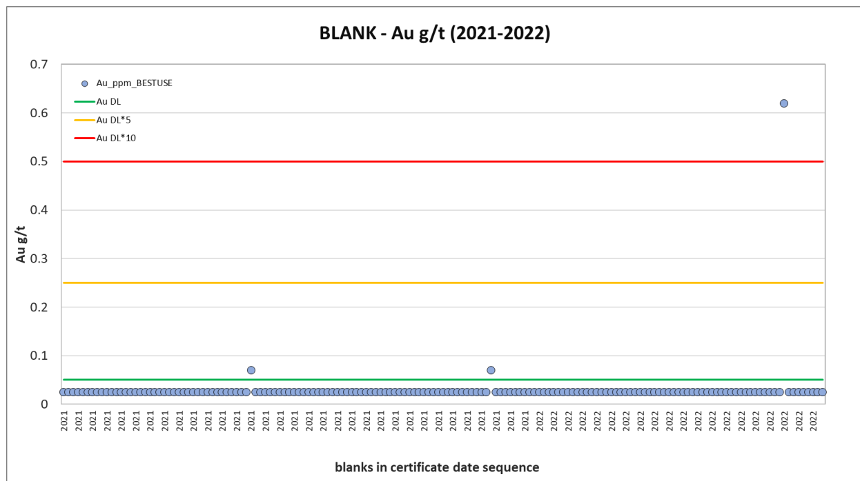
Figure 11-7 Blank Performance 2021-2022 - Au
