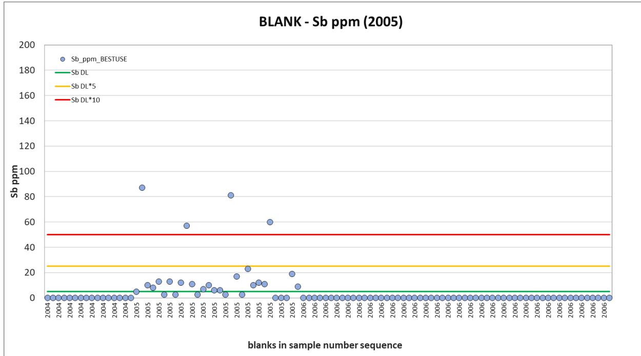
Figure 11-2 Blank Performance 2005 - Sb
