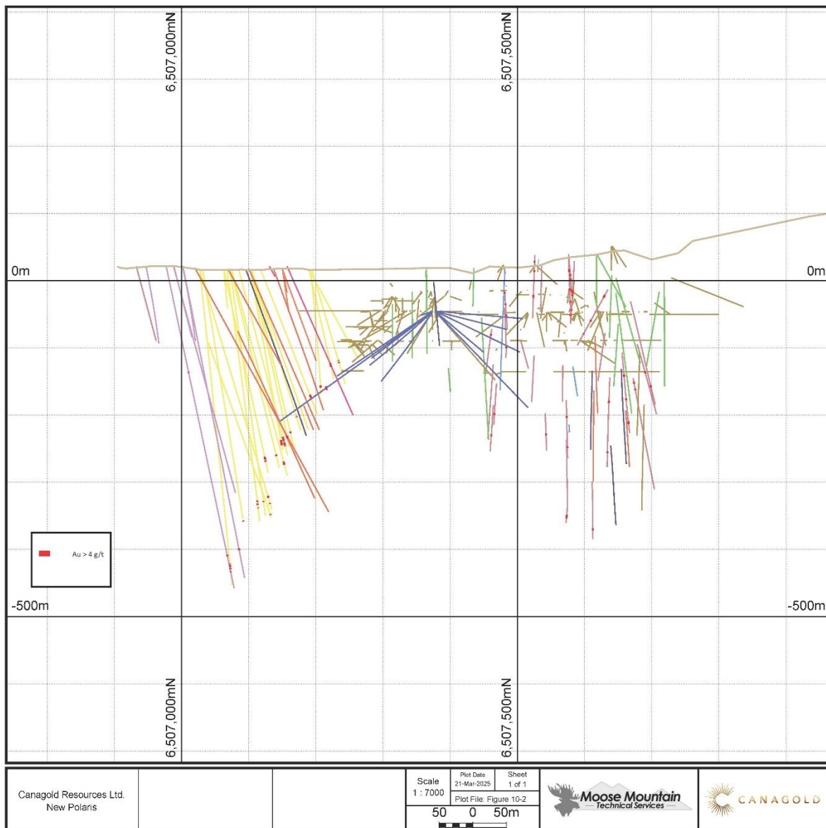
Figure 10-2 Section of the Drillholes and Gold intercepts > 4 g/t. Section depth +/- 50m.
