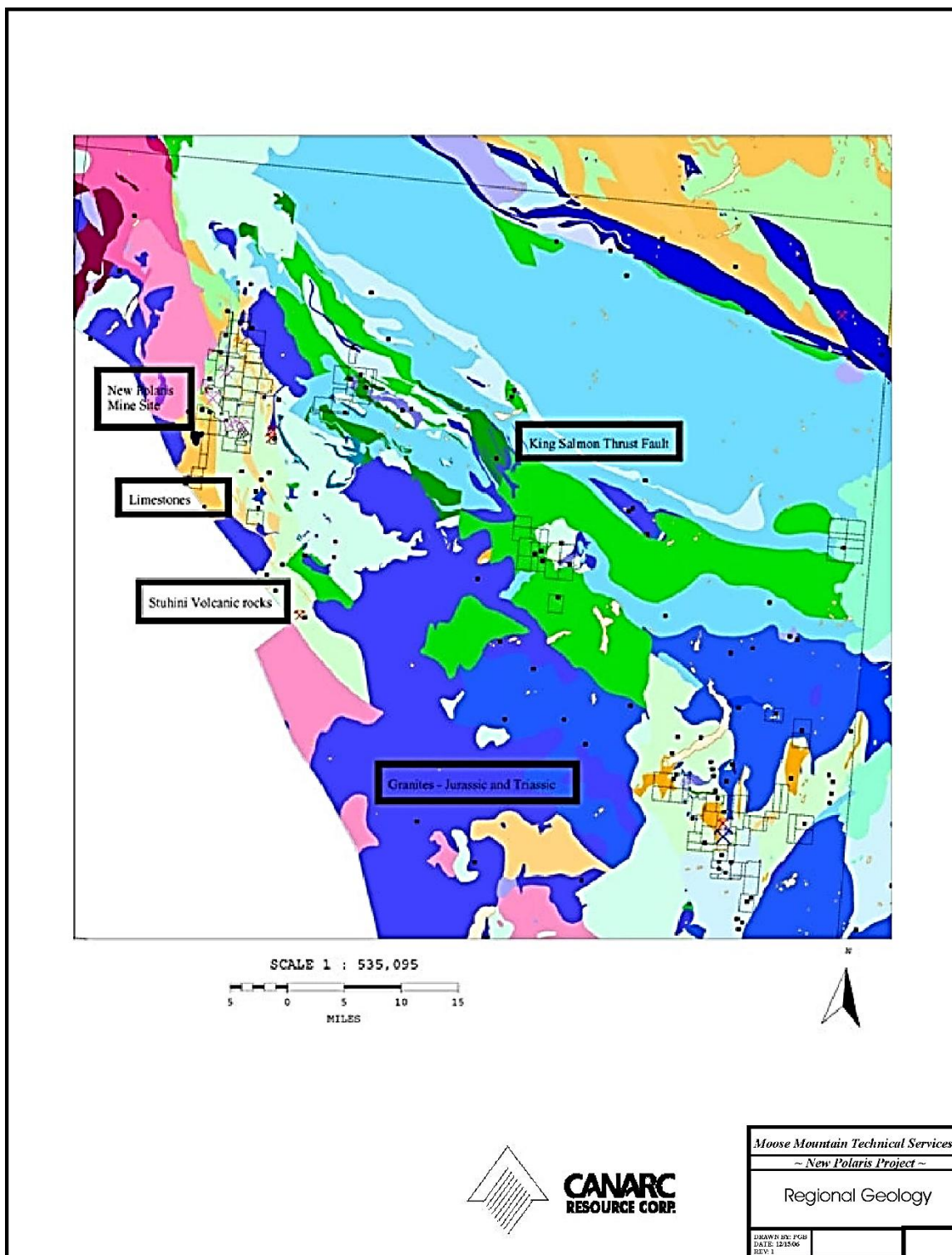
Figure 7-1 Regional Geology
