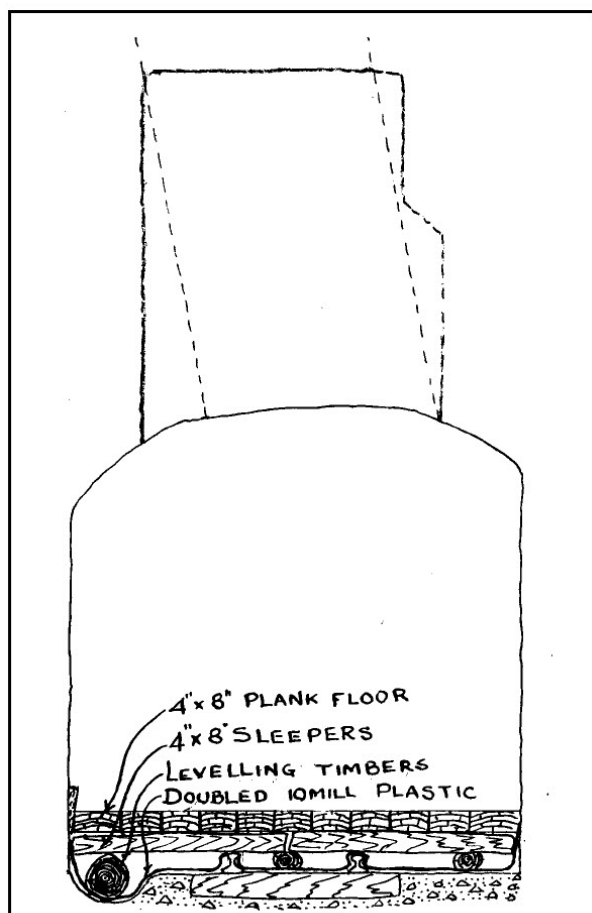
Figure 11.2: Flooring arrangement for bulk sample collection
