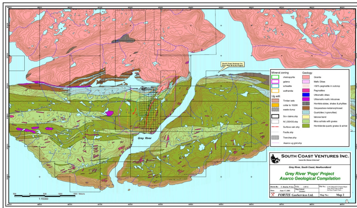
Figure 8.1: Grey River Regional Geology Deposit Types
