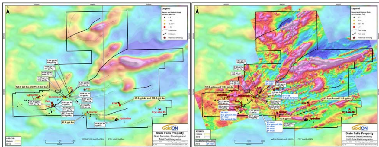
Figure 4 – Includes overlays of historical data and preliminary interpreted fold axis and limbs
