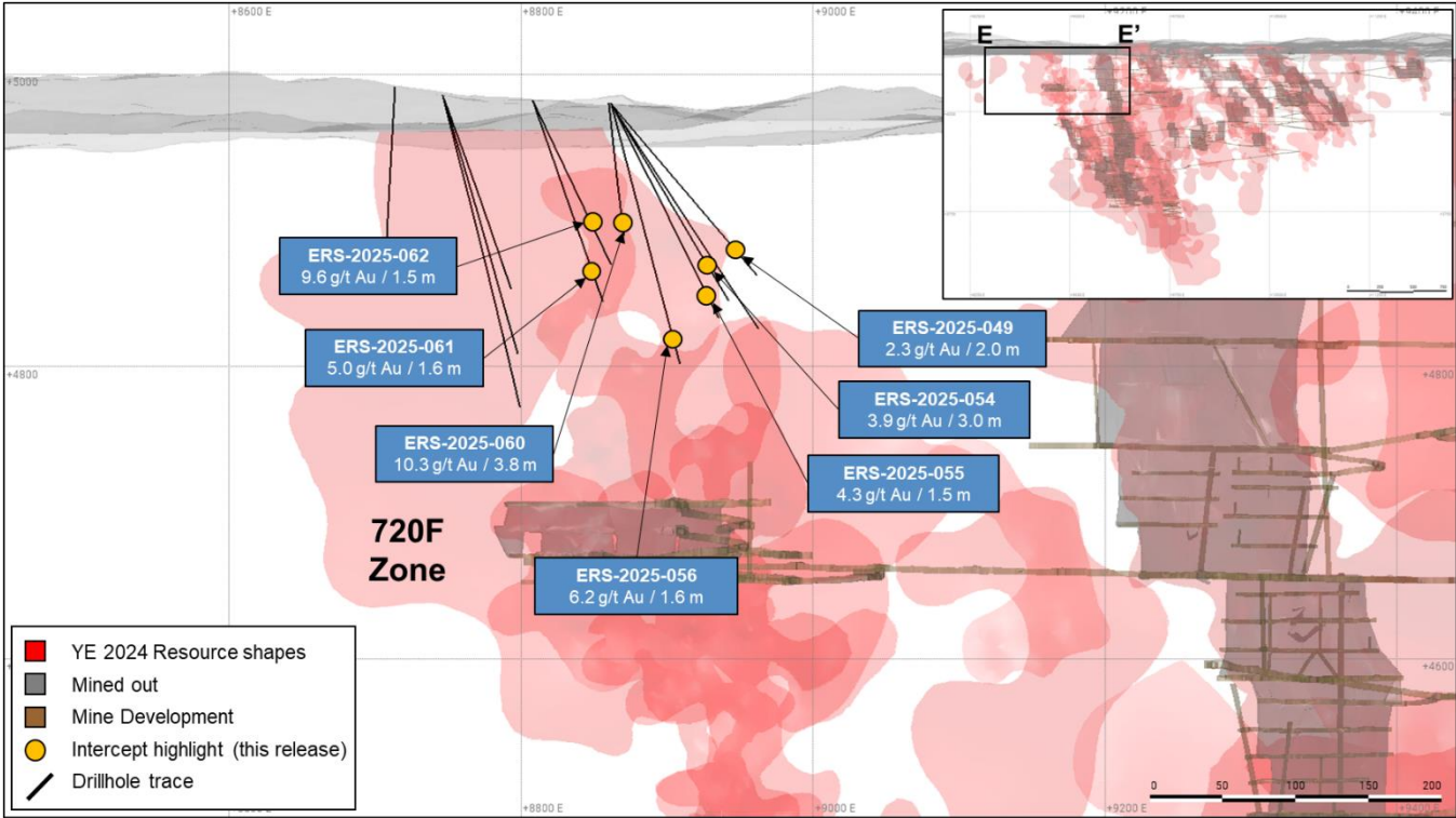
Figure 7: Falcon 720 Zone Long Section Looking North
