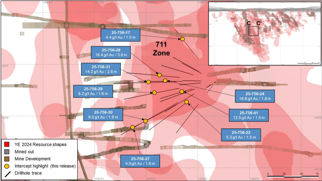
Figure 5: 711 Zone Long Section Looking North
