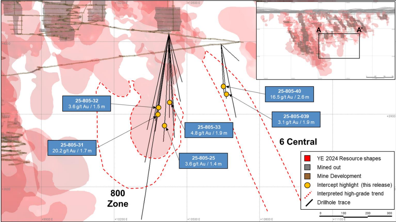
Figure 3: 6 Central Zone and 800 Zone – Long Section Looking North
