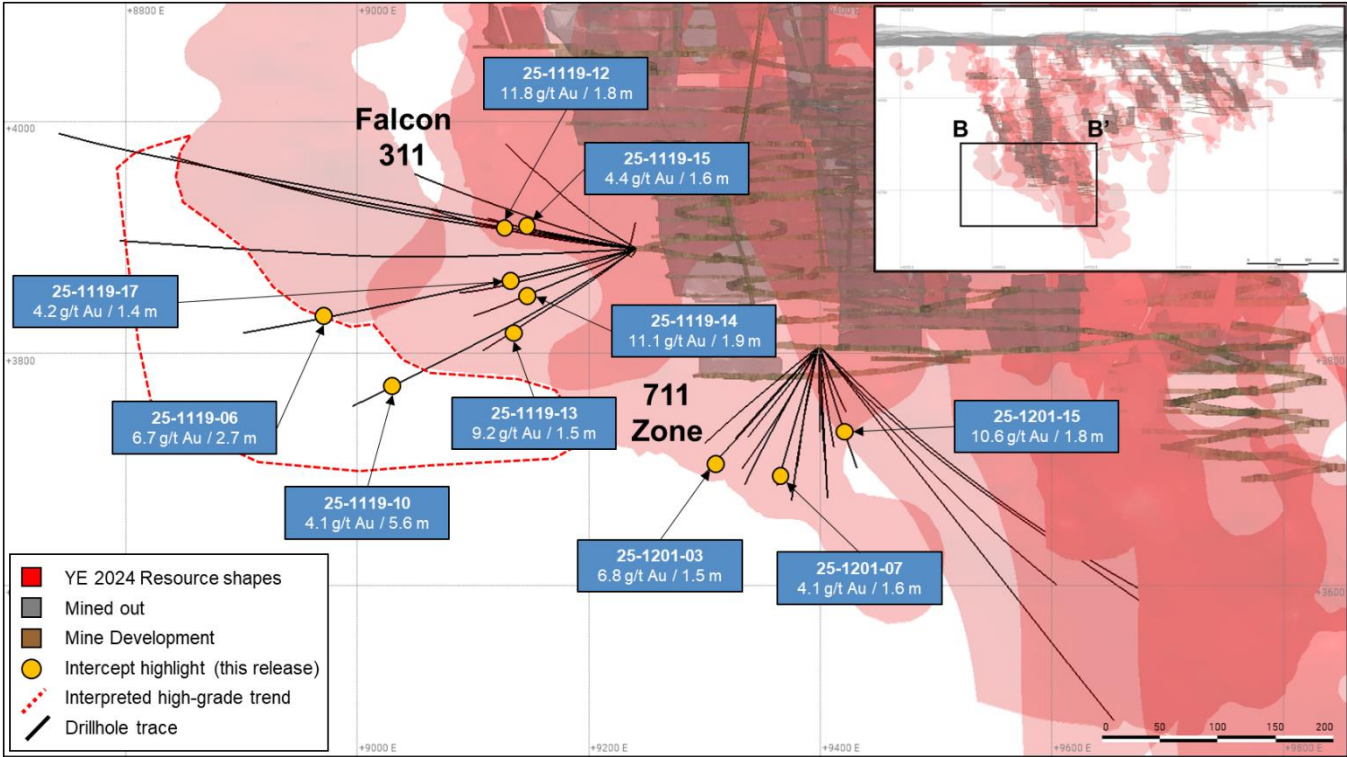
Figure 4: Falcon 311 and 711 Zones Long Section Looking North
