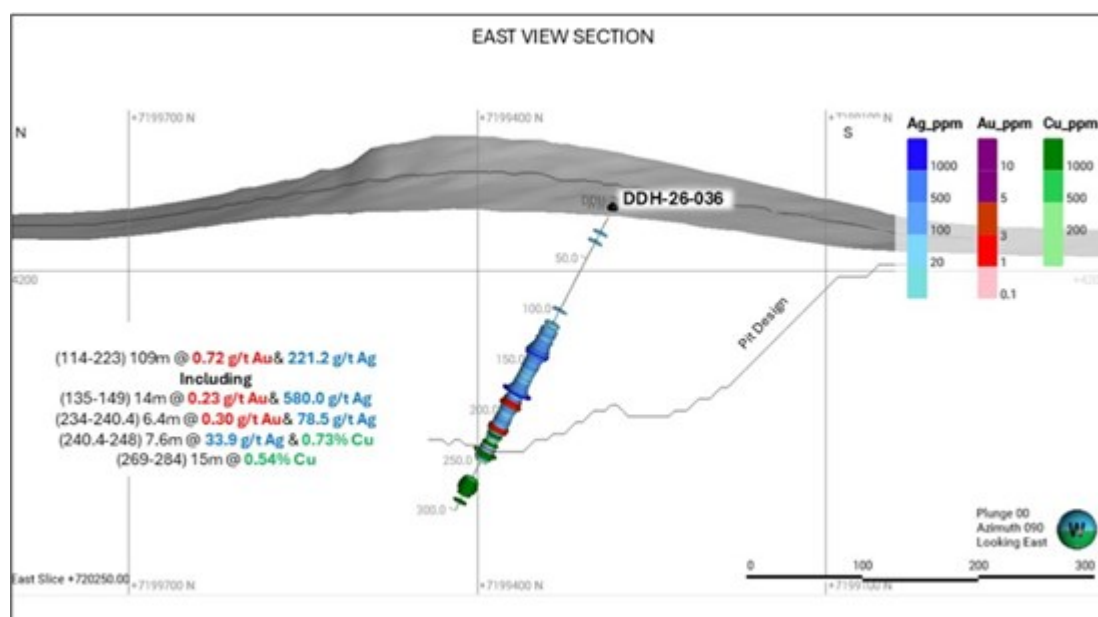
Figure 2 - Cross-Section Through Hole DDH 26-036 at Oculito West
