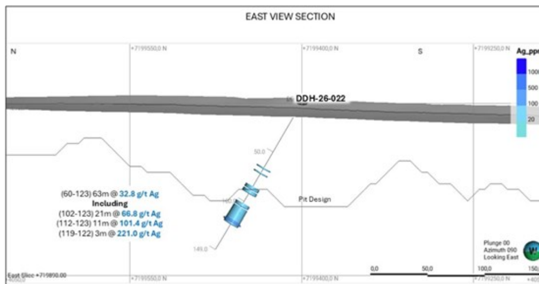
Figure 3 - Cross-Section Through Hole DDH 26-022 at JAC / Oculito
