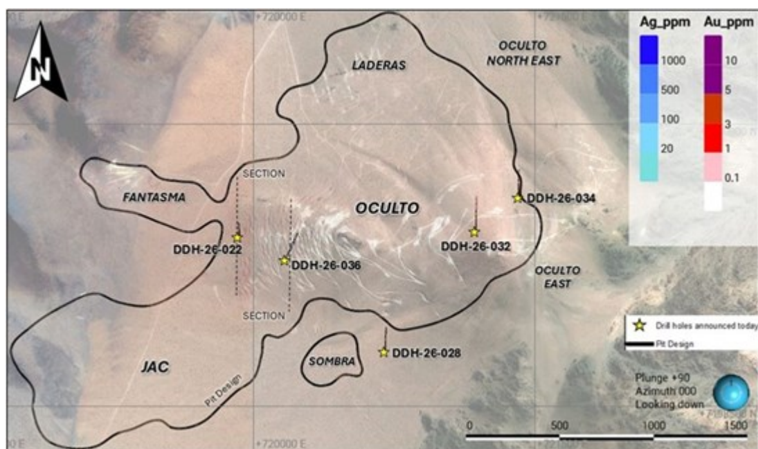
Figure 1 - Plan View of Drill Results
