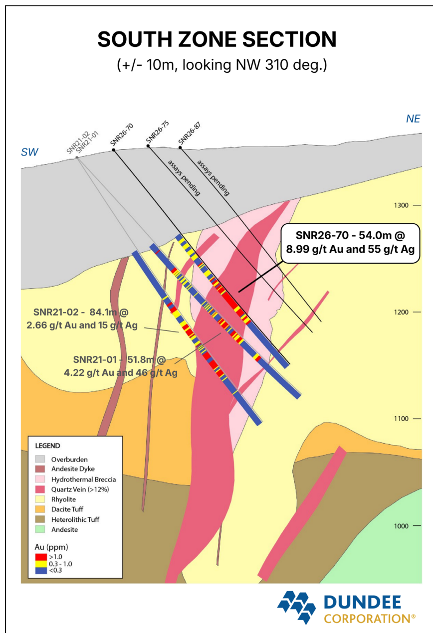
Figure 2 – South Zone Cross Section
