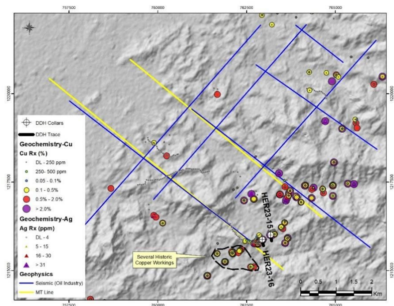
Figure 2. AM drill locations, MT and seismic lines.
