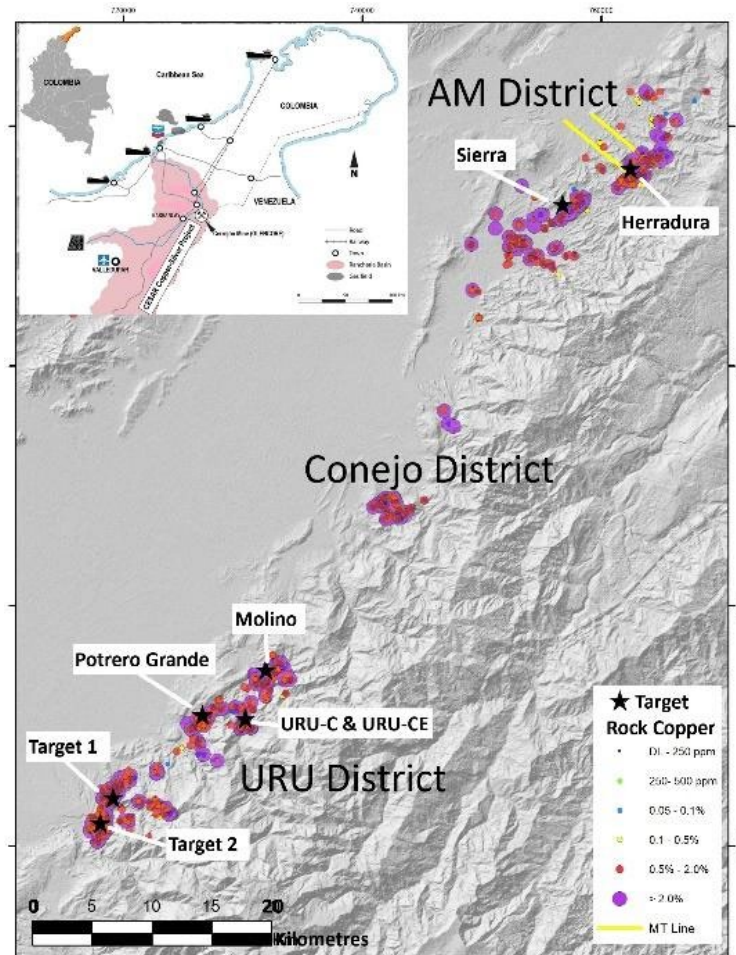
Figure 1. CESAR priority targets.
