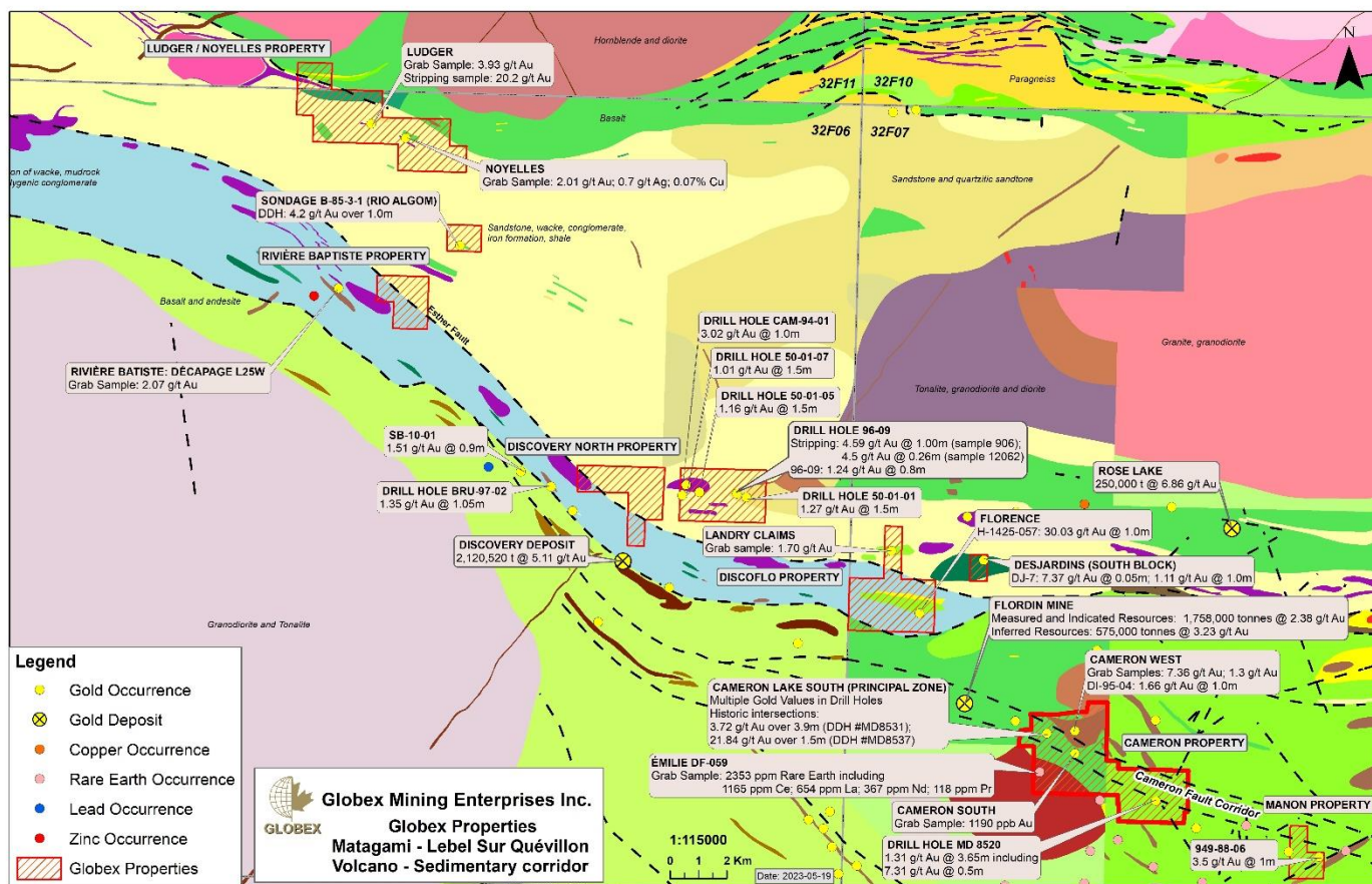
Cameron Fault Corridor Area Geology Map (Figure 1 of 2)
