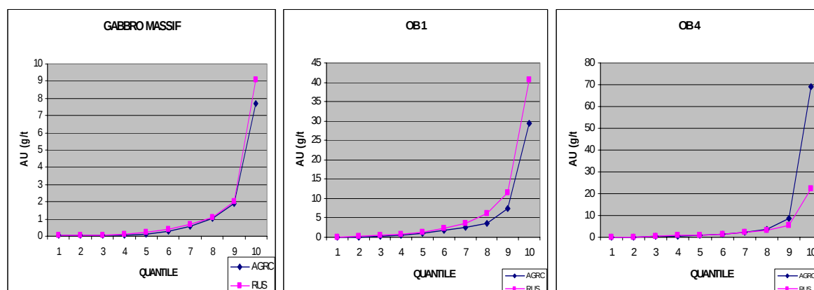
Figure 17.3: Comparison of Grade Distributions for Soviet and AGRC Drilling for Gabbro Massif and Orebodies 1 and 4
