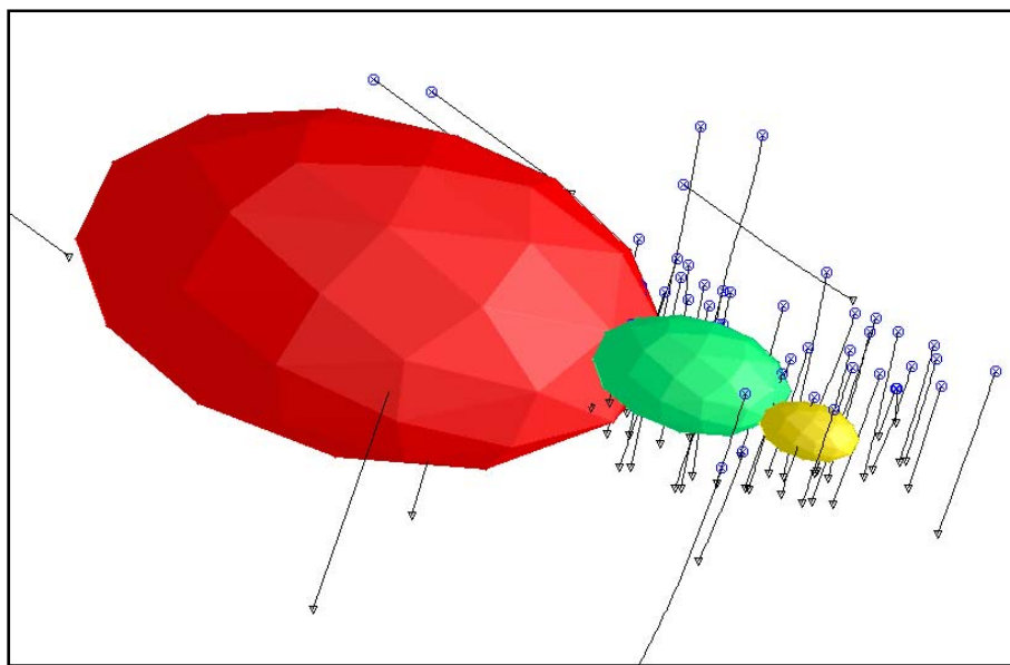
Figure 16.11 –Different Search Ellipsoids Used for the Interpolation Process
