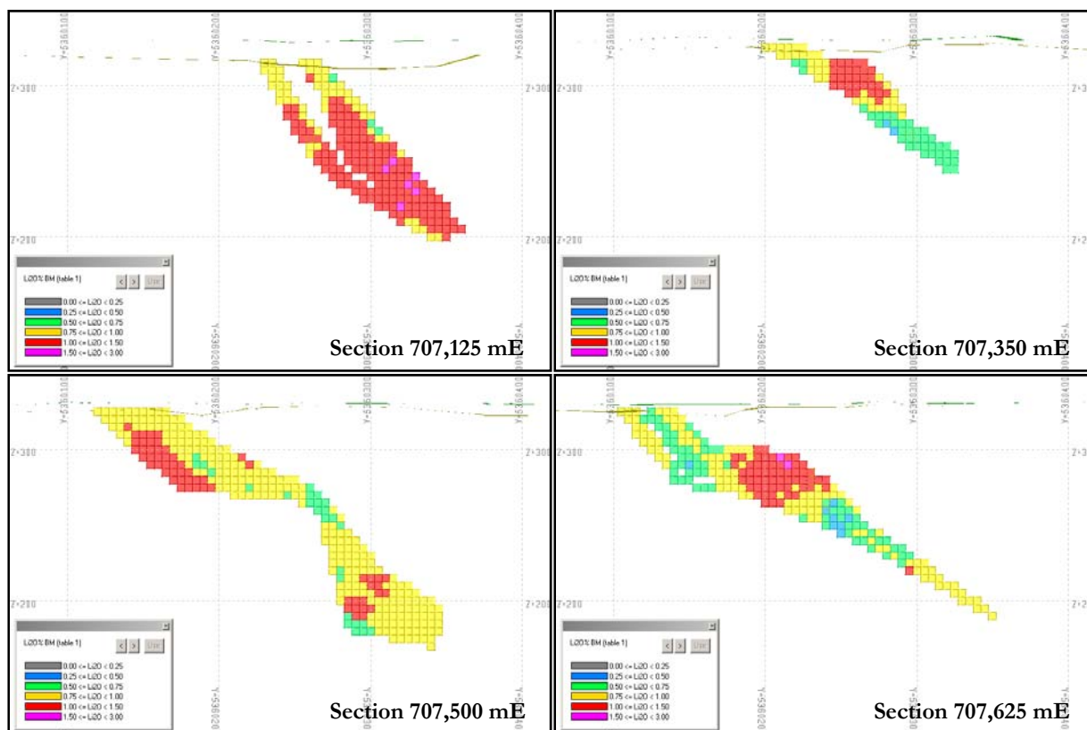
Figure 16.12 – Section Views Showing Block Model Interpolation Results (Looking West)
