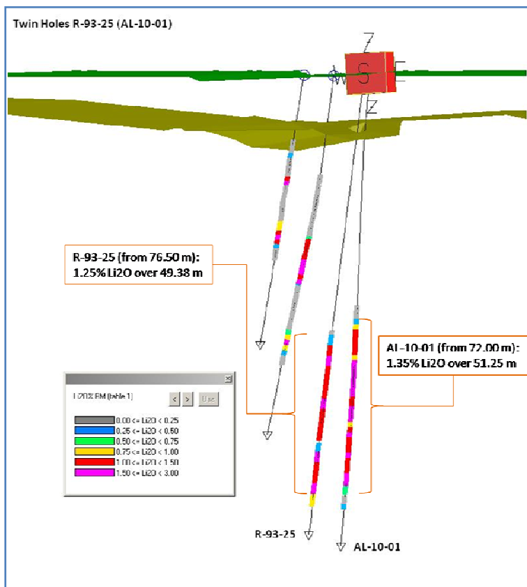
Figure 13.4 – Section Showing Results for Twin Holes AL-10-01 and R-93-25
