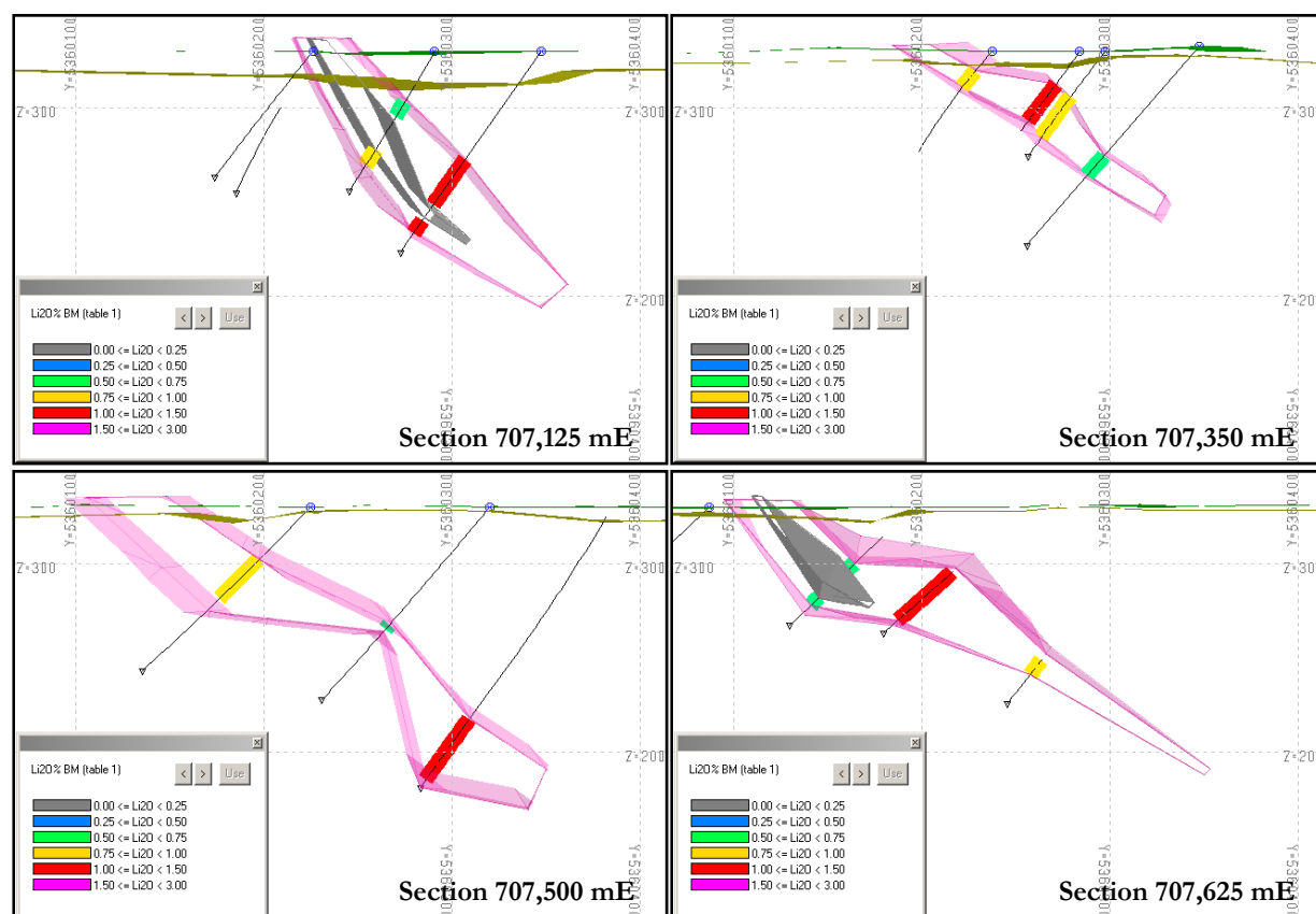
Figure 16.6 – Modeled Envelopes with Mineralised Intervals in Section Views (Looking West)
