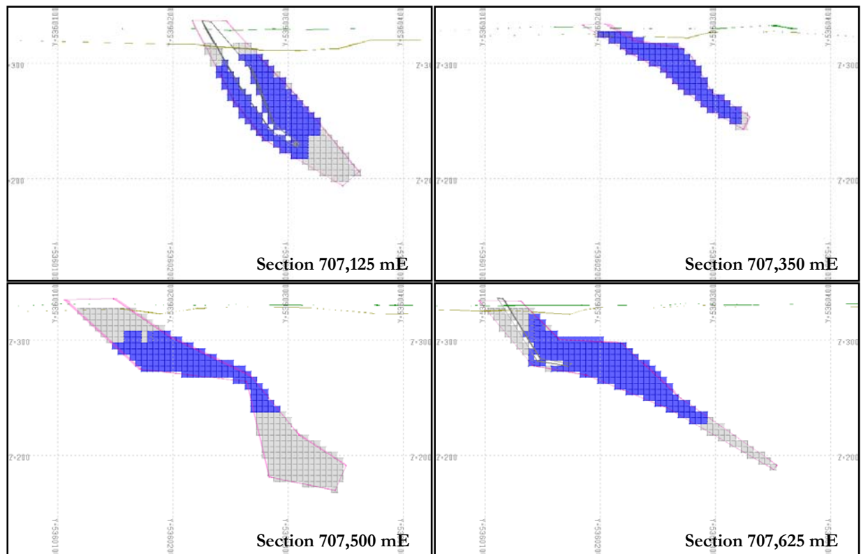
Figure 16.14 – Block Model Classification in Section Views (Looking West)
