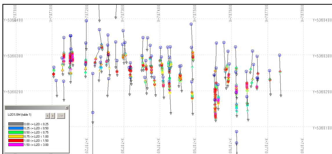
Figure 16.4 - Plan View Showing the Spatial Distribution of the Composites
