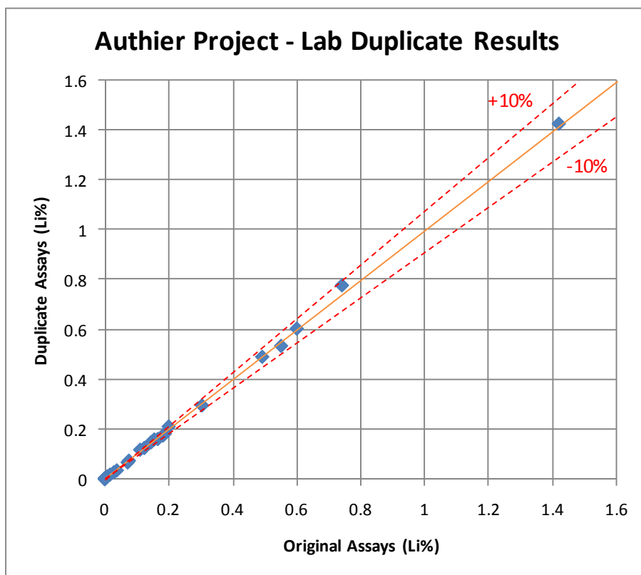
Figure 12.3 – Correlation Plots for the Laboratory Pulp Duplicates
