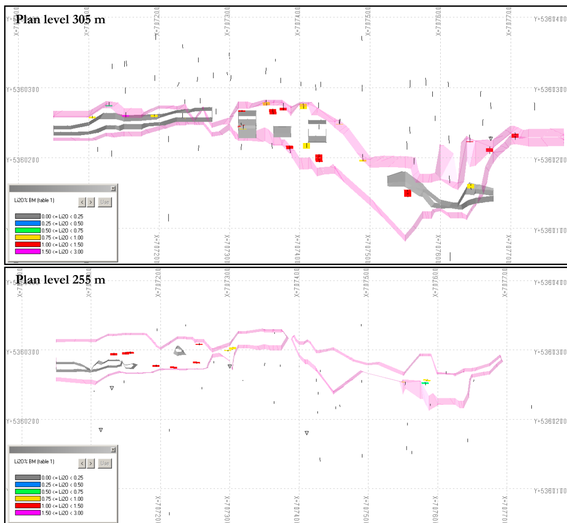
Figure 16.7 – Modeled Envelopes with Mineralised Intervals in Plan Level Views
