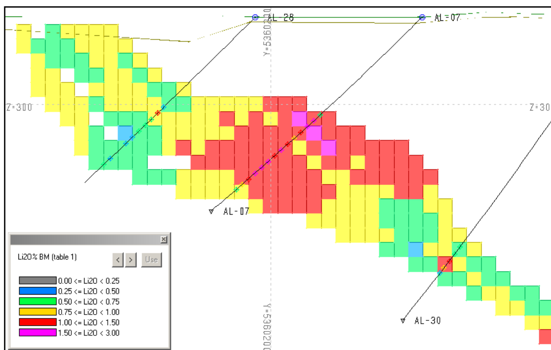
Figure 16.16 – Example of Visual Validation between Composites and Block Model Data
