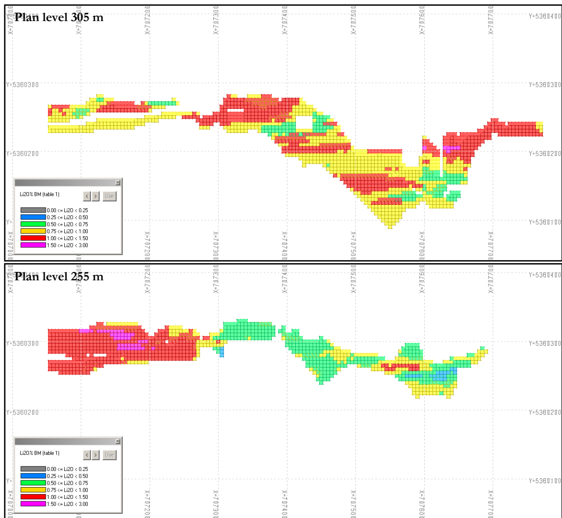
Figure 16.13 – Plan Level Views Showing Block Model Interpolation Results
