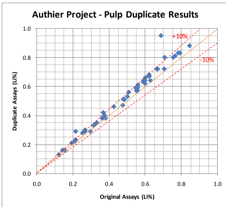
Figure 12.4 – Correlation Plot of the Pulps Re-analysis
