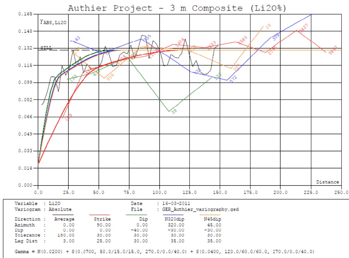
Figure 16.8 – Variograms of Li 2 O Grade of 3 metre Composite
