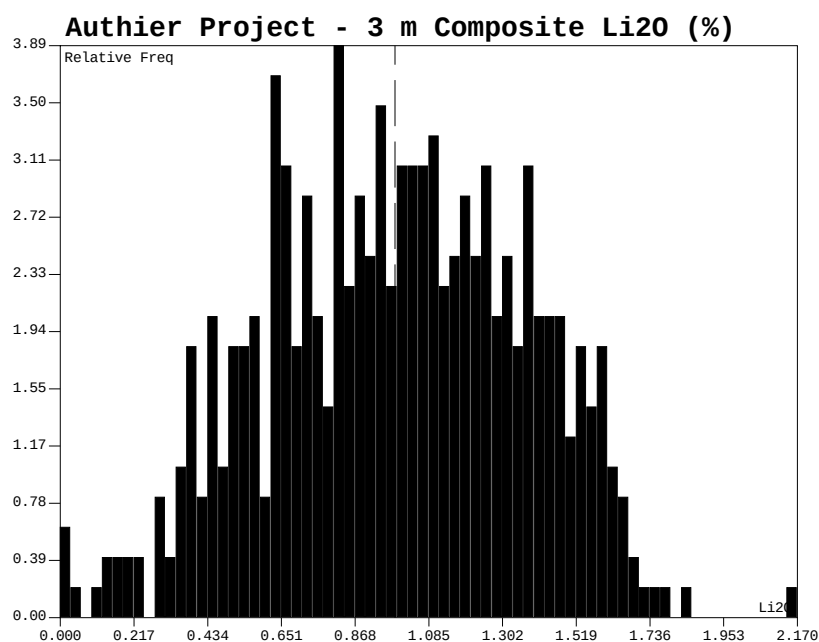
Figure 16.3 – Histogram of 3 metre Composites for Li 2 O
