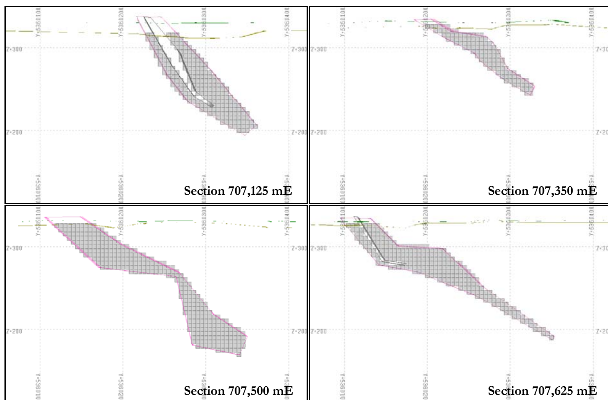
Figure 16.9 – Block Model vs. Mineralised Envelopes in Section Views (Looking West)
