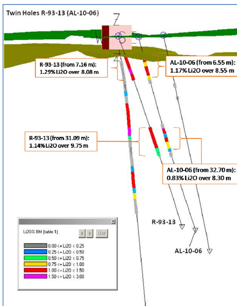
Figure 13.3 – Section Showing Results for Twin Holes AL-10-06 and R-93-13
