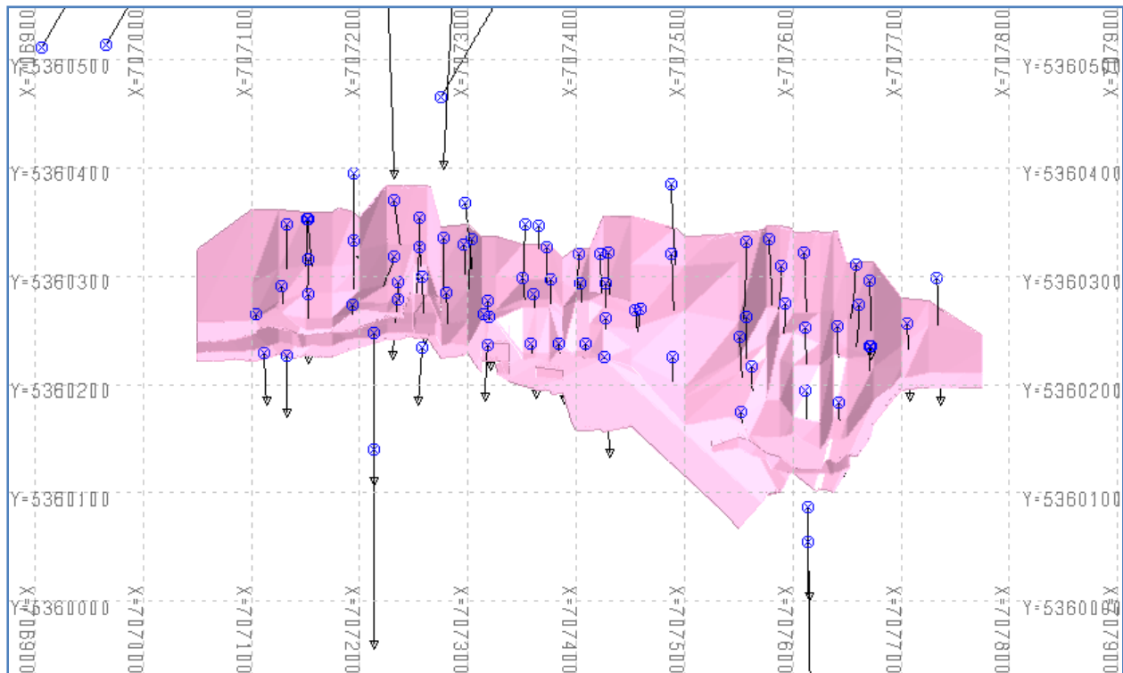
Figure 10.1 – Plan View of the Historical and Recent Drilling in the Vicinity of the Main Pegmatite Intrusion at the Authier Property
