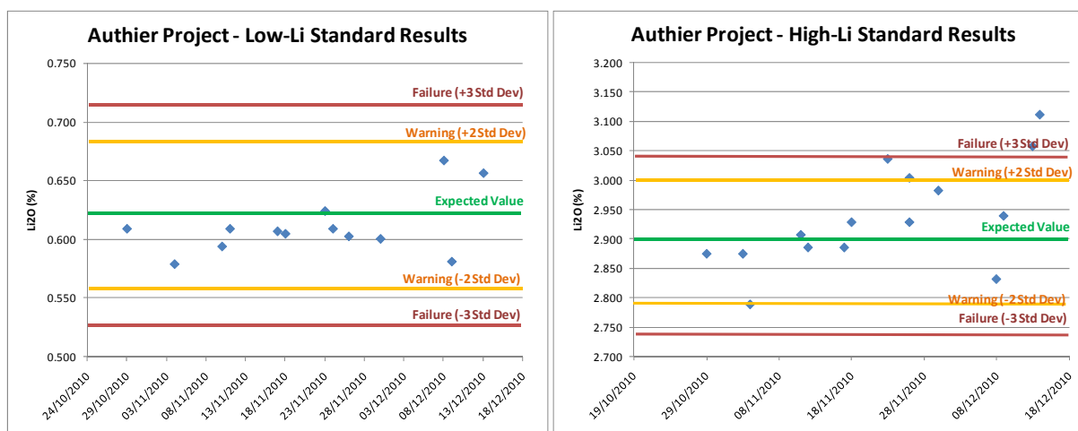
Figure 12.1 – Plots of the Variation of the Low-Li and High-Li Standards with Time
