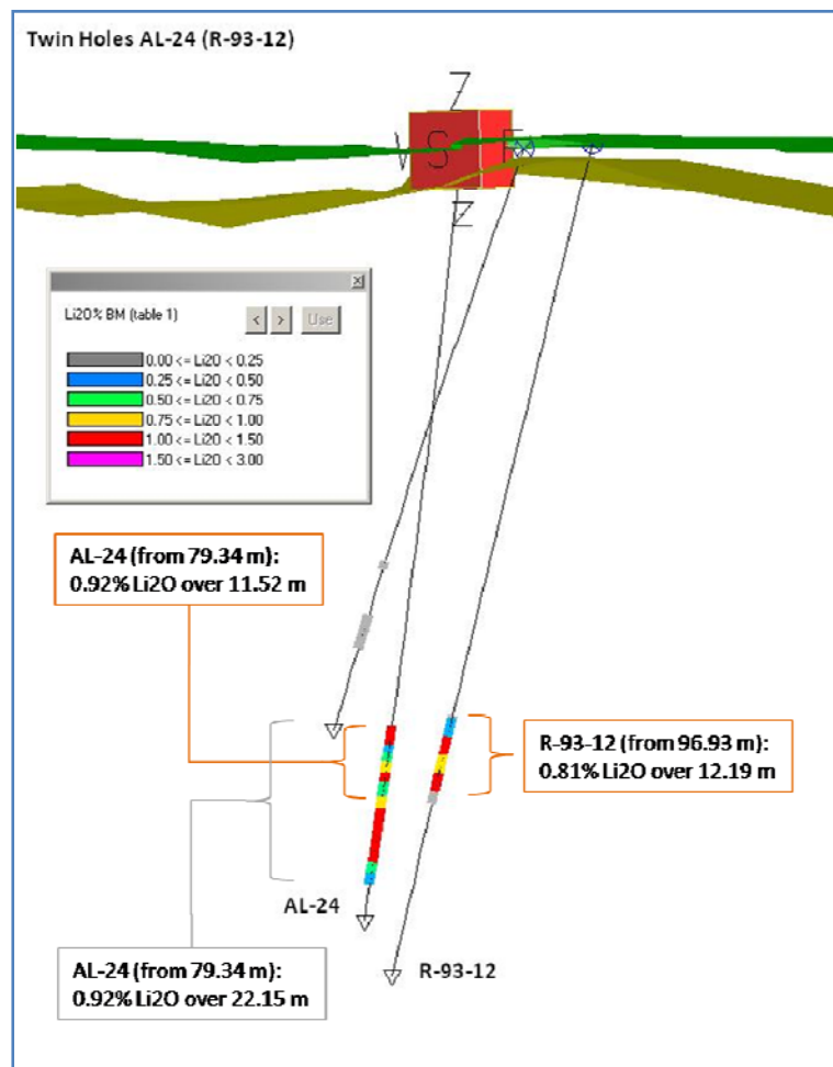
Figure 13.6 – Section Showing Results for Twin Holes R-93-12 and AL-24
