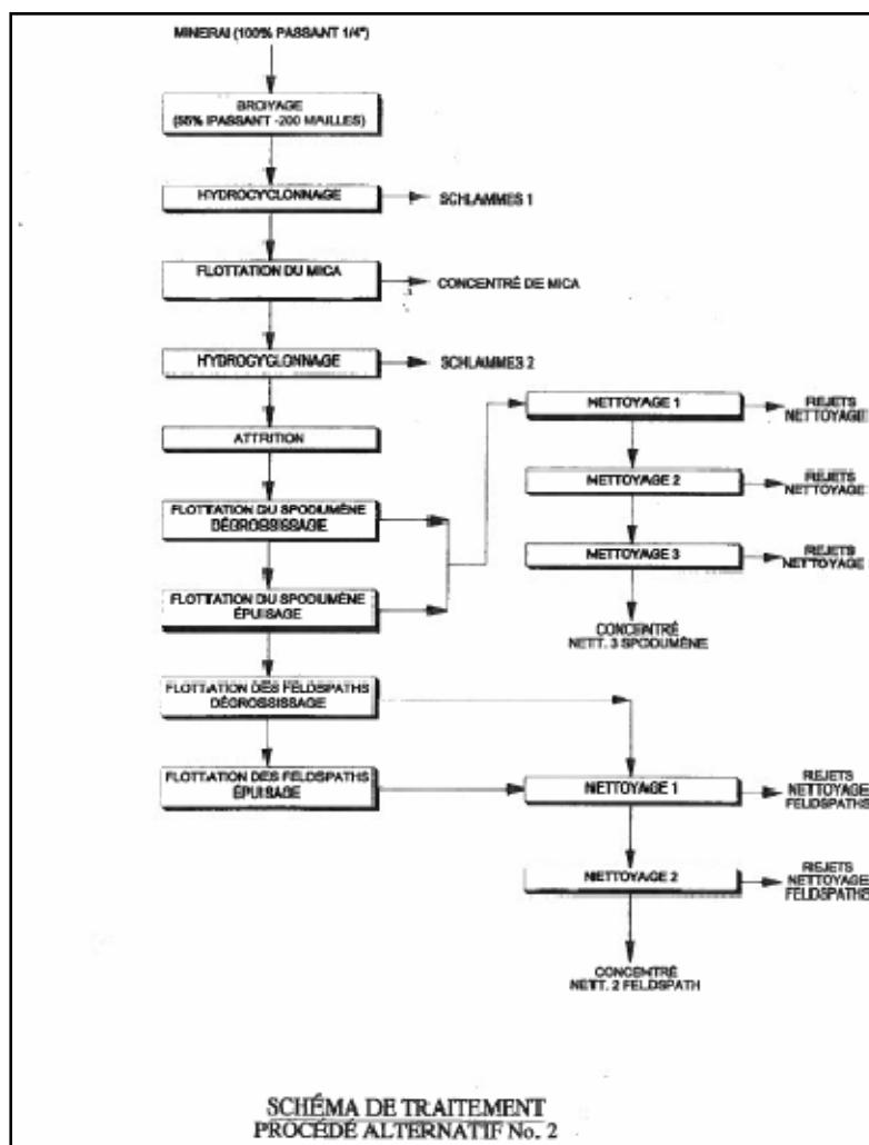
Figure 15.1 –Flowsheet of Alternative Process Number 2 of the 1999 Metallurgical Study
