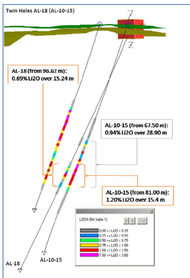
Figure 13.5 – Section Showing Results for Twin Holes AL-10-15 and AL-18
