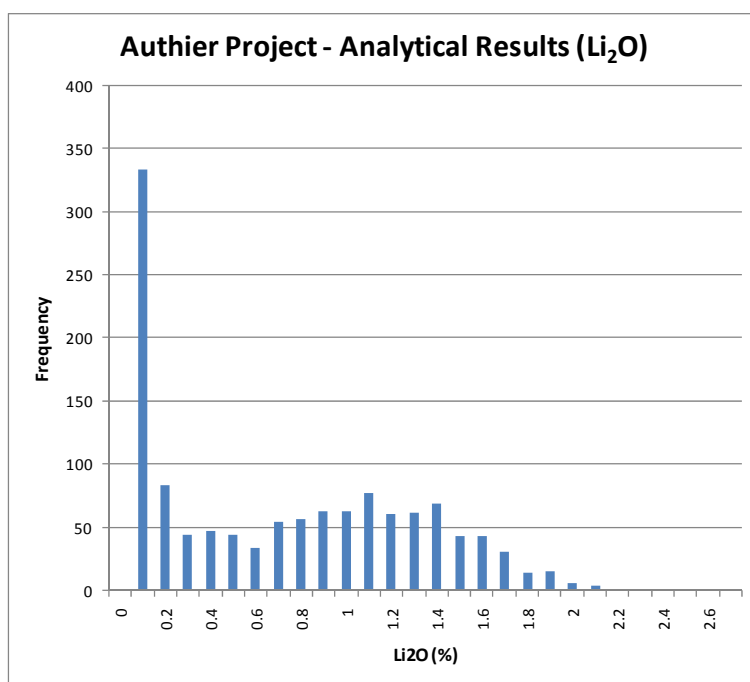
Figure 16.1 – Histogram of the Li 2 O Analytical Data from Authier Database
