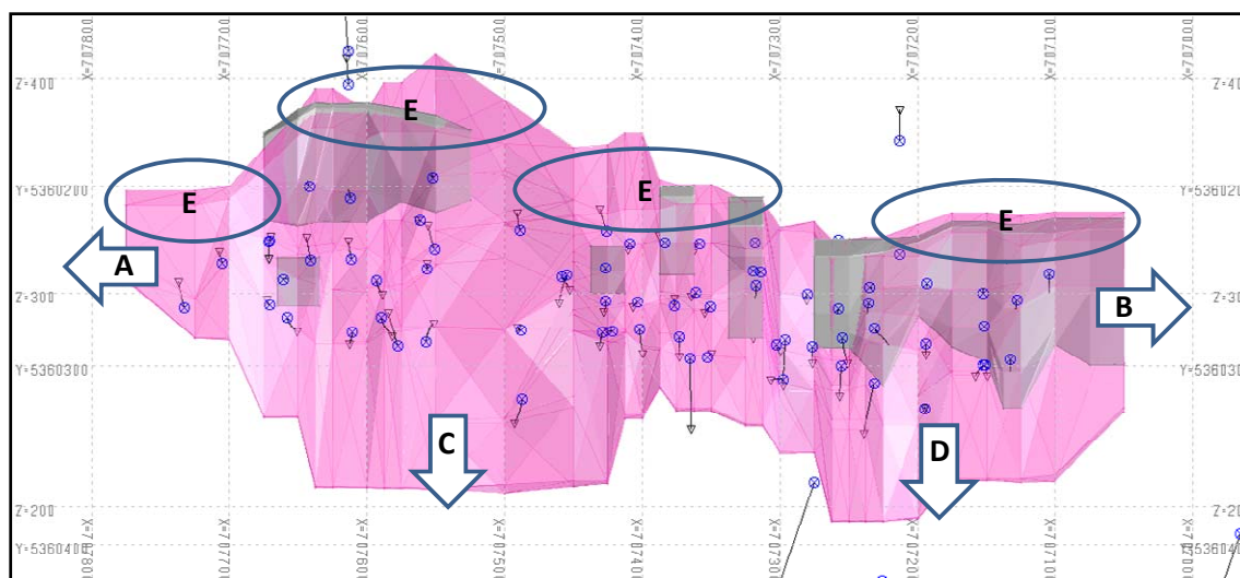
Figure 19.1 – Inclined Longitudinal Section Showing Proposed Drilling Area (Looking South)
