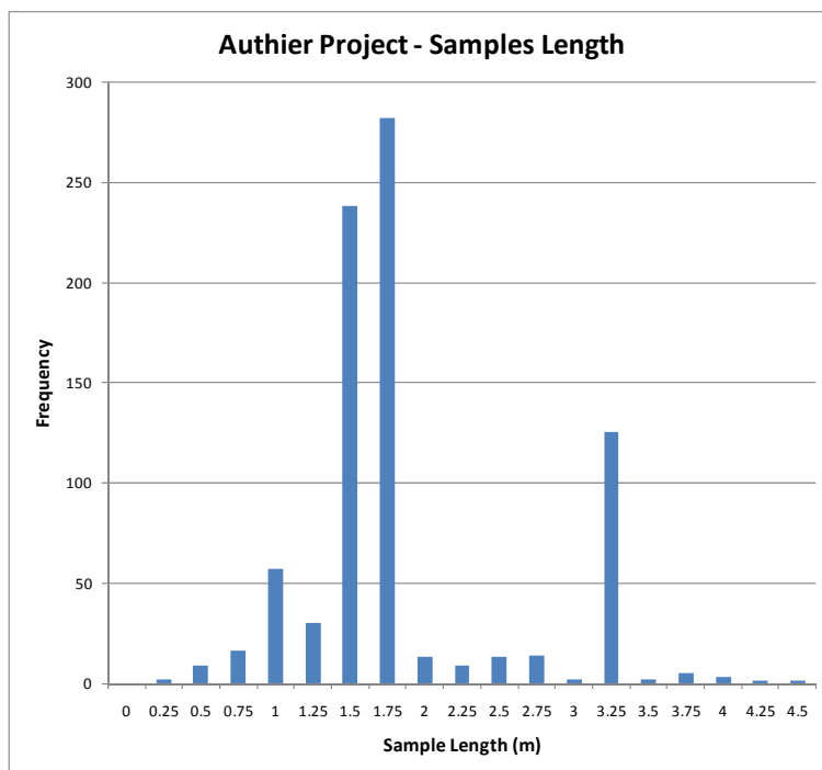
Figure 16.2 – Histogram of Samples Length from Authier Database
