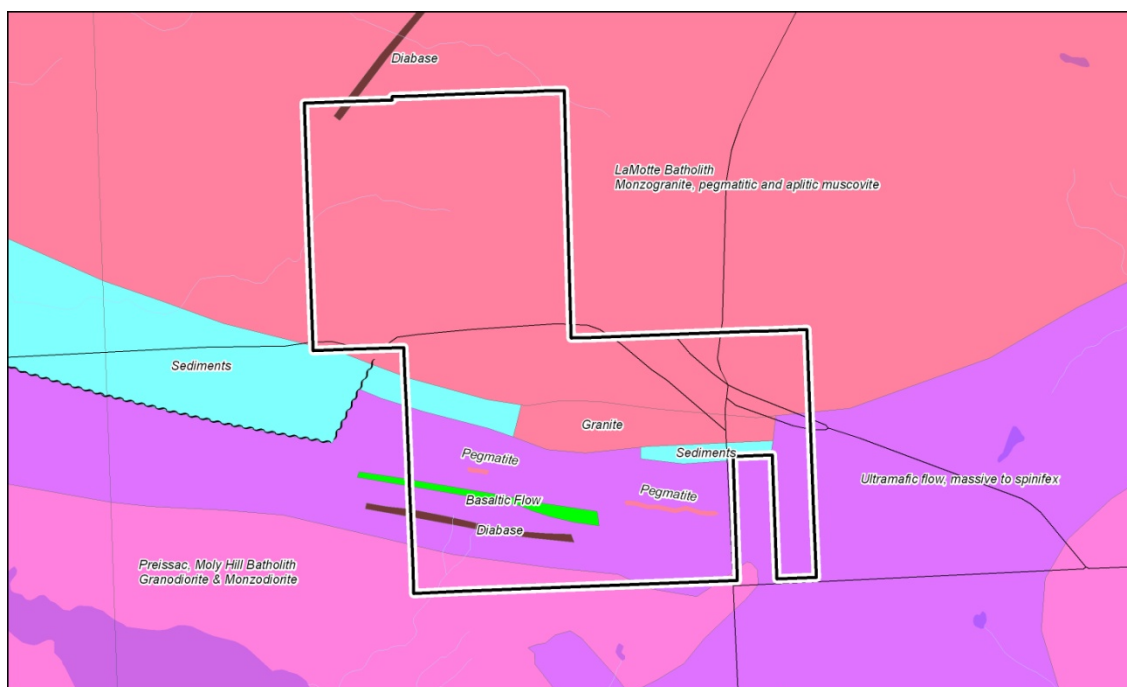
Figure 7.2 – Local Geological Map
