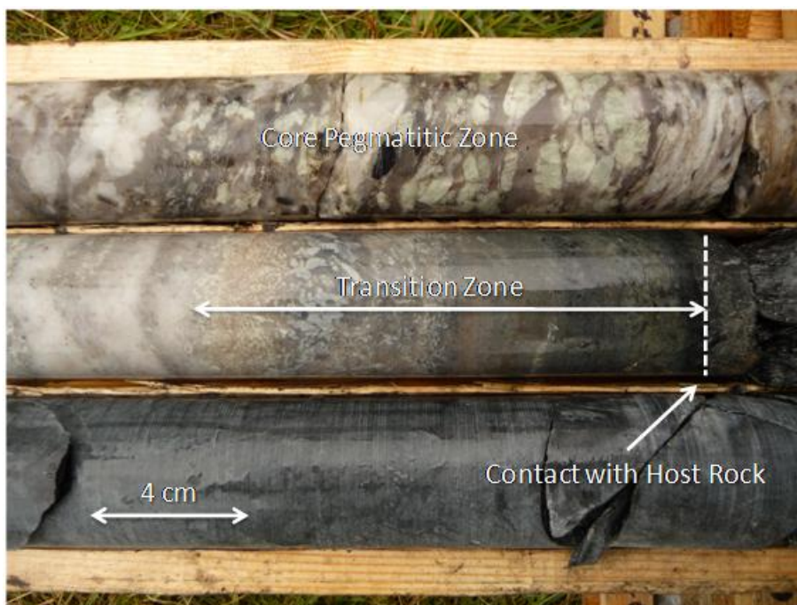
Figure 9.1 – Drill Core from Hole AL-10-03 Showing the Core and Transition Zones
