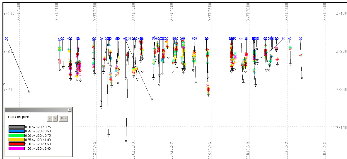
Figure 16.5 – Longitudinal View Showing the Distribution of the Composites (looking north)
