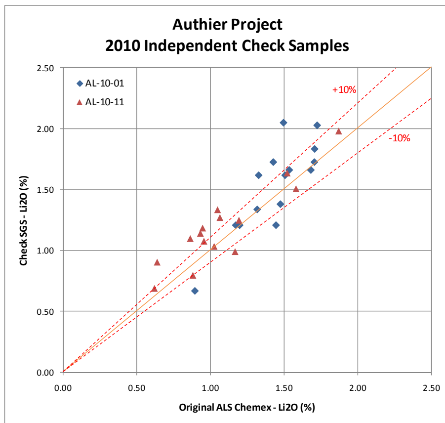
Figure 13.1 – Correlation Plot of Independent Check Samples
