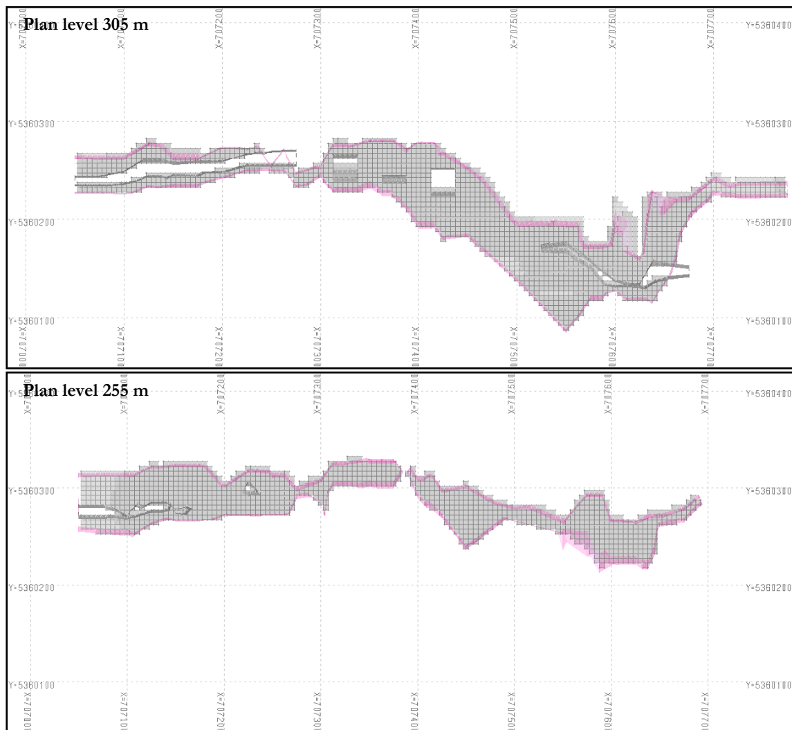
Figure 16.10 – Block Model vs. Mineralised Envelopes in Plan Level Views
