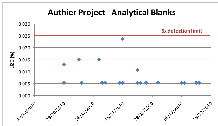
Figure 12.2 – Plot of Variance of Analytical Blanks with Time
