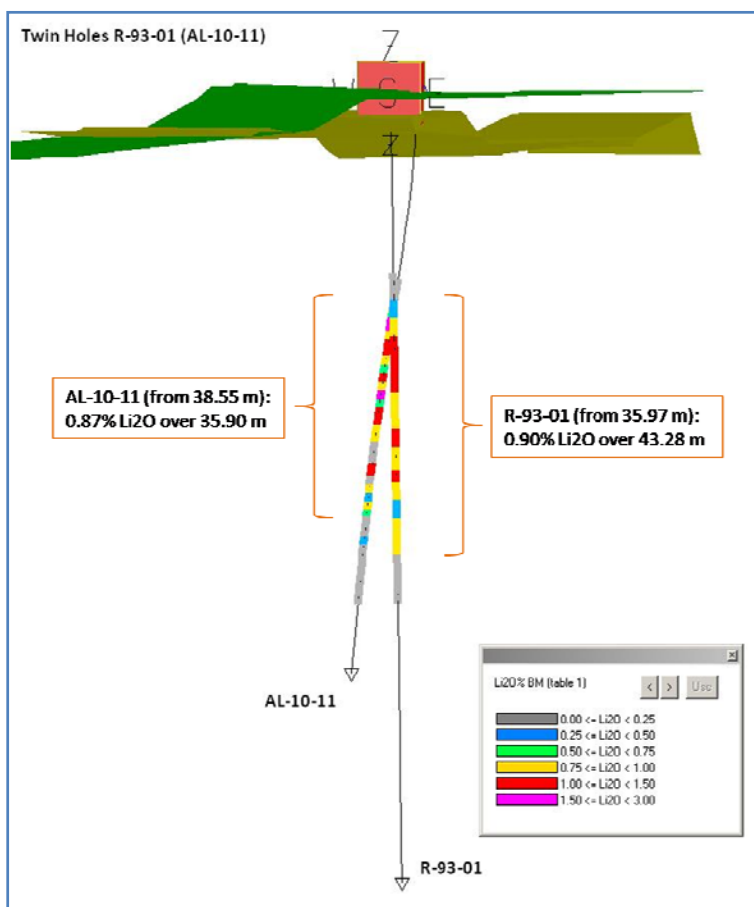
Figure 13.2 – Section Showing Results for Twin Holes AL-10-11 and R-93-01
