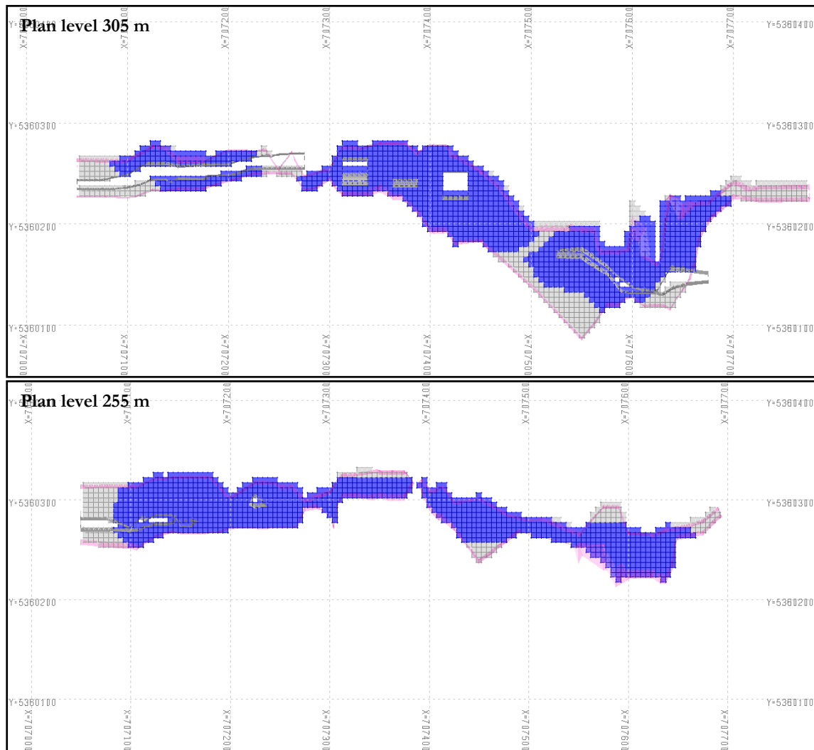
Figure 16.15 – Block Model Classification in Plan Level Views
