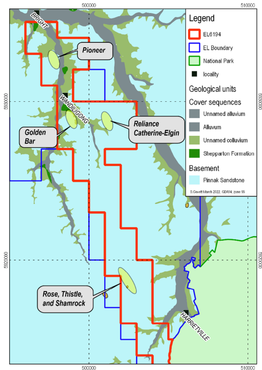
Figure 14; Prospect location map at the Bright project, EL6194.
