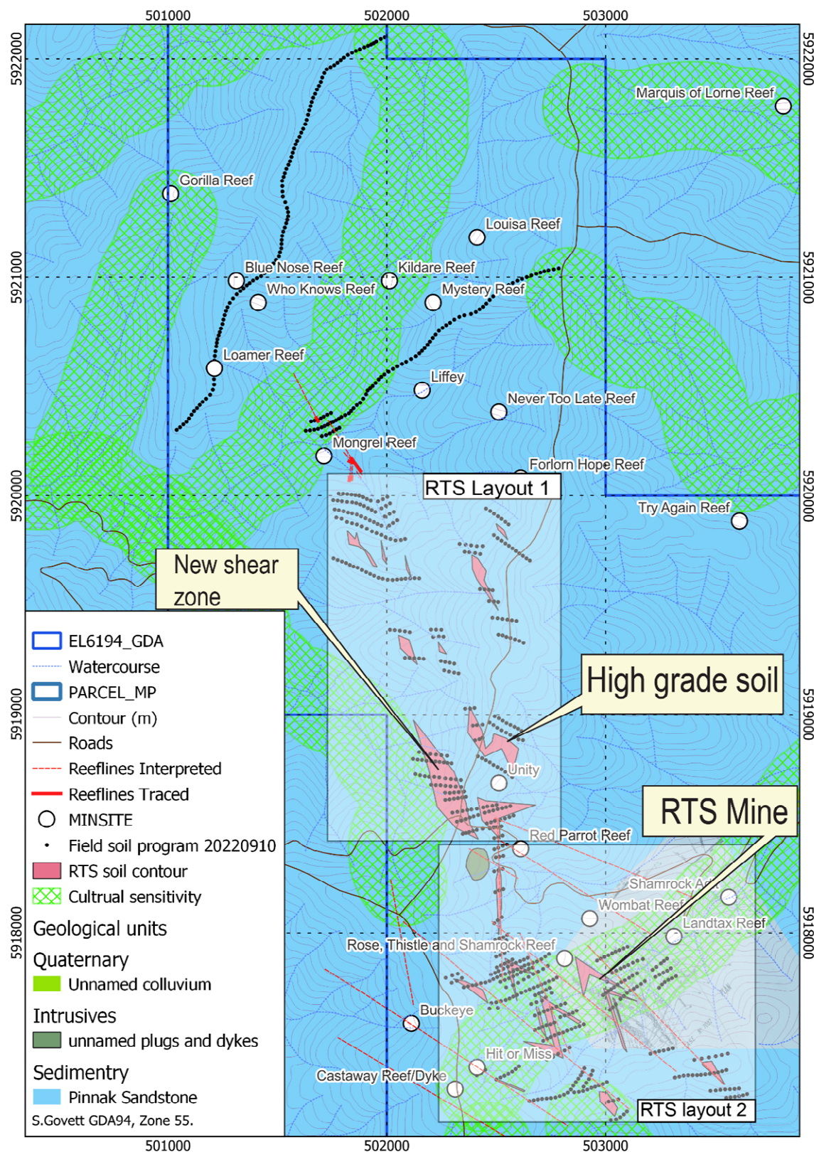
Figure 11; upcoming soil program testing historic and new soil anomalism surrounding and north of the Rose, Thistle, and Shamrock (RTS) Mine.
