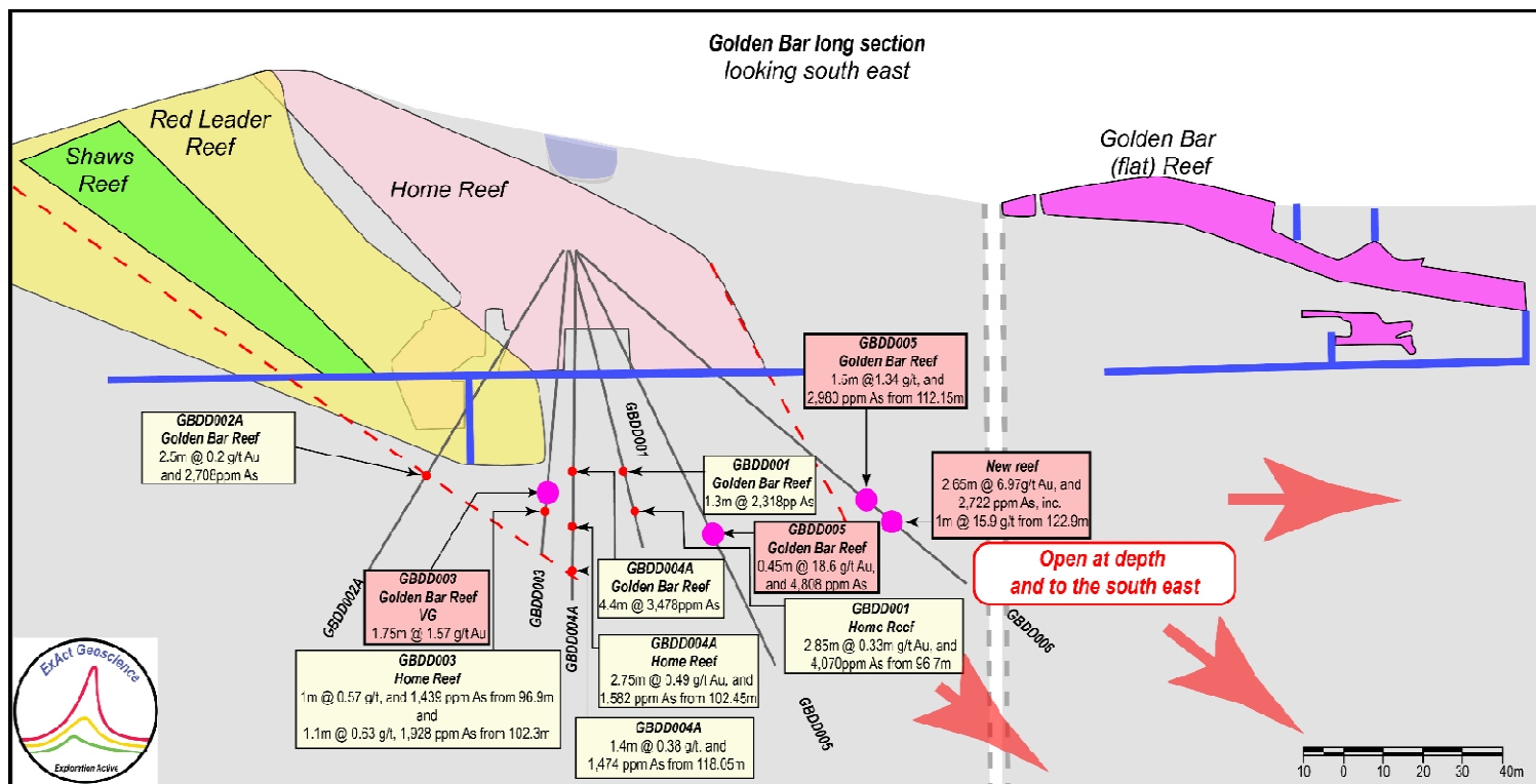
Figure 6; Golden Bar long section, looking north-east. Historic mined areas in colour modified from (Kenny, 1966)
