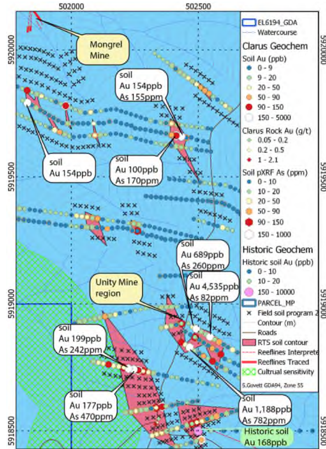
Figure 12; RTS layout 1 , 2022 soil results and planned program north of the RTS mine (left) Note 1,000ppb is equivalent to 1g/t gold.
