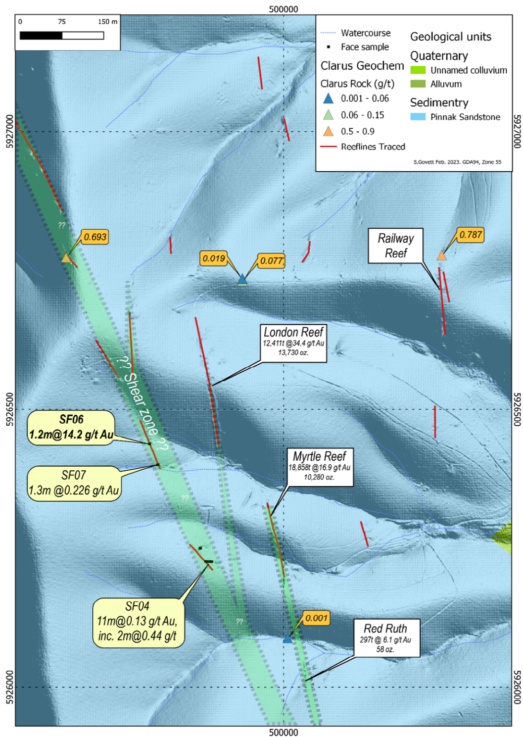
Figure 9; Myrtle Reef mine area. Significant surface geochemistry results and LiDAR surface workings. Potential broad shear-zone shown in green hashed region.
