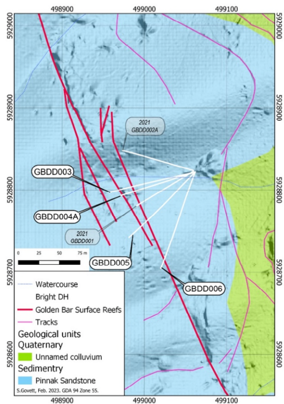
Figure 1 Golden Bar Prospect drilled holes over LiDAR plan with traced tracks and surface expressions of controlling reef structures.
