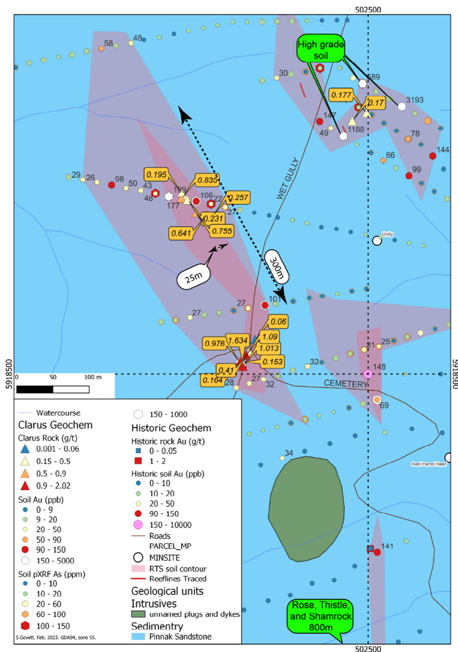
Figure 10; broad shear zone related mineralisation north of Rose, Thistle, and Shamrock.
