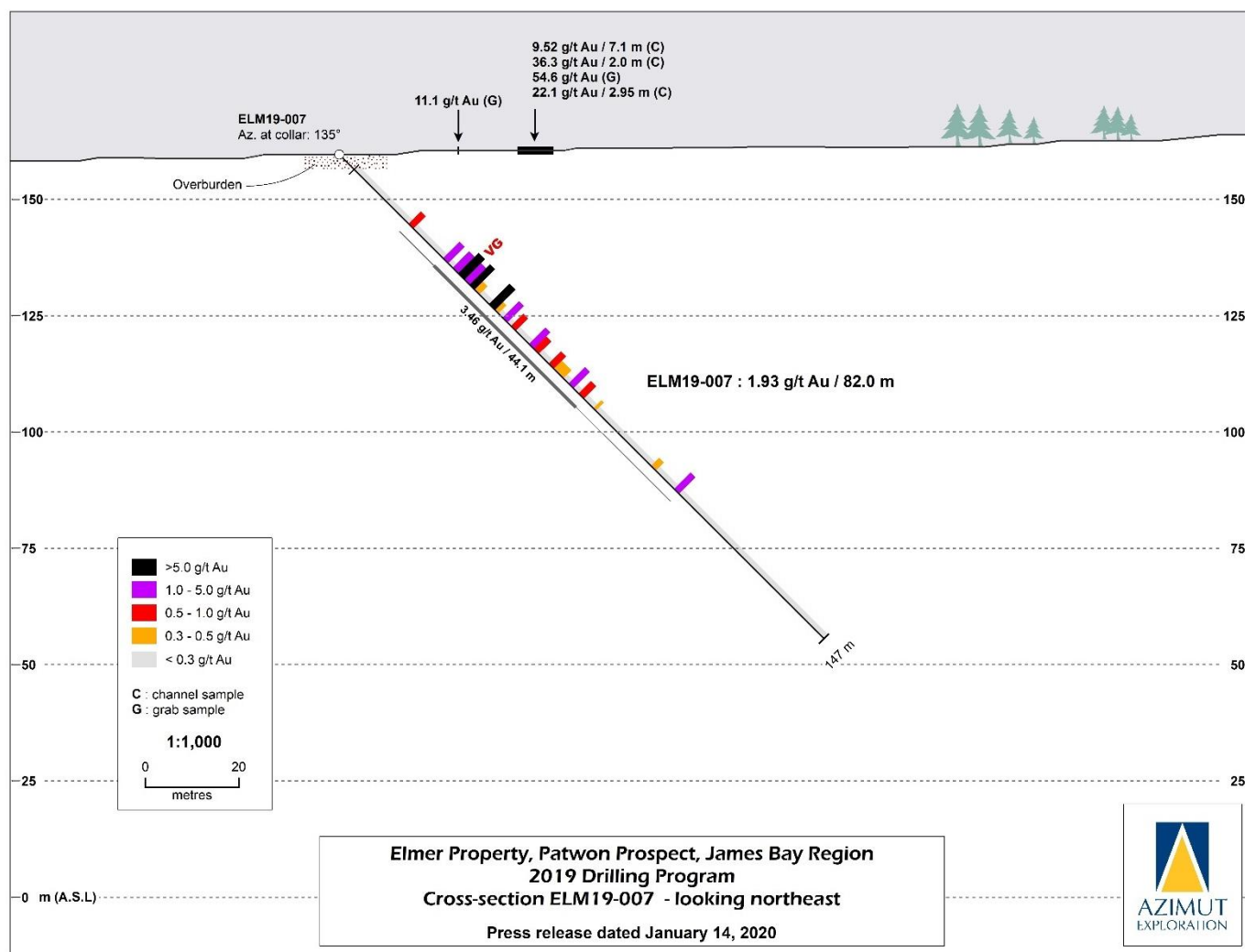
Figure 16c: Cross section of selected drill holes on the Patwon Prospect (looking northeast, ELM19-007).
