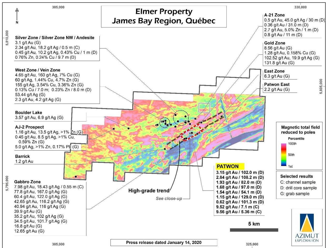
Figure 14: Magnetic map of the Elmer Property showing salient historical and recent exploration results and the location of the main gold trend (grey dashed outline) and the target area of the 2019 drilling program (red dashed outline).
