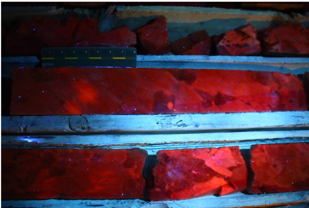
Photo 3: Very coarse white spodumene crystals in Hole GAL24-020 (this picture: from 126.5 m to 127.7m). UV light. Spodumene crystals appear in red.
