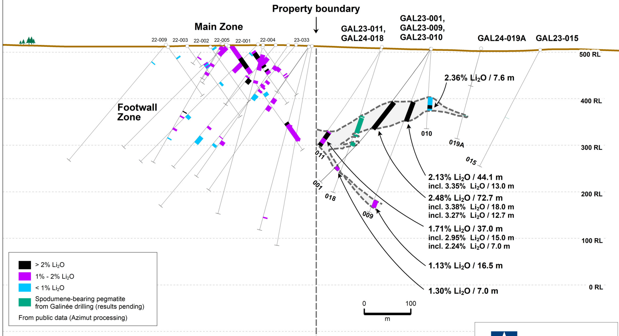
Galinée - Adina Area, James Bay Region Cross-section L535E looking East (50 m corridor of influence) Holes GAL23-001, 009, 010, 011, 015, GAL24-018 and 019A
