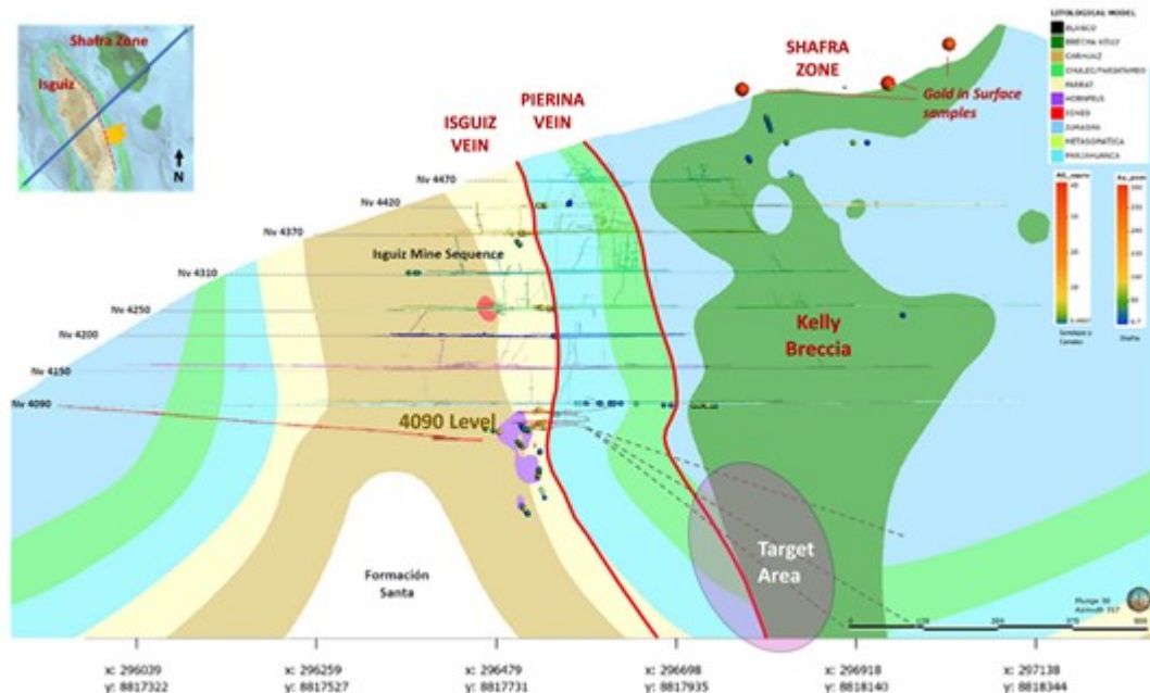
Figure 5: Shafra Exploration, Longitudinal Section Looking Northwest
