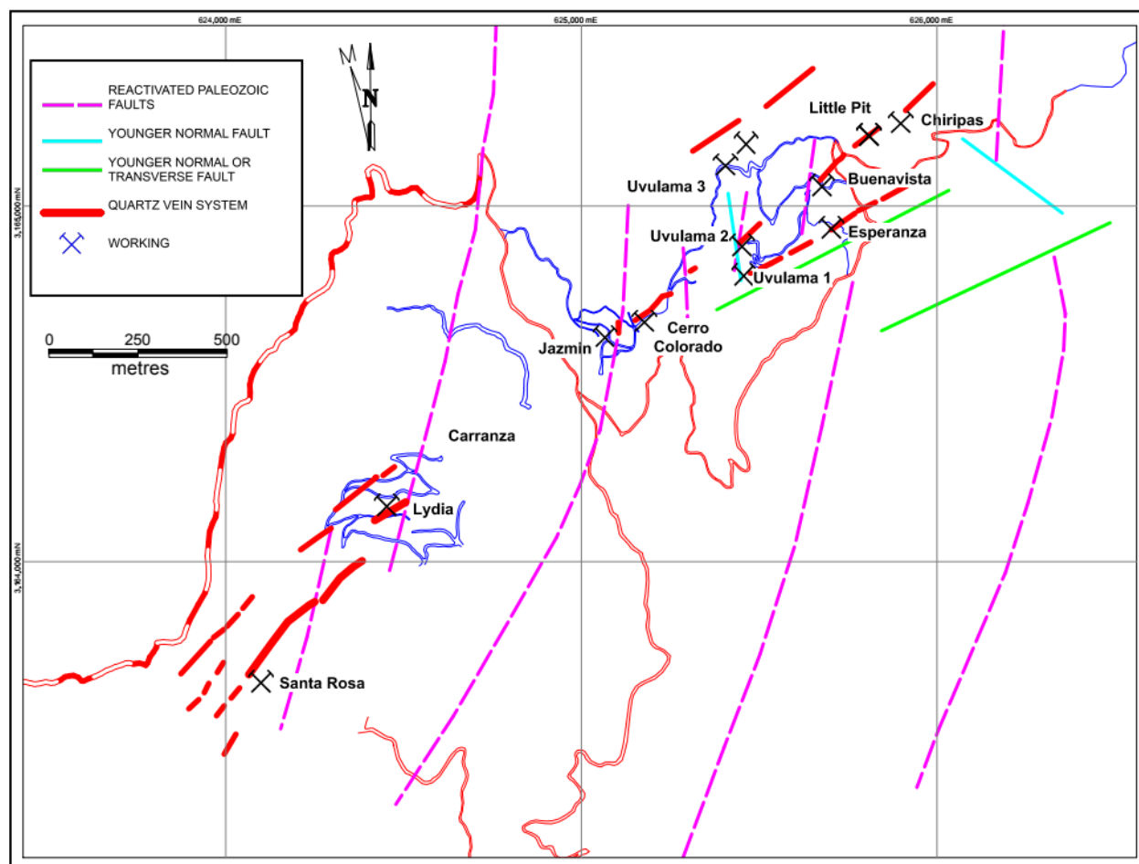
Figure 1. Schematic Plan View of Veins and Showings along the SRMC
