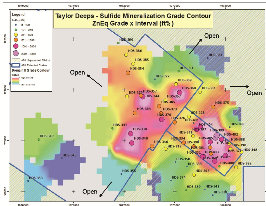
Figure 2. Taylor Deeps Mineralization Grade Contour Map
