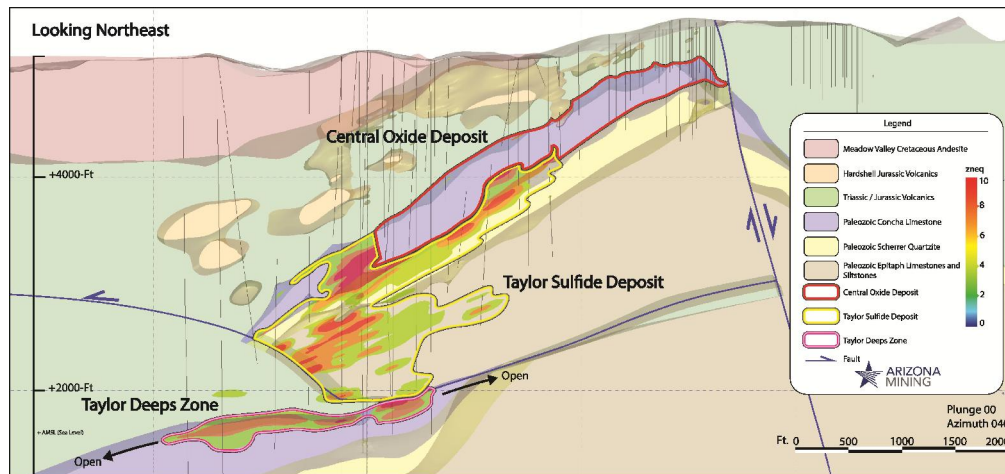
Figure 1. Longitudinal View of Oxide & Sulfide Mineralized Deposits and Taylor Deeps Zone
